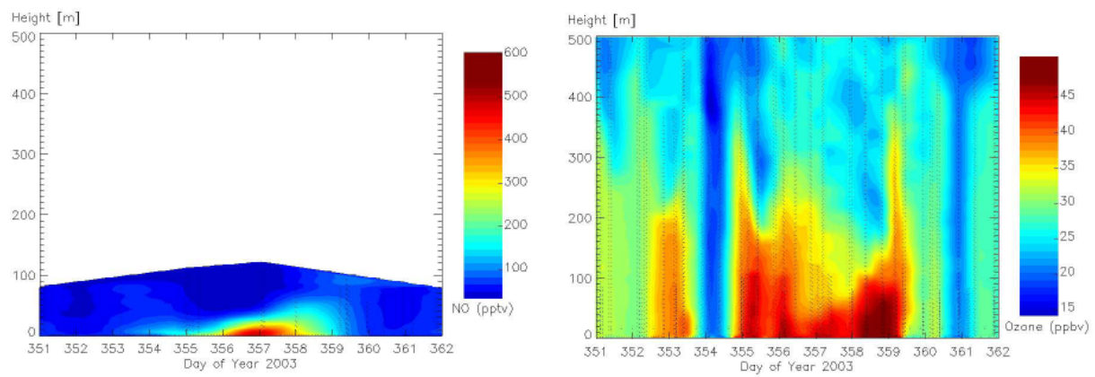
Figure 10. Comparison of the vertical distribution of NO (left) and ozone (right) during Dec. 2003 at South Pole. These data are from concurrent vertical profile measurements of NO and ozone using a tethered balloon. (Figures adapted from Helmig et al., 2007a, 2007 9 ).
