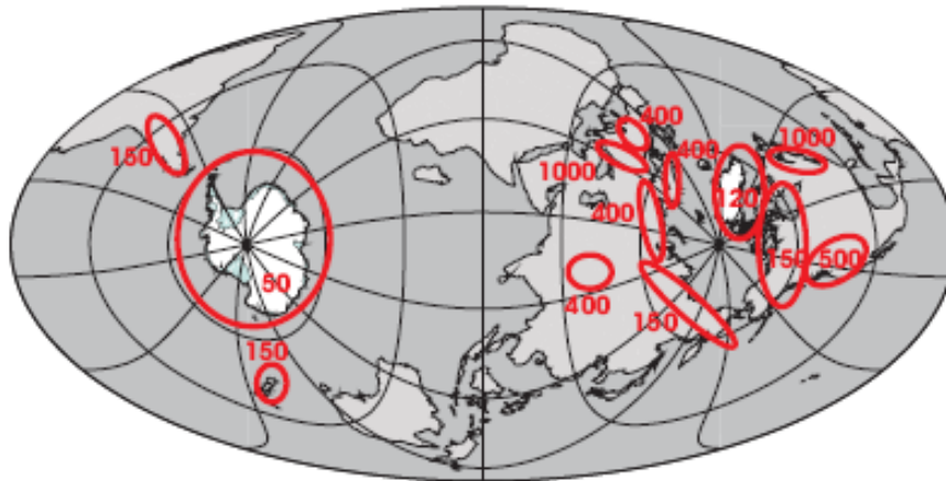
Figure 7. Estimates of snow nitrate concentrations ( \mu\text{g kg}^{-1} ) for different snow-covered regions. See original references for details. Antarctica and sea ice zone (Mulvaney and Wolff, 1994) (much higher values may be found in the very surface layer in central Antarctic (Röthlisberger et al., 2000) and in coastal regions, where sea salt and mineral aerosols efficiently scavenge nitric acid (Beine et al., 2006)); Greenland and adjacent Arctic islands (Röthlisberger et al, 2002; Koerner et al., 1999); North America: maps at National Atmospheric Deposition Program (NADP) ( http://nadp.sws.uiuc.edu/isopleths/annualmaps.asp ); Alps (summer concentrations) (Preunkert et al., 2003); rest of Europe: EMEP ( http://www.nilu.no/projects/ccc/emepdata.html ); Himalayas (Hou et al., 1999); other regions by analogy. The uncertainty on these values due to extrapolation from specific sites is at the very least a factor 2, and this range has to be explored in sensitivity studies.
