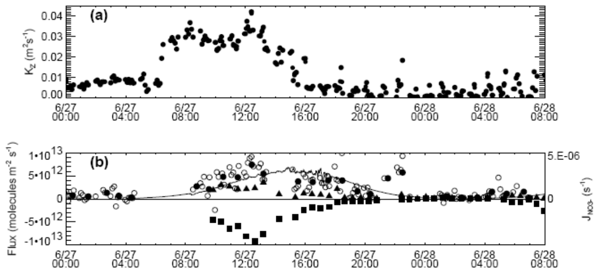
Figure 4. a) Eddy diffusivity measurements and (b) calculated fluxes (flux-gradient approach) during 27-28 June at Summit, Greenland. circles = \text{NO}_x , triangles = \text{HONO} , squares = \text{HNO}_3 , solid line = J(\text{NO}_3^-) . Positive values indicate an upward flux. (Reprinted from Honrath et al., Vertical fluxes of \text{NO}_x , \text{HONO} and \text{HNO}_3 above the snowpack at Summit, Greenland, Atmospheric Environment , 36, 2629 - 2640, 2002, with permission from Elsevier).
