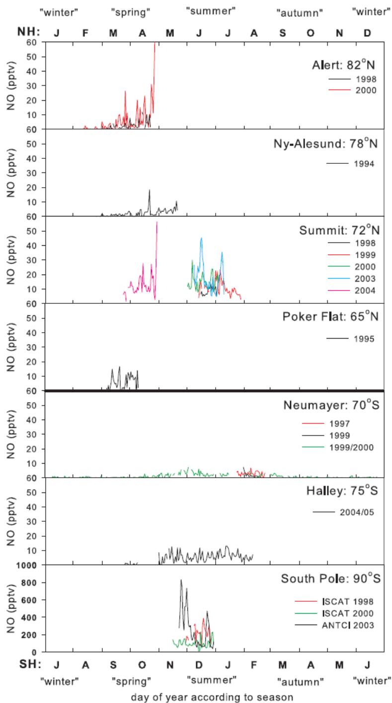
Figure 5a. Overview of recent NO measurements from high latitude sites.
