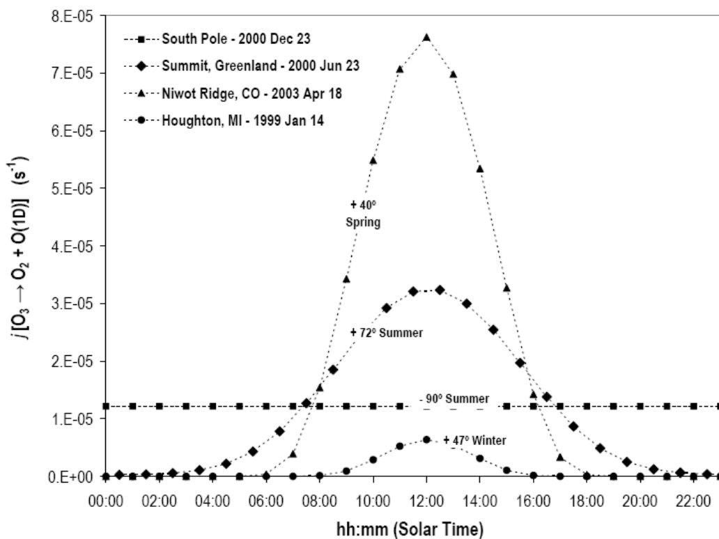
Figure 1. Cloud-free J[\text{O}_3 + hv \rightarrow \text{O}_2 + \text{O}(^1\text{D})] from TUV (Tropospheric Ultraviolet and Visible) radiation model for various latitudes and seasons at selected sites where snow photochemistry measurements have been made. Data shown for: South Pole ( 90^\circ\text{S} , 23-December, 2000); Niwot Ridge, Colorado, USA ( 40^\circ\text{N} , 18-April, 2003); Houghton, Michigan, USA ( 47^\circ\text{N} , 14-January, 1999); and Summit, Greenland ( 74^\circ\text{N} , 23-June, 2000).
