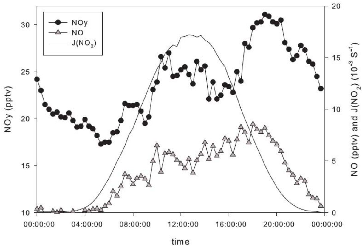
Figure 6. Diurnal variation in NO y , NO and J-NO 2 measured at Neumayer Station, Antarctica, 1997, (Weller et al., 1999).
