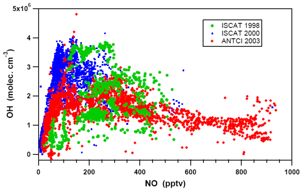
Figure 8. OH versus NO at South Pole.
