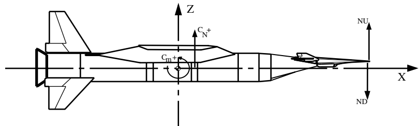
Fig. 6 Coordinate system of the 3%-scale Hyper-X launch vehicle stack model.
