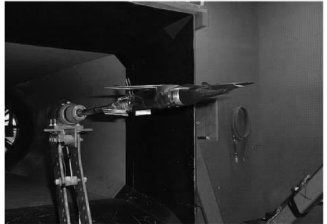
Fig. 2 The 3%-scale Hyper-X launch vehicle stack model in the ViGYAN 3 by 4 ft low-speed wind tunnel.
