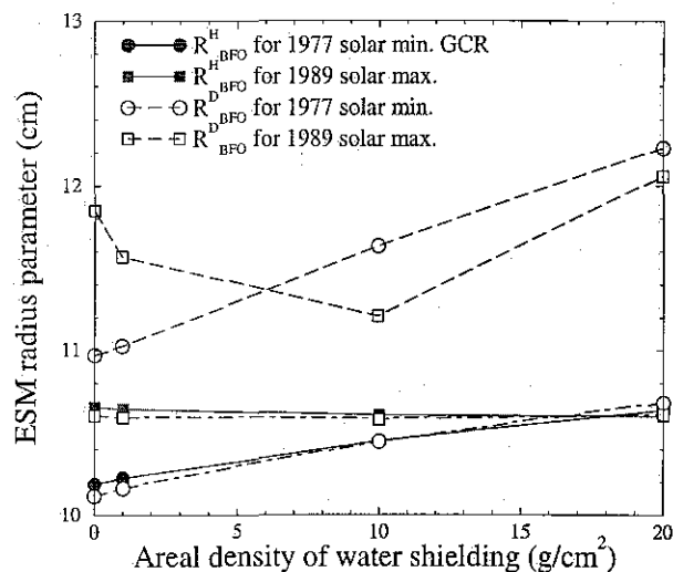
FIG. 7: The radius parameters for BFO in GCR environments as a function of the areal density of the water shielding surrounding the organ. The dot-dashed curves represent the radius parameters for the BFO dose equivalent when the ICRP26 quality factor is used.
