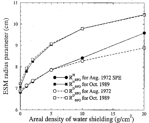
FIG. 4: The radius parameters for BFO in two SPE environments as a function of the areal density of the water shielding.
