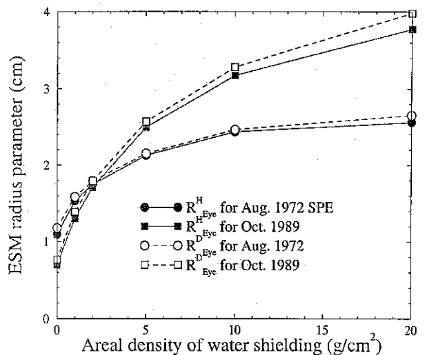
FIG. 5: The radius parameters for the eye in two SPE environments as a function of the areal density of the water shielding.
