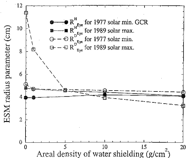
FIG. 8: The radius parameters for the eye in GCR environments as a function of the areal density of the water shielding.
