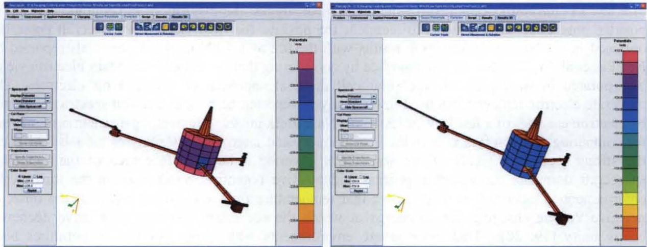
Figure 6 - Nascap-2k low speed solar wind environment potential results using the (a) interplanetary and (b) geosynchronous computation option.
