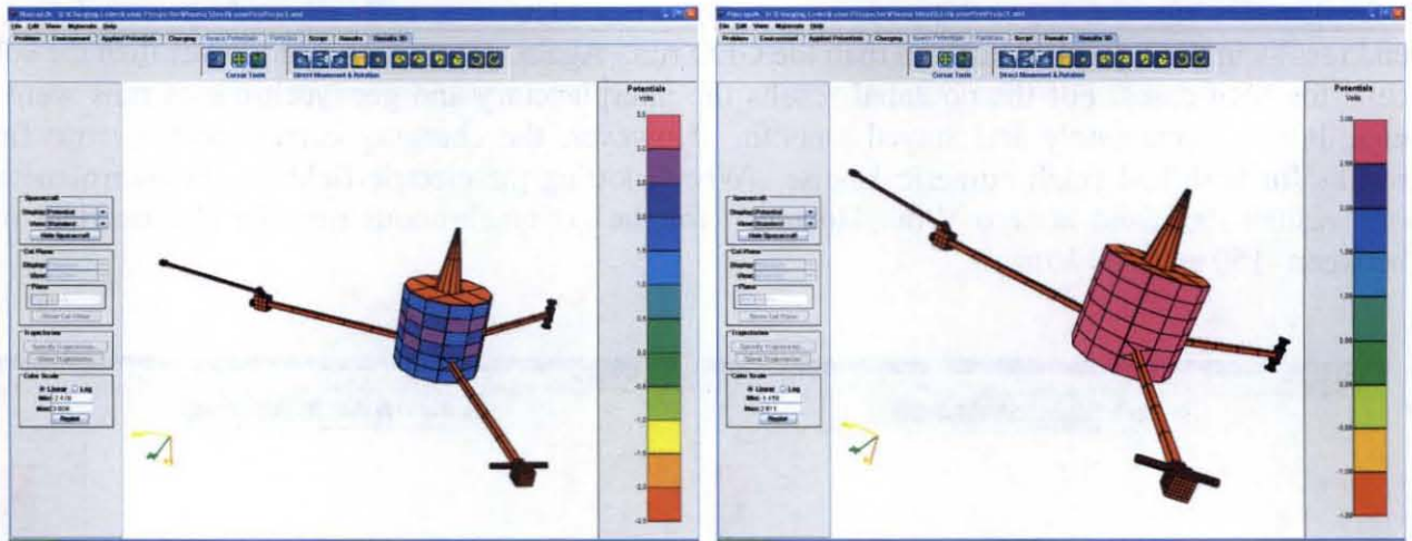
a. b. Figure 4 - Nascap-2k plasmashet environment potential results using the (a) interplanetary and (b) geosynchronous computation option.
