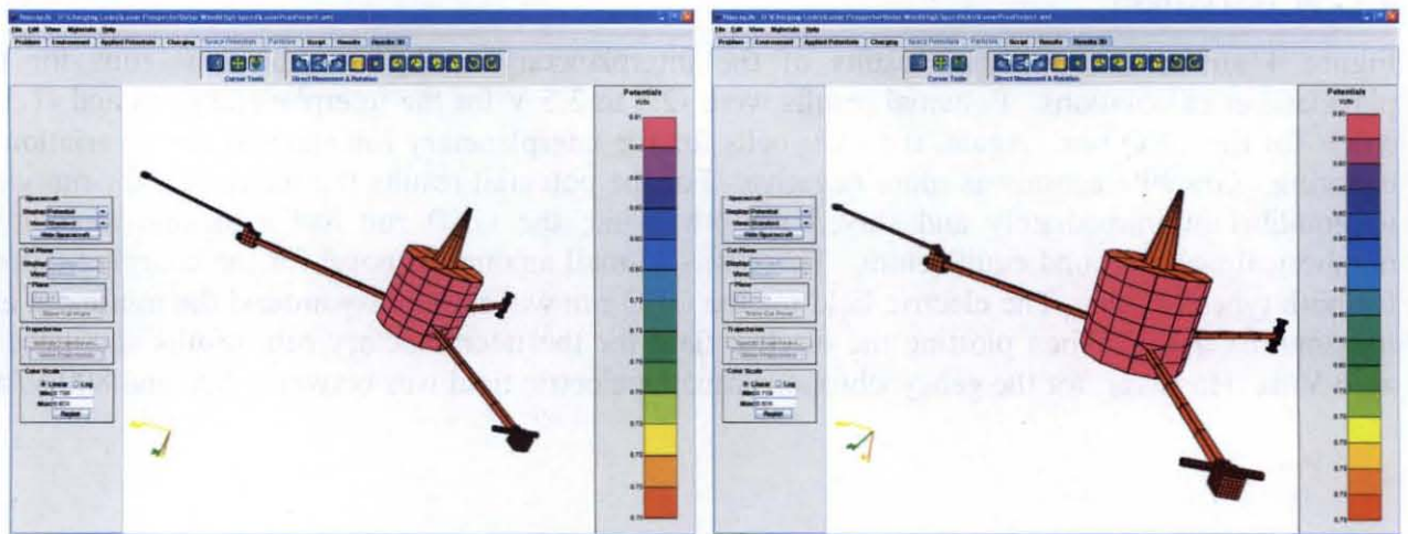
a. b. Figure 5 - Nascap-2k high speed solar wind environment potential results using the (a) interplanetary and (b) geosynchronous computation option.
