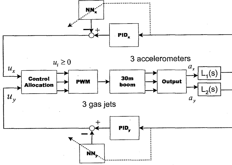
Figure 3: Control Architecture
