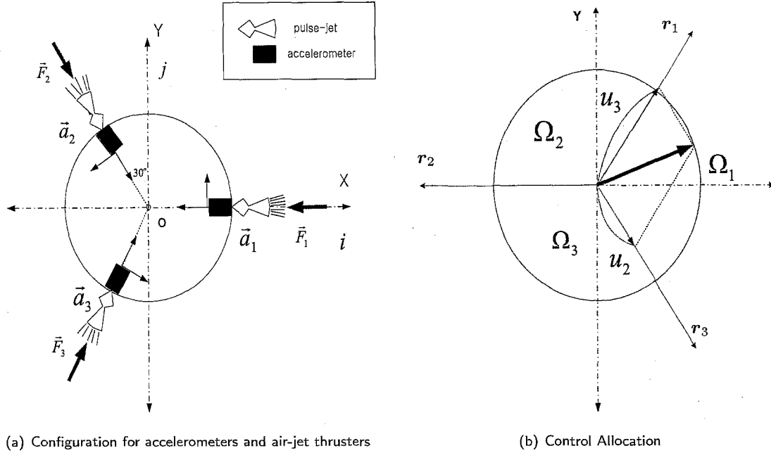
Figure 4: Outputs and Control Allocation
