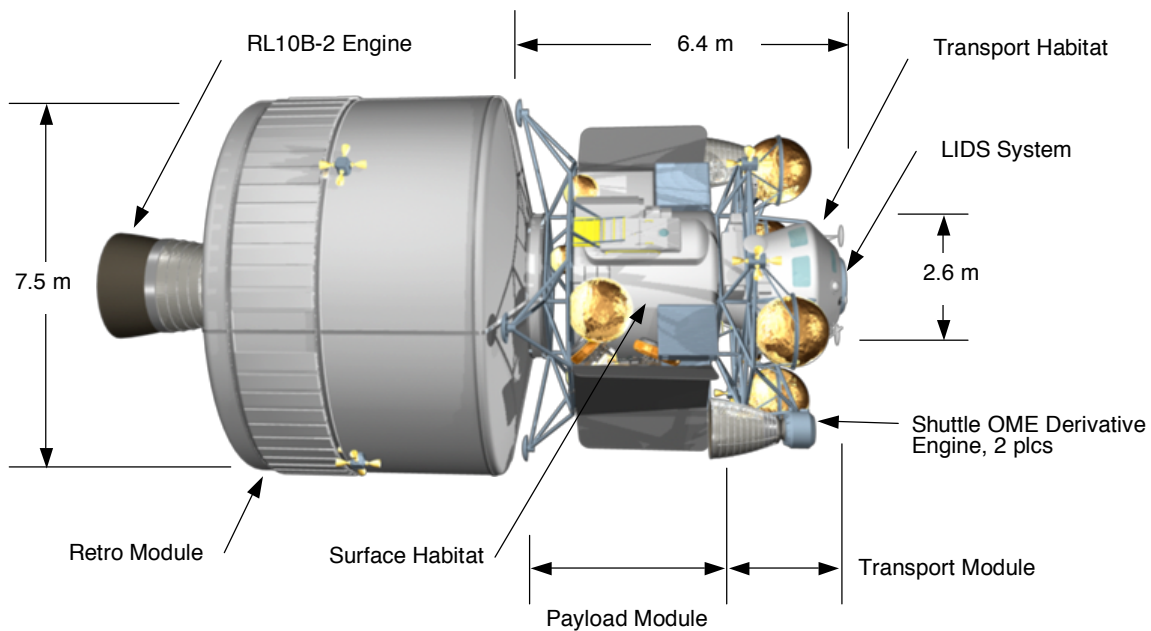
Figure 3. Descent Assisted, Split Habitat Lander.
