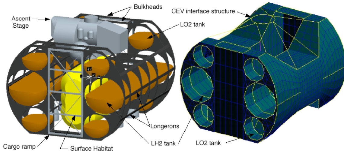
Figure 8. Horizontal Lander structural components.
