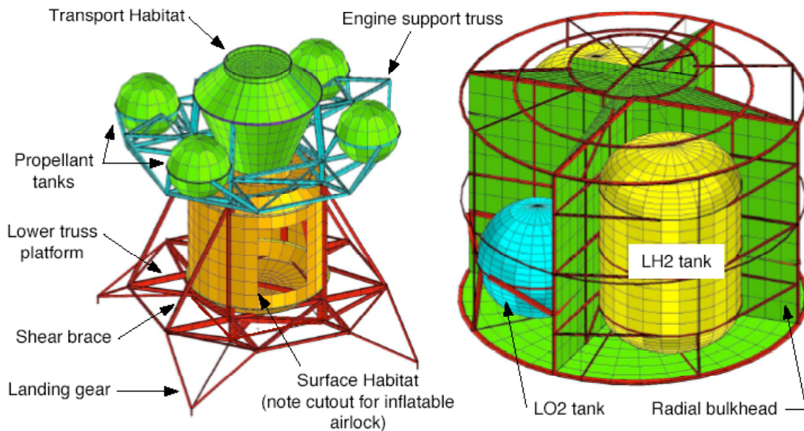
Figure 6. DASH Lander structural components.
