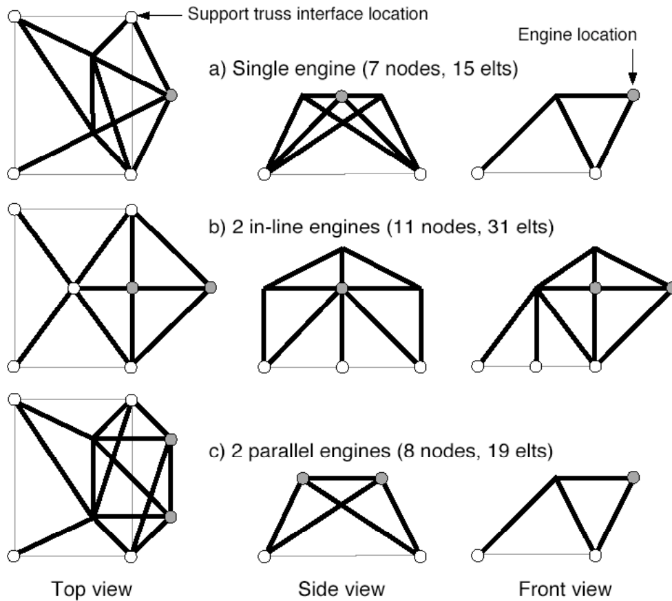
Figure 7. DASH engine support truss concepts.
