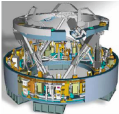
Figure 5. LIDS androgynous docking and berthing mechanism.
