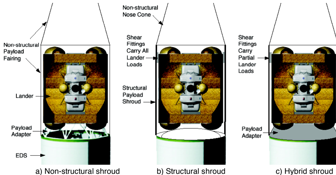
Figure 9. Payload shroud concepts.
