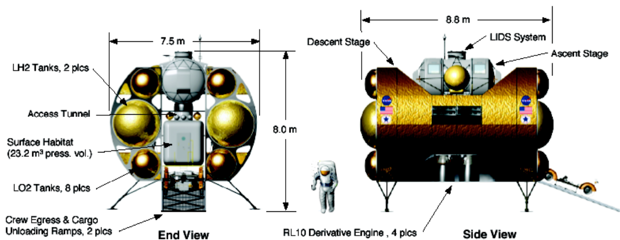
Figure 4. Cargo Star Horizontal Lander overview.
