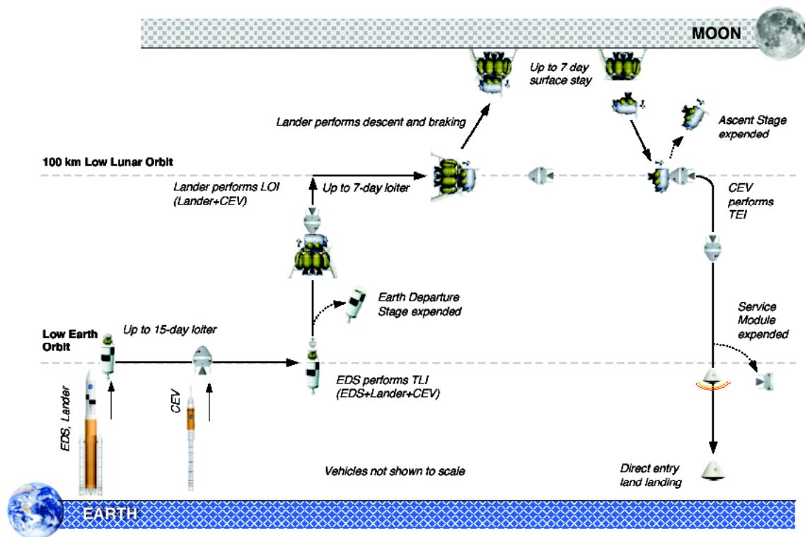
Figure 1. ESAS lunar design reference mission.
