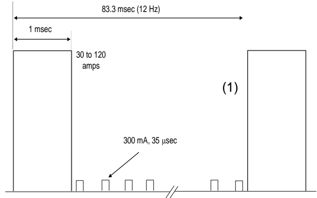
Figure 2. The Forward Voltage-Short Pulse technique for measuring the LDA junction temperature.
