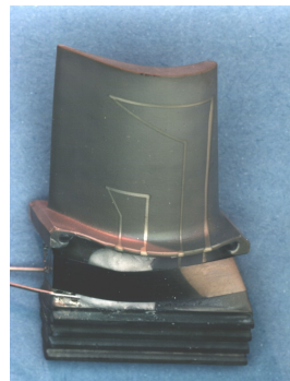
Pt- Pt/Rh temperature sensor to T=1200°C
