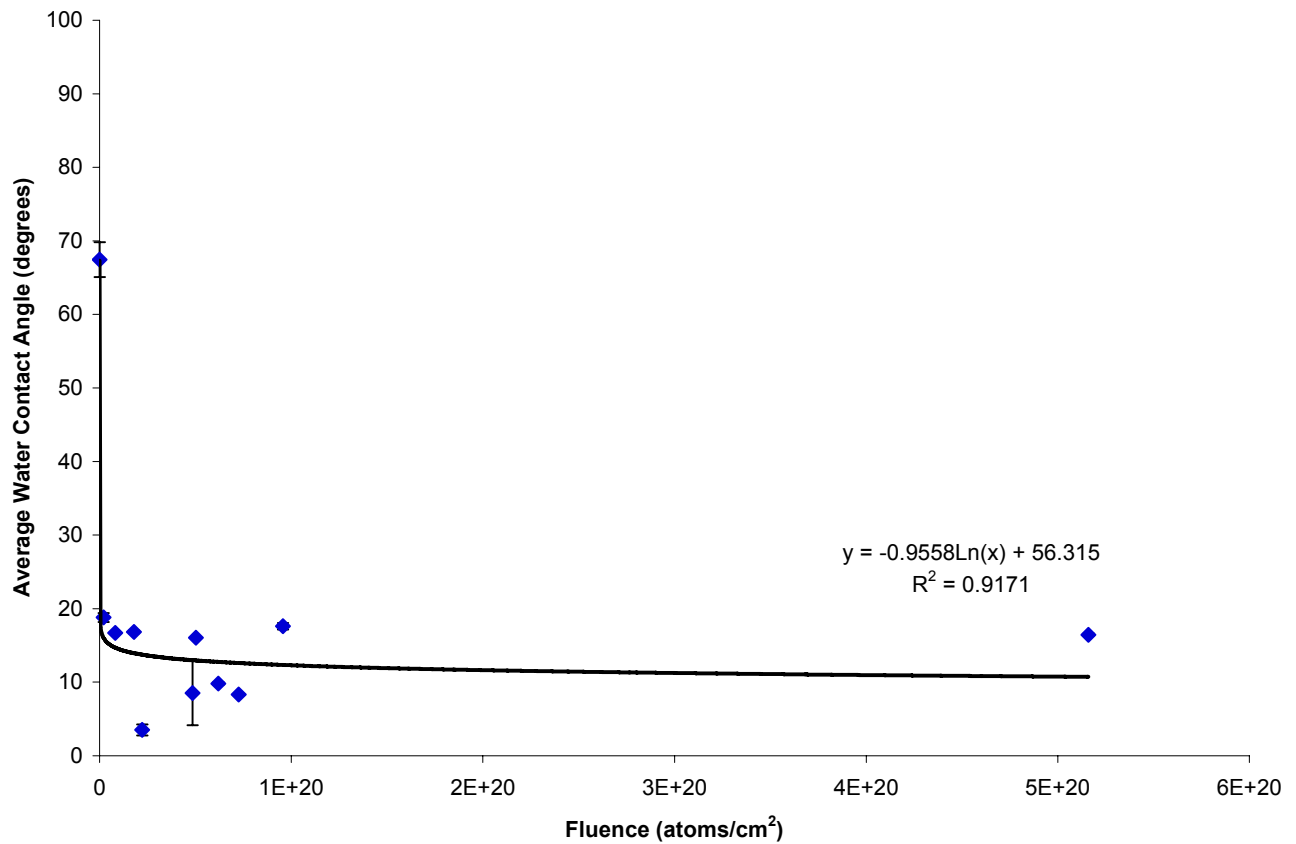
Fig. 2. Water contact angle versus atomic oxygen fluence of PET
