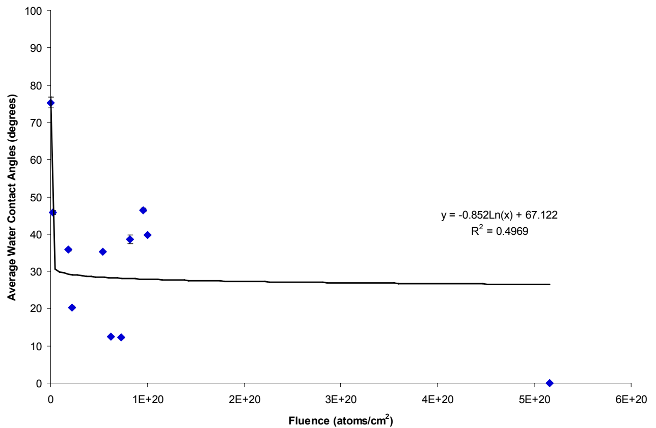
Fig. 6. Water contact angles versus atomic oxygen fluence of PMMA
