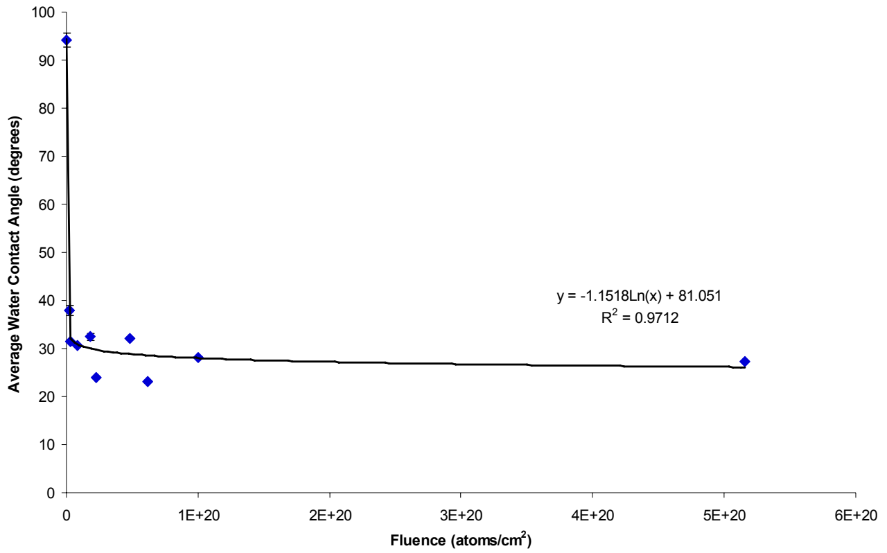
Fig. 1. Water contact angle versus atomic oxygen fluence of PE
