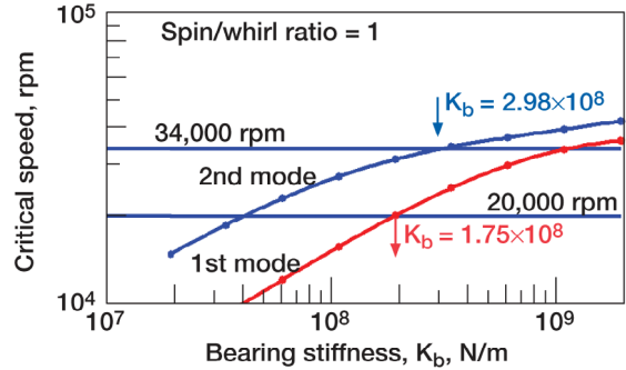
Fig. 15. Critical speed map of seal test rotor with Linear bearings.
