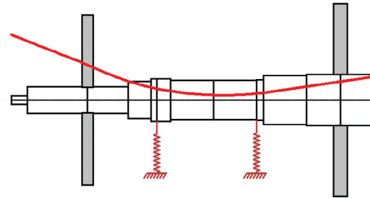
Fig. 17. Second mode shape at 31,291 rpm with K_b = 175 \text{ MN/m} .
