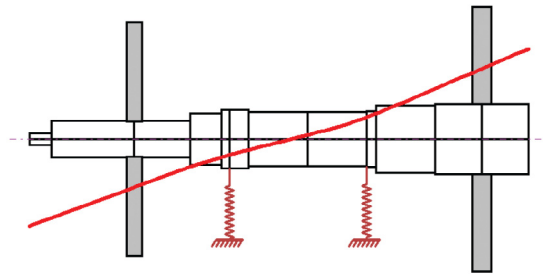
Fig. 16. First mode shape at 20,088 rpm with K_b = 175 \text{ MN/m} .
