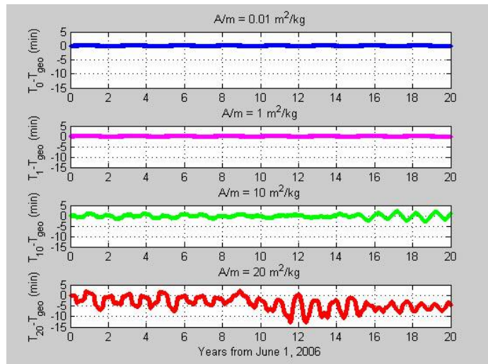
Figure 1 Deviation from GEO Period 20-year Histories for A/m = .01, 1, 10 and 20 m^2/kg
