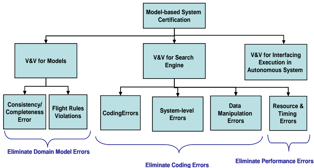
Figure 3.1 - Property decomposition for model-based software.
