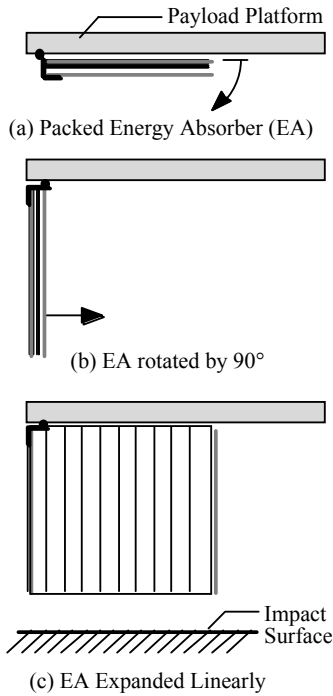
Fig. 3. Basic steps required for linear deployment of a packed energy absorber. Deployment mechanisms could include springs or actuators of various kinds.
