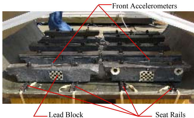
Fig. 32. Close-up photograph of fuselage floor showing instrumentation position, the seat rails and lead blocks.
