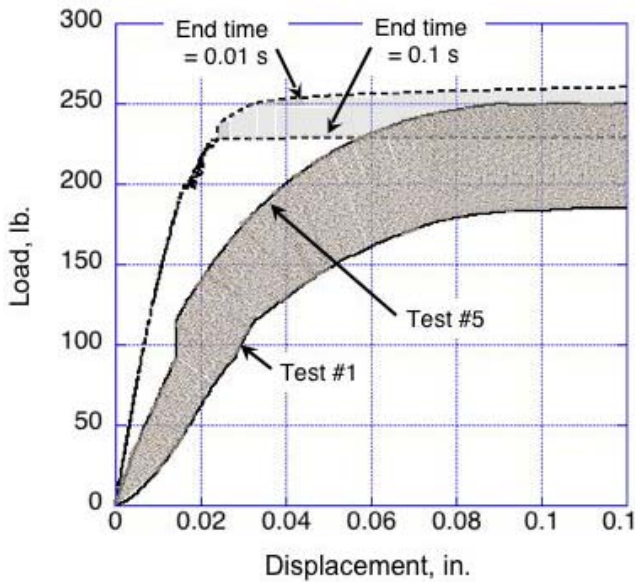
Fig. 30. Test/analysis correlation for three-point-bend test ( W=0.75'' , t=0.01'' ).
