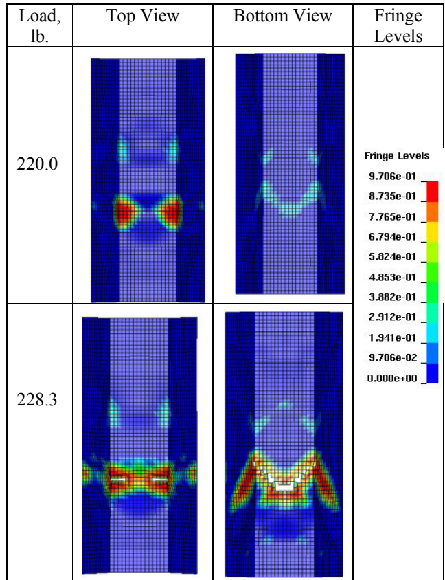
Fig. 31. Fringe plots of history variable #3.
