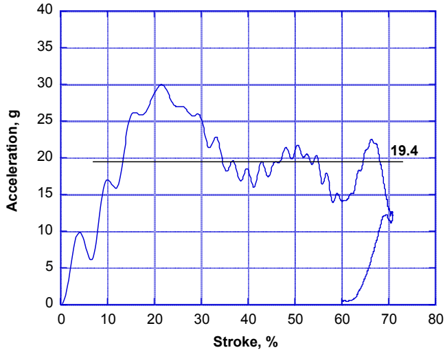
Fig. 23. Typical acceleration/stroke response from the vertical fuselage test: – center left accelerometer.
