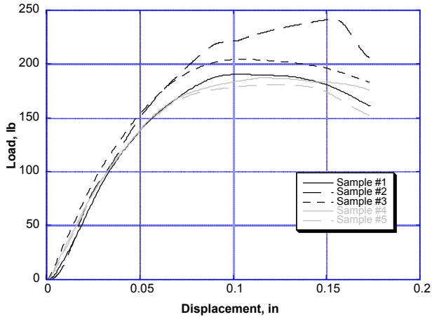
Fig. 19. Load displacement response from 3-point-tests on samples with t=0.010'' , and W= 1.0'' .
