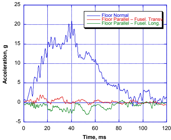
Fig. 26. Acceleration/time response for oblique fuselage-section drop. The three orthogonal accelerometers were mounted at the center of the floor.
