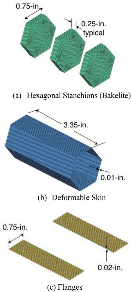
Fig. 28. Three distinct parts of the LS-DYNA model.
