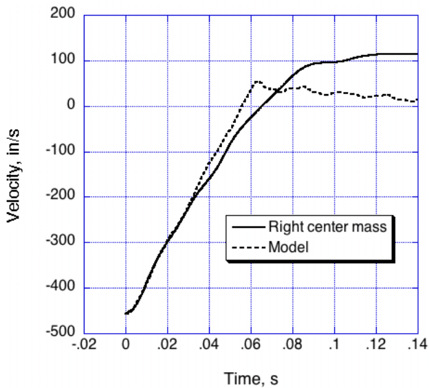
Fig. 37. Velocity time history comparison between analysis and experiment.
