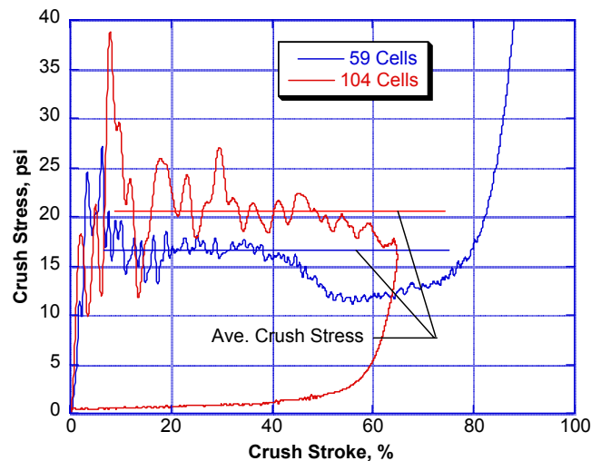
Fig. 14 Dynamic crush response of deployable honeycomb samples with similar cell geometry. Both samples were made of a single woven layer of Kevlar-129.
