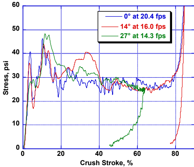
Fig. 16. Effect of cell-axis orientation on the crush response of spectra/glass hybrid deployable honeycombs. All samples had the same cell-wall thickness and width.
