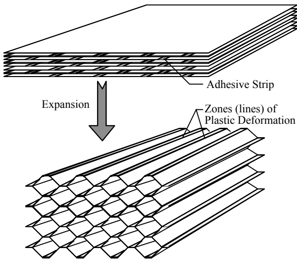
Fig. 7. Schematic of typical fabrication method used in the production of conventional honeycombs.
