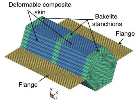
Fig. 27. LS-DYNA single cell model for 3-point-bend test.
