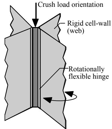
Fig. 1. Schematic of the junction (hinge) of a square cell deployable structure.
