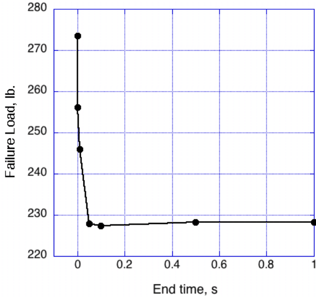
Fig. 29. Failure load versus end time for three-point-bend test.
