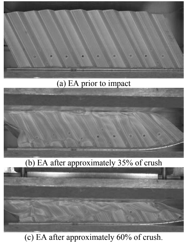
Fig. 17. High speed video frames from 27° off axis test.
