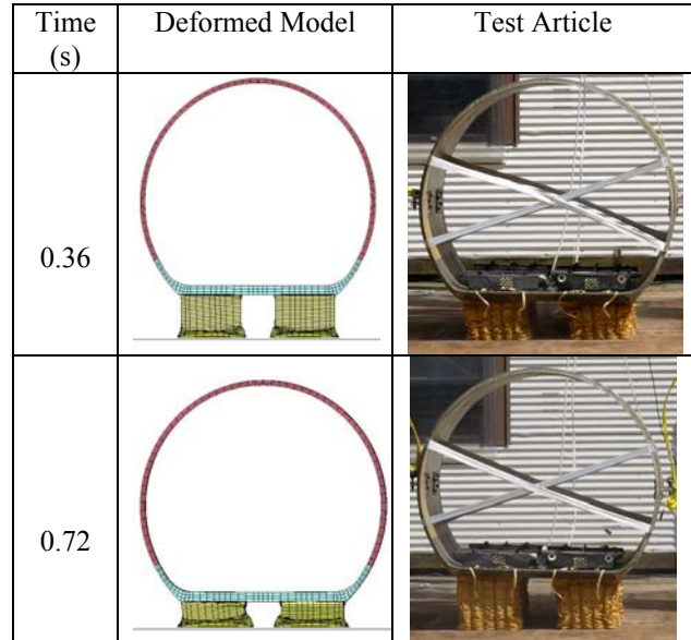
Fig. 35. Analysis and test comparisons of EA crush.
