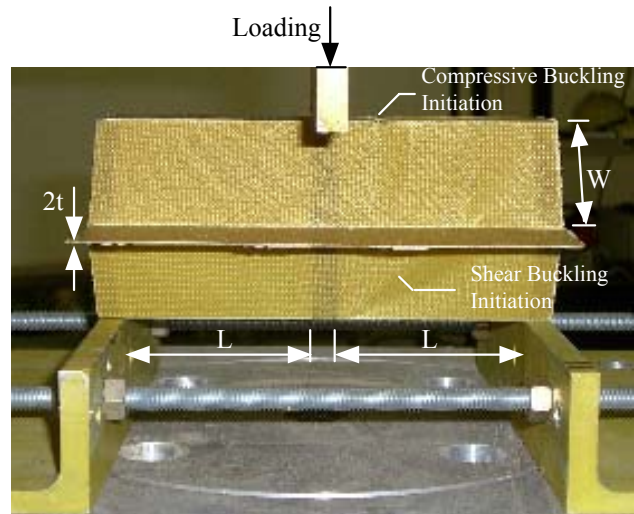
Fig. 18. Three-point-bend set-up for single cell tests. For the sample shown, W=1.5'' and t=0.010'' . The flange thickness was 2t .
