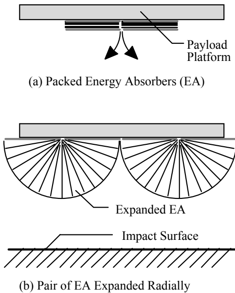
Fig. 4. Radial deployment of two energy absorbers. EA shape can be spherical, cylindrical, or any desired cross section. Note that deployment greater than 180° is possible if more vehicle coverage is required.
