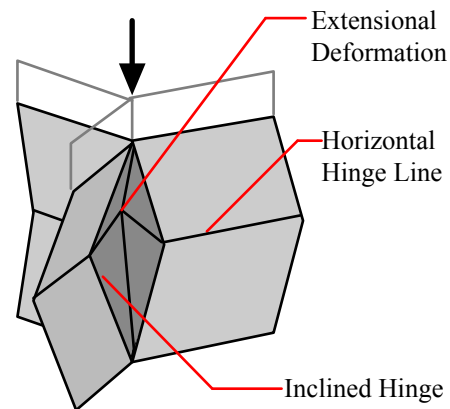
Fig. 11. Energy absorbing deformation modes for "Y" element of conventional honeycomb.
