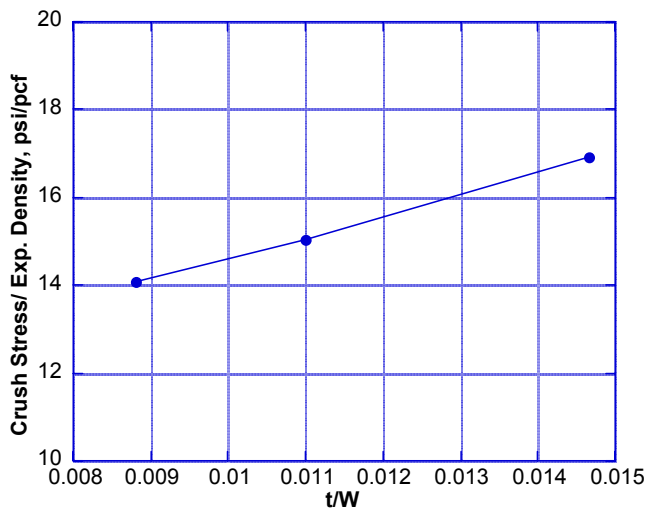
Fig. 15. Relationship between experimentally measured specific crush strength and t/W . All three values represent dynamic data at approximately 20 fps impact velocity.
