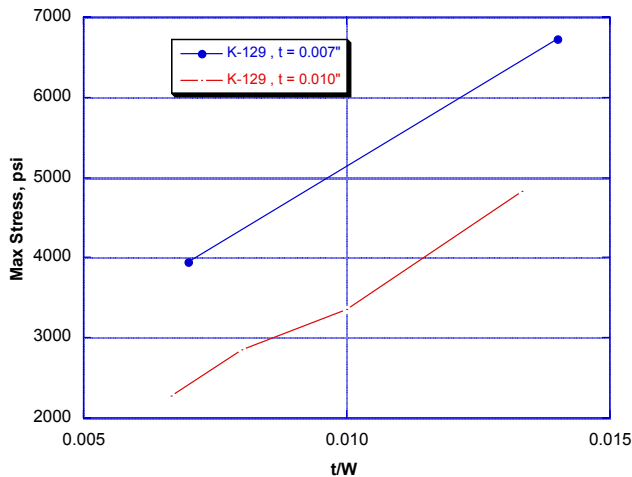
Fig. 20. Peak stress as a function of t/W for hexagonal cells made of two Kevlar 129 fabrics ( t=0.01'' and 0.007'' ).
