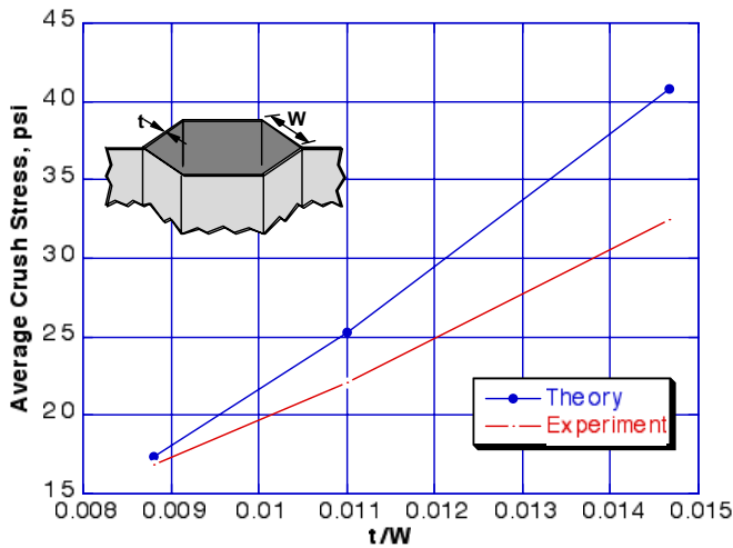
Fig. 12. Average sustained crush stress versus t/W . Theoretical points were derived using the relationship of stress versus t/W , as described in reference [15].
