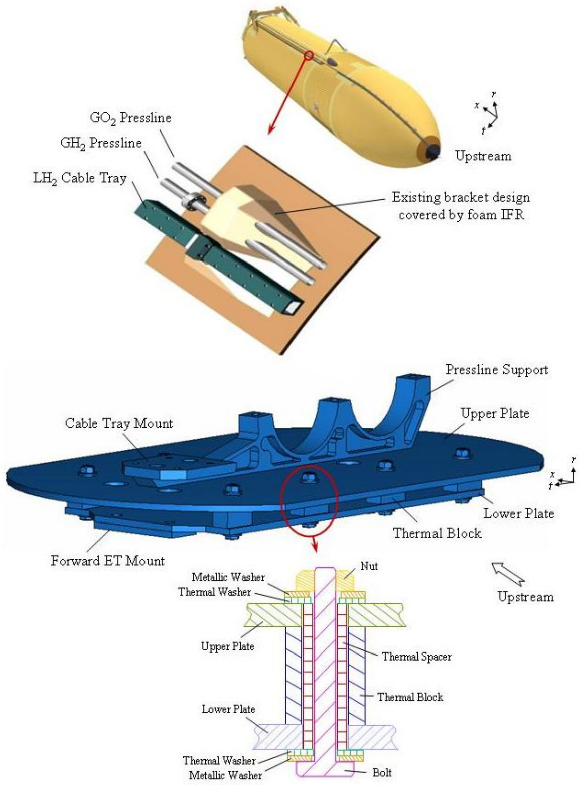
Figure 2: Proposed LH 2 IFR bracket design.
