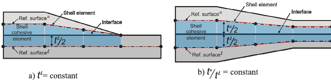
Figure 5. Special configurations with constant thickness properties.
