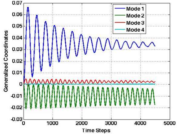
Fig. 10 Combined ROM static and dynamic aeroelastic solutions for the RSM configuration at 0.7 Mach number, 3 degrees angle of attack, and 0.1 psi dynamic pressure.
