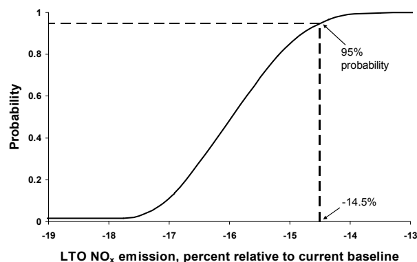
Figure 10: Cumulative distribution function of LTO NO x emission – from Propulsion-21 technologies.
