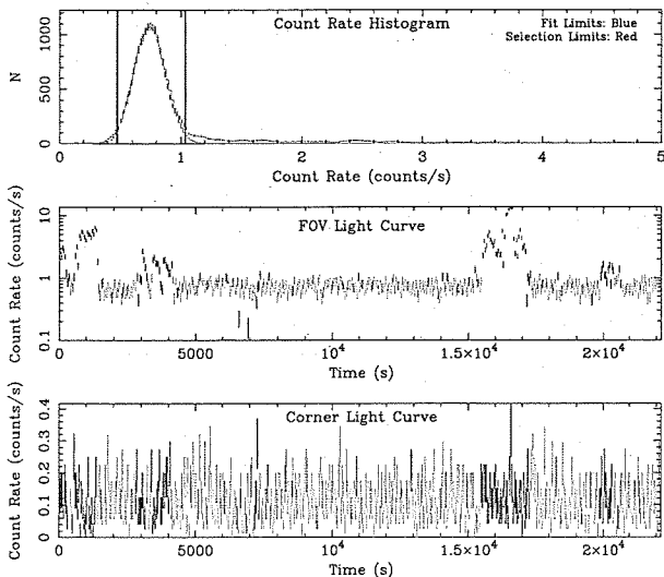
Fig. 1.— Top: A histogram of the count rate in the 2.5-8.5 keV band over the entire FOV. The blue curve is a Gaussian fitted to the histogram between the two vertical lines. The peak of the Gaussian defines the quiescent count rate, which will be composed of counts from the object and the quiescent particle background. Parts of the observation falling above 2.5\sigma above this mean quiescent rate are deemed to be contaminated by the soft proton flares. Middle: Light curve in the 2.5-8.5 keV band for the FOV smoothed with a 50 second boxcar function. The green parts of the curve are those accepted as “flare-free”. Bottom: Light curve in the same energy for the unexposed pixels. Note that the flares are not seen in the unexposed-region pixels, confirming their soft-proton origin.
