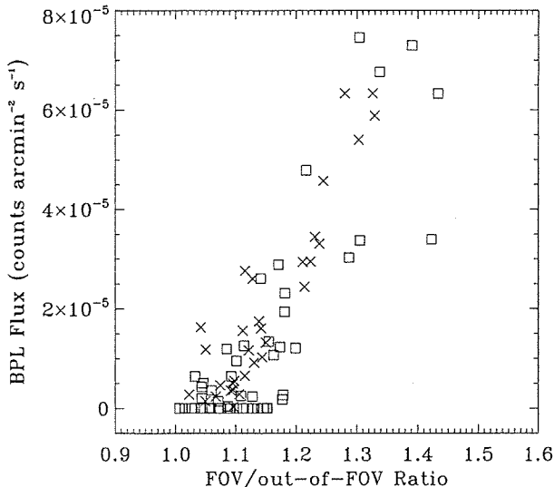
Fig. 24.— The FOV/out-of-FOV ratio in 8 < E < 12 keV compared to the amount of soft proton contamination determined by fitting the spectrum. The boxes are 78 “blank-sky” images while the crosses are for 38 cluster observations.
