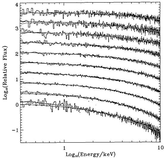
Fig. 14.— The mean flare spectra as a function of the (8.0-10.0 keV)/(0.35-1.35 keV) hardness ratio for MOS1 observing through the Medium filter. Blue: The fitting function was the sum of two exponentials where the parameters for the second exponential are quadratic functions of the parameters of first. No RMF or ARF was used in this fit. Red: The fitting function was a broken power law where all of the parameters were allowed to vary freely for all of the spectra. Only the RMF was used. Green: The fitting function was a broken power law where the break energy was set to a single value for all of the spectra. Only the RMF was used.
