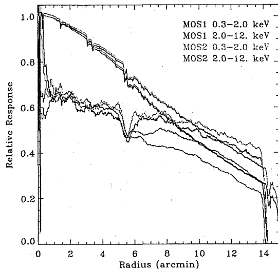
Fig. 17.— The vignetting function of the flares compared to the vignetting function of the X-rays for MOS1 observations made with the Medium filter. The upper set of curves are the vignetting function of the X-rays for both detectors and two energy bands. The X-ray vignetting functions are normalized to unity between 1' and 2' . The lower set of curves are the vignetting function of the flare images. The flare vignetting functions were normalized to unity between 2' and 3' , then shifted downwards for clarity. The flare vignetting functions show evidence of contamination by point sources for R < 1' .
