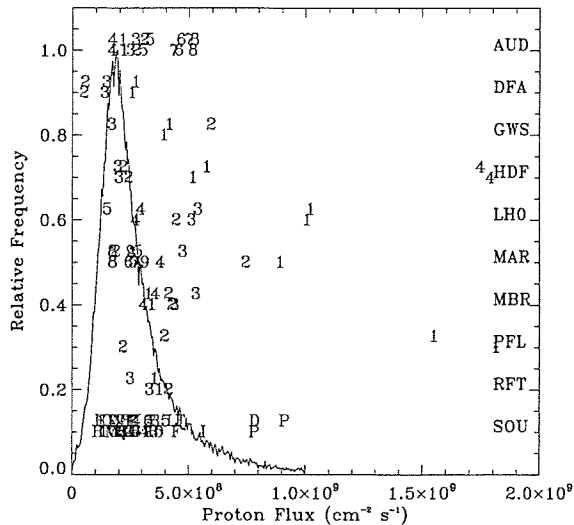
Fig. 22.— Solid Line: The relative frequency of the solar wind proton flux derived from the ACE archival data. A plot for the WIND archival data is very similar. The three letter mnemonics on the righthand side of the plot refer to the various sets of observations. Plotted at the same vertical level as the mnemonic are the values of the solar wind for each observation within that set. The set of values plotted in red slightly above the mnemonic are derived from the ACE data, while those plotted in blue slightly below the mnemonic are derived from the WIND data; not all observations have both ACE and WIND data.
