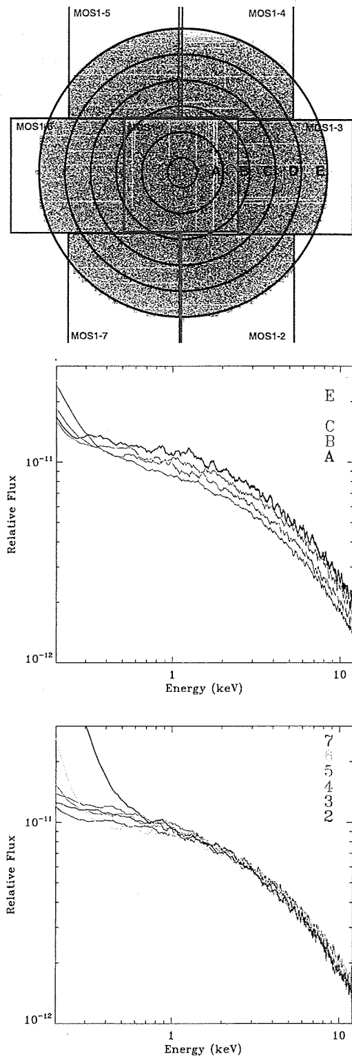
Fig. 16.— Top: Soft proton flare image for MOS1 showing the locations of the chips and the annuli used in this analysis. Middle: The flare spectrum as a function of radius. Bottom: The flare spectrum as a function of chip for the outer two annuli (D and E).
