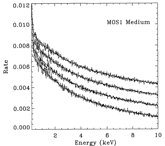
Fig. 15.— The flare spectrum for four different levels of flare strength. From the bottom, 1-2, 2-3, 3-4, and 4-5 counts/second above the quiescent level. As the flare strength increases, the mean spectrum becomes harder.
