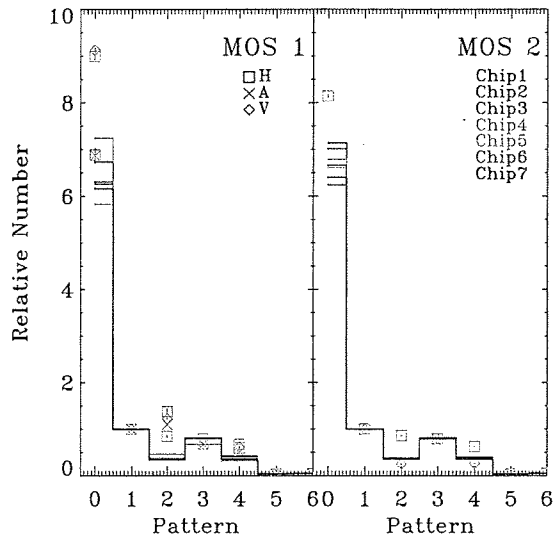
Fig. 12.— The distribution of pattern values for each state of each chip. All of the histograms have been normalized to unity for pattern 1. Normal states are shown by solid lines; anomalous states by symbols. The different chips are shown with different colors.
