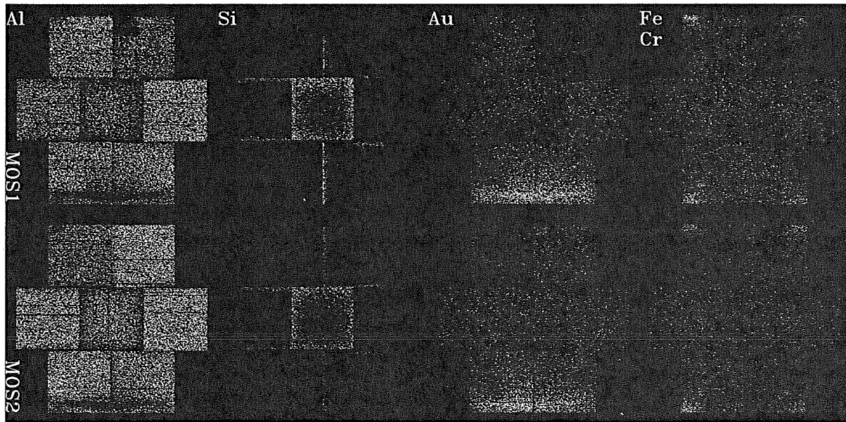
Fig. 3.— Filter-wheel-closed images in narrow energy bands including the principal lines. Top: MOS1, Bottom: MOS2. From left to right, Al 1.49 keV, Si 1.74 keV, Au 2.12, 9.71, and 11.4 keV, and Fe 6.4 keV + Cr 5.4 keV. The Fe and Cr distributions are similar so adding them together improves the visibility of the spatial distribution.
