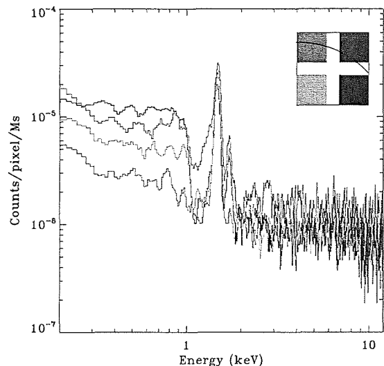
Fig. 11.— The spectrum from the four quadrants of chip MOS1-4 during the “anomalous” period. The inset shows the location of the quadrants with respect to the unexposed pixels (above the curved line).
