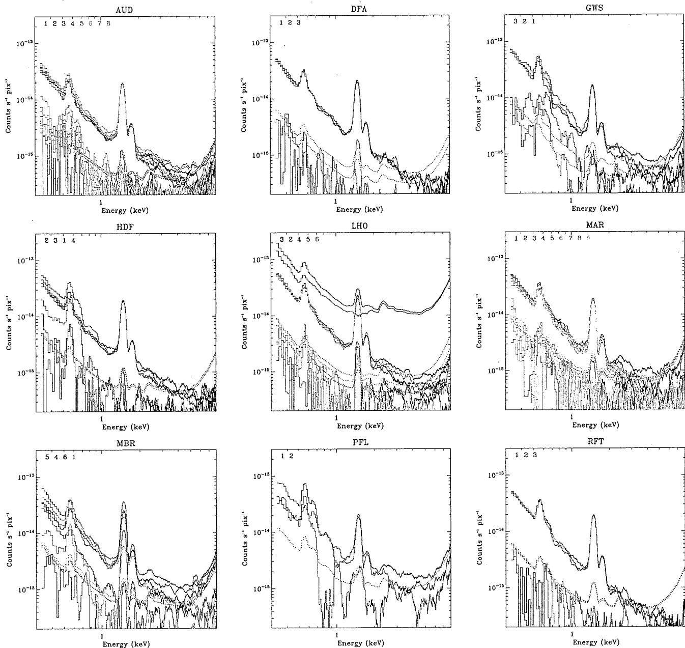
Fig. 21.— Each panel contains the all of the spectra for a single target. Of the upper set of plots (solid lines) the black spectrum is that which has the smallest O VII and O VIII flux. Each spectrum is the sum of the MOS1 and MOS2 spectrum after division by the response (arf). The lower set of solid lines shows the difference between the black spectrum and each of the other spectra. The dotted lines are the propagated uncertainties for the difference spectra.
