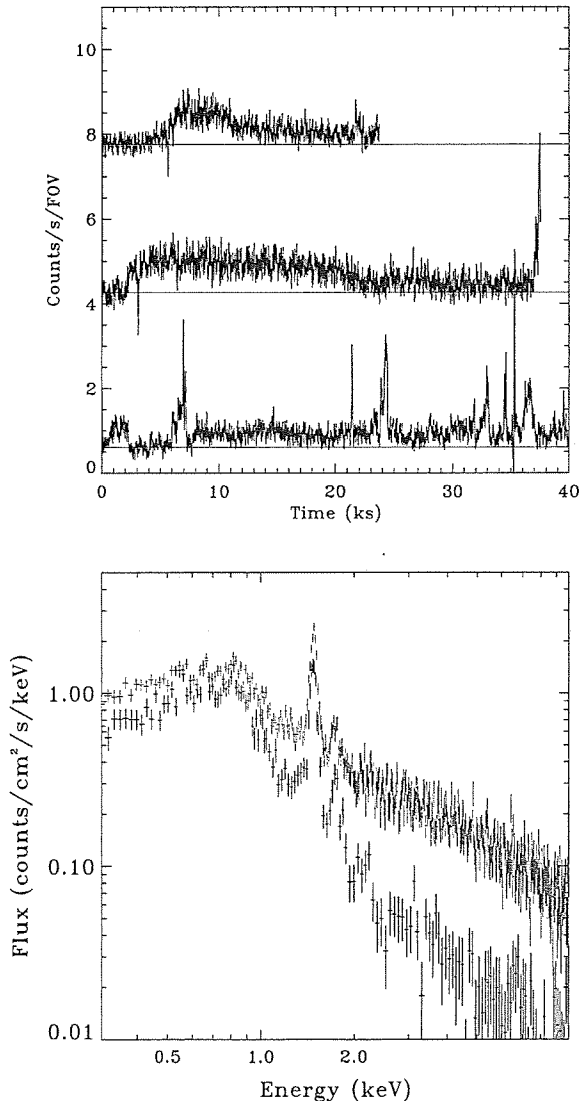
Fig. 13.— Top: Three light curves which, were the exposures much shorter, could have led to measurements of a significant overestimate of the QPB rate. Bottom: Two spectra of the same region of “blank” sky, both of were cleaned of flare intervals using the method described in §2.
