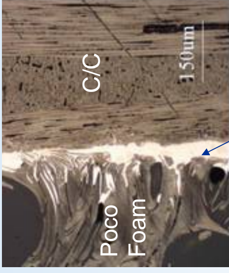
Brazed Joints
