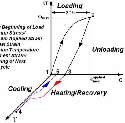
Figure 2: Schematic of an unconstrained strain recovery step test showing measurement points 1-5. Undercooling and reheating are omitted for clarity.
