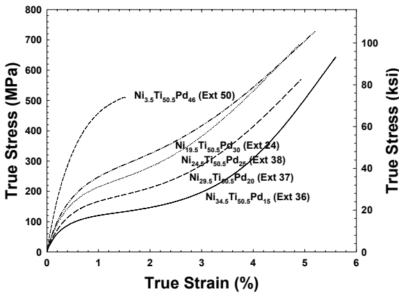
Figure 9: Monotonic tensile behavior of the alloys in the martensite state – test temperature of M_T-50^\circ\text{C} .
