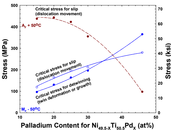
Figure 11: Critical stress data for NiTiPd alloys determined from monotonic tensile tests and strain recovery behavior.
