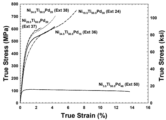
Figure 10: Monotonic tensile behavior of the alloys in the austenite state – test temperature of A_T+50^\circ\text{C} .
