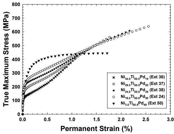
Figure 15: Permanent strain data from the five alloys.
