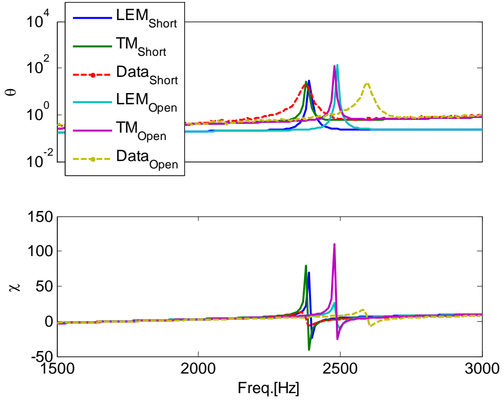
Figure 16. Comparison LEM, TR and measurement results for a short- and open-circuited EMHR (CASE I), the damping loss of the backplate is assumed to be acoustic radiation resistance
