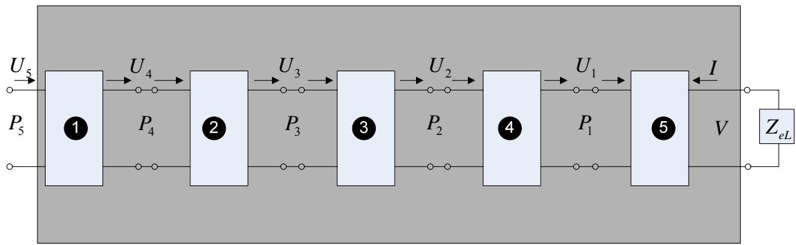
Figure 3. Illustration of the modeling EMHR using the transfer matrix method, where each subsystem is denoted as: 1-area contraction; 2-duct element; 3-area expansion; 4-duct element; 5-piezoelectric backplate.
