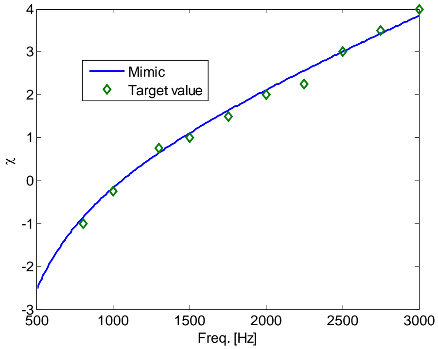
Figure E-5. Mimic behavior of the PEEK diaphragm
