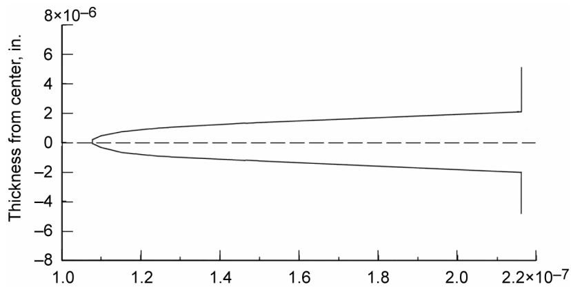
Figure 19.—Nanoscale physical variable transverse moisture diffusivity, D_{\ell 22} (in.²/hr).
