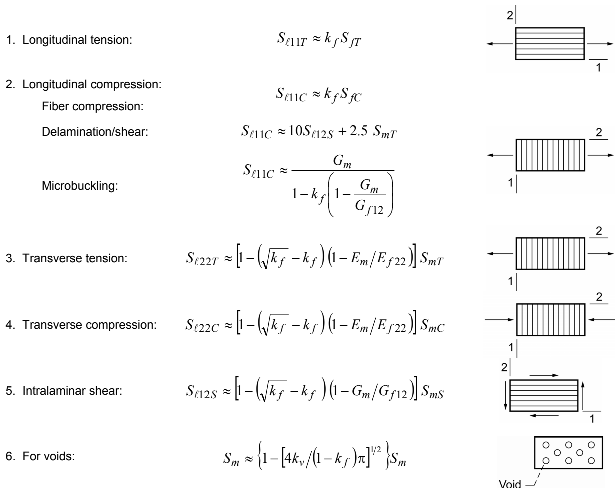
Figure 31.—Composite micromechanics, uniaxial strengths, in-plane.
