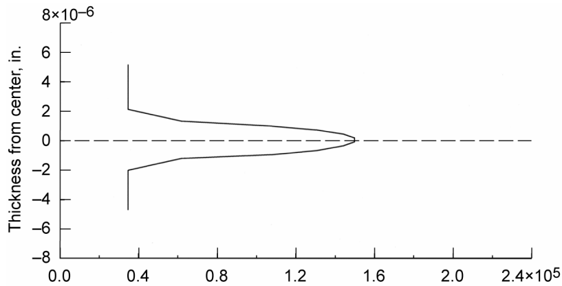
Figure 33.—Nanoscale uniaxial longitudinal compressive strength, S_{\epsilon_{11C}} (lb/in. 2 ).
