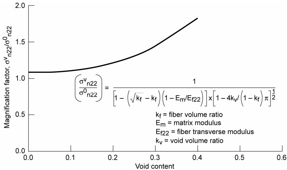
Figure 7.—Nanocomposite magnification factor.
