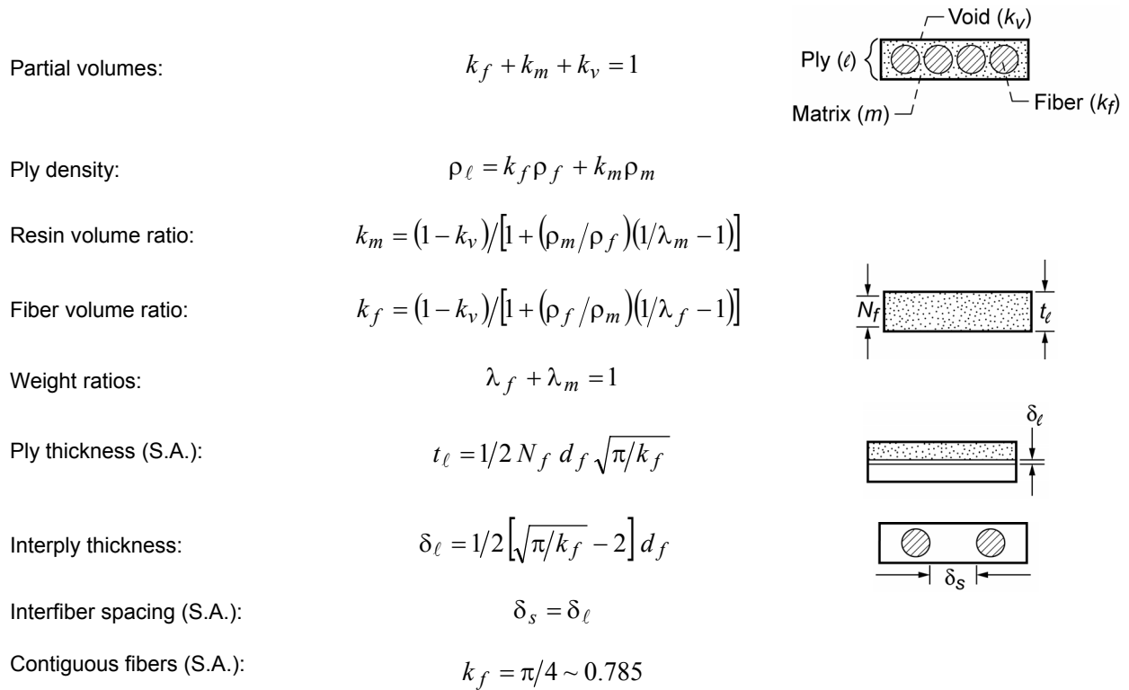
Figure 8.—Micromechanics and geometric relationships.
