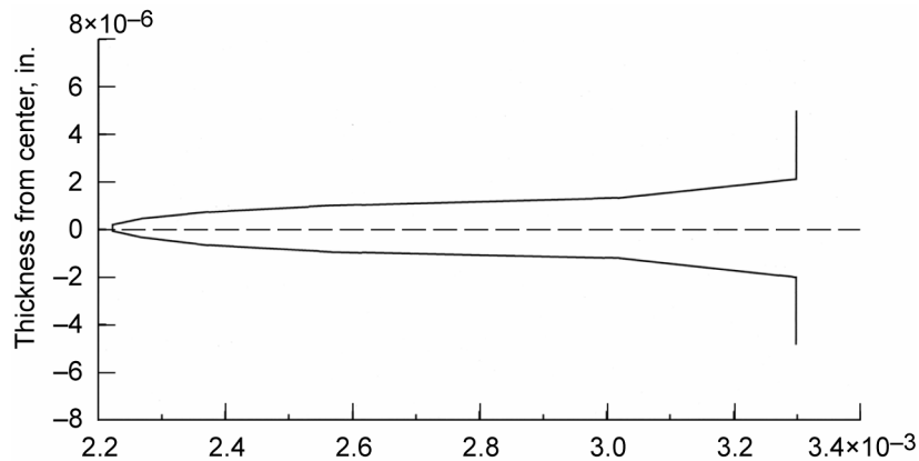
Figure 21.—Nanoscale physical variable transverse moisture expansion, \beta_{T22} (in./in./%M).
