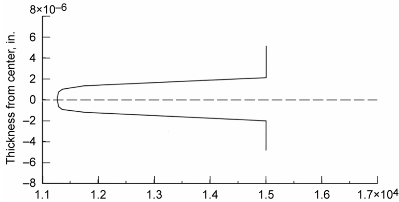
Figure 34.—Nanoscale uniaxial transverse tensile strength, S_{\sigma 22T} (lb/in. 2 ).
