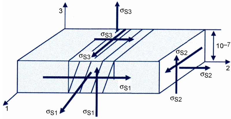
Figure 5.—Nanostresses on a nanosubply (units are in inches).
