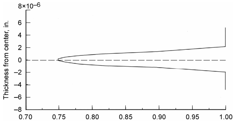
Figure 10.—Nanoscale in situ fabrication parameter, k_m .
