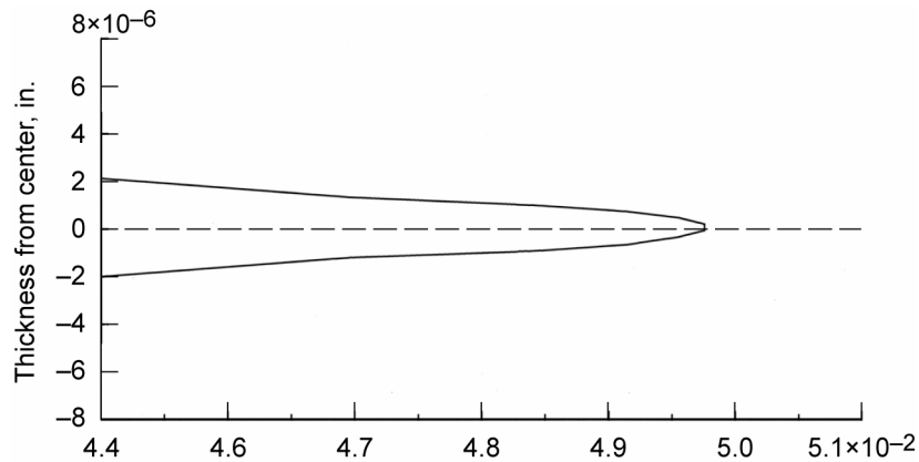
Figure 13.—Nanoscale physical parameter density, \rho_{\ell} (lb/in. 3 ).
