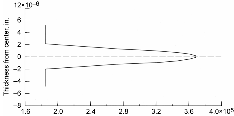
Figure 28.—Nanoscale mechanical property, G_{223} (lb/in. 2 ).
