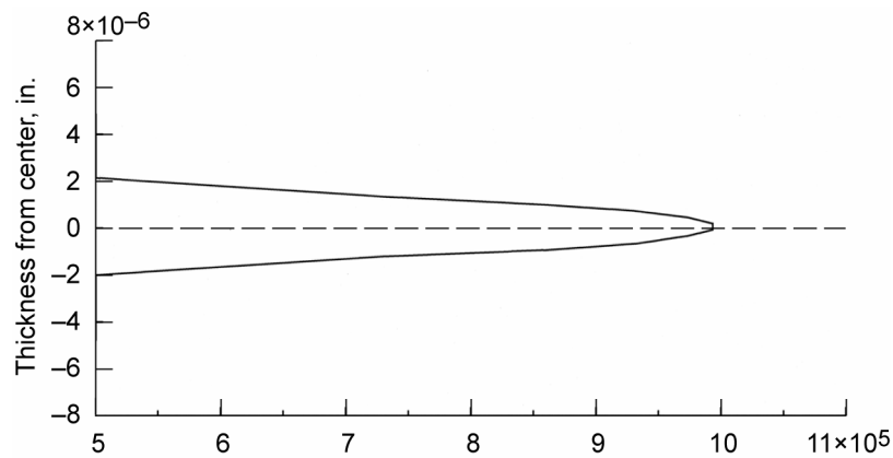
Figure 26.—Nanoscale mechanical property variable transverse modulus, E_{t22} (lb/in. 2 ).
