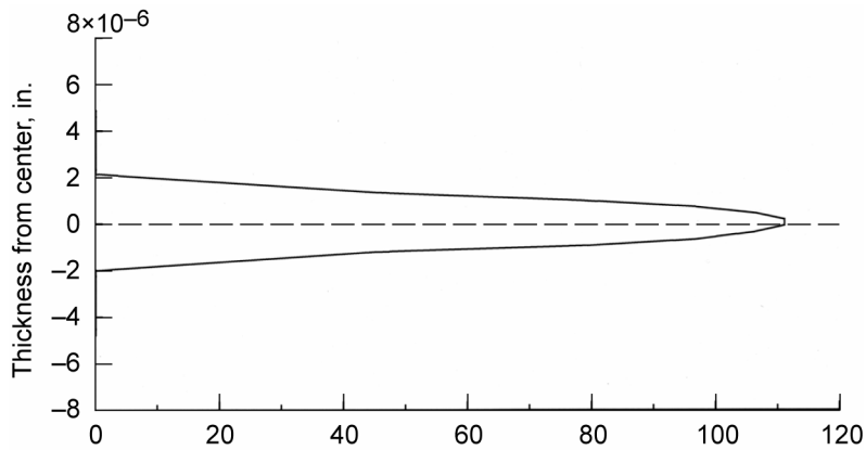
Figure 15.—Nanoscale physical variable longitudinal heat conductivity, K_{11} (Btu/hr/ft 2 /°F/in.).
