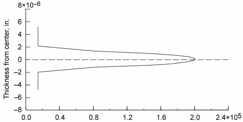
Figure 32.—Nanoscale uniaxial longitudinal tensile strength, S_{\epsilon_{11T}} (lb/in. 2 ).
