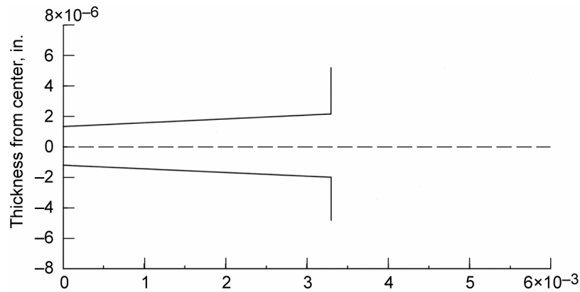
Figure 20.—Nanoscale physical variable longitudinal moisture expansion, \beta_{L11} (in./in./%M).
