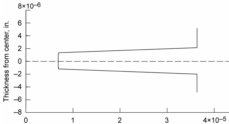
Figure 22.—Nanoscale physical variable longitudinal thermal expansion, \alpha_{11} (in./in./°F).
