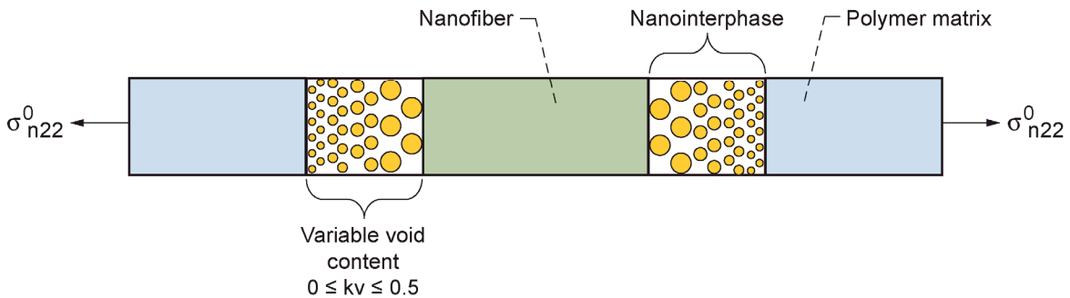
Figure 6.—Vertical section of a composite nanocell through nanofiber center.
