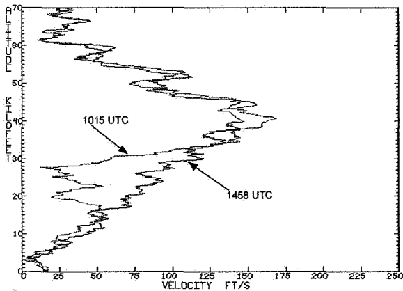
Figure 10. Measure wind velocities on 10 May 2006 between 1015 UTC and 1458 UTC.
