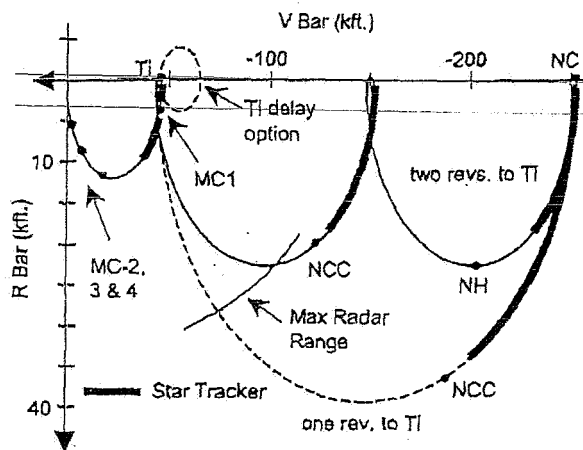
Fig. 13 Stable orbit rendezvous (1983-1997).
