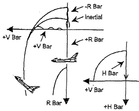
Fig. 7 Proximity operations approaches.
