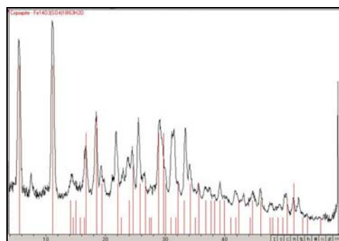
Figure 3. XRD analysis results of the salt of Figure 2: 2D XRD pattern and corresponding 1D diffractogram with phase identification (copiapite).
