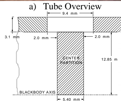
Figure 2: Blackbody Tube.
