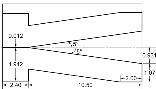
Fig. 1: Schematic of LTSA with dimensions in cm.
