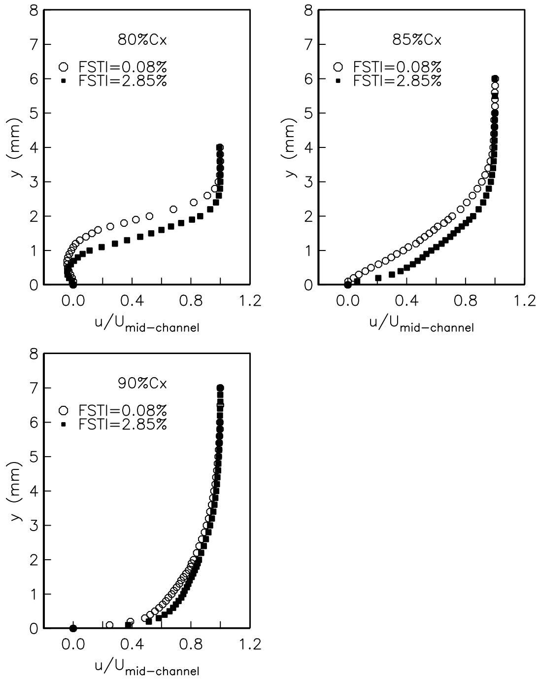
Figure 3.12 (continued). The comparison of the boundary layer profiles for two different freestream turbulence intensities at Re_c = 50,000 .
