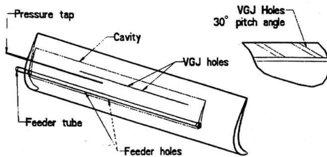
Figure 1.7. The active separation control (ASC) blade geometry (from Bons [3] ).
