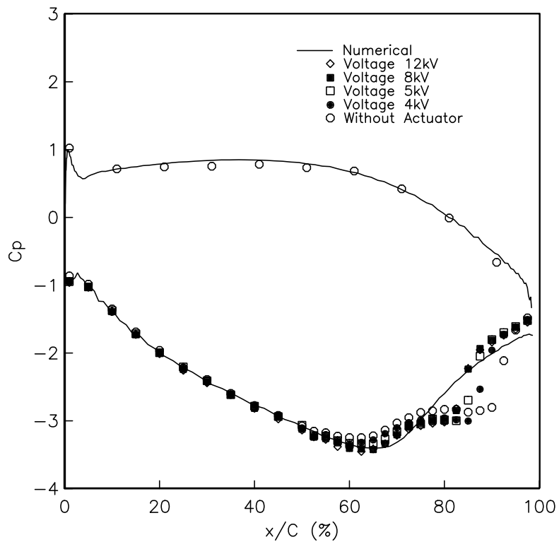
Figure 5.6. Blade pressure distributions with a single steady plasma actuator at 67.5\%C_x , for different actuation levels at Re_c = 50,000 .
