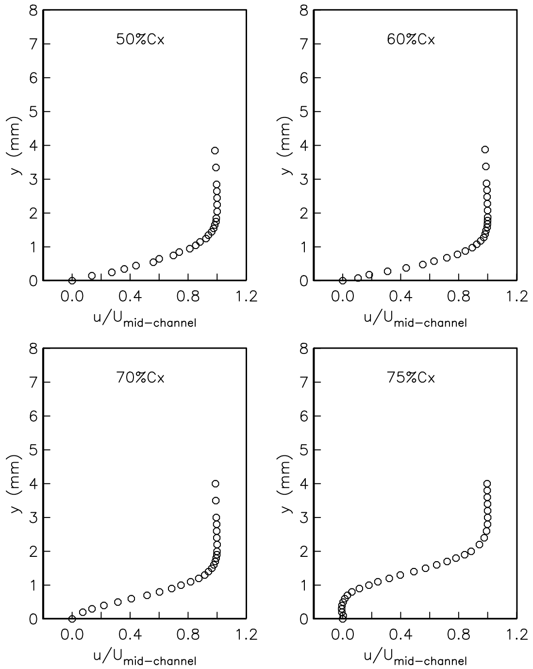
Figure 3.5. Boundary layer profiles for Re=75,000 and FSTI=0.08\% .
