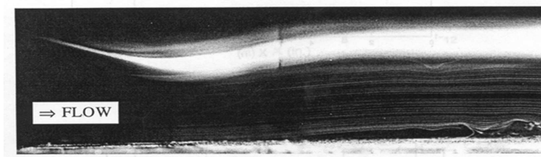
Figure 1.3. The flow visualization of the separation bubble (from Sohn [54] ).
