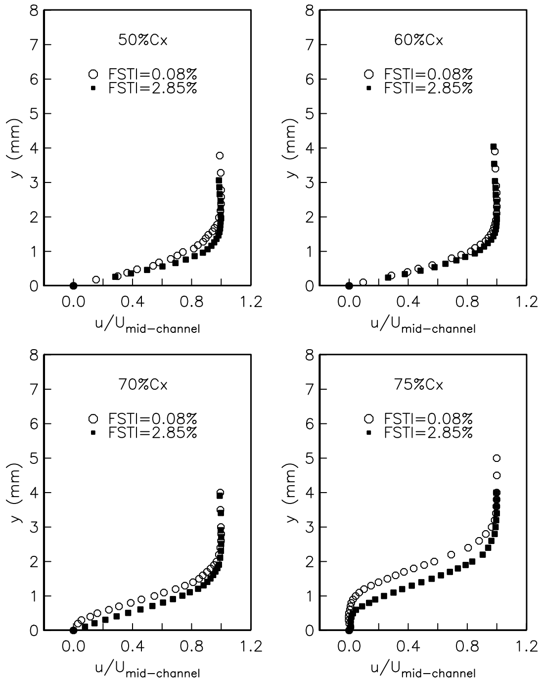
Figure 3.11. The comparison of the boundary layer profiles for two different freestream turbulence intensities at Re_c = 50,000 .
