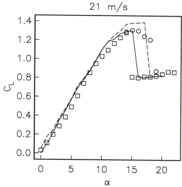
Figure 1.12. Lift coefficient versus angle of attack for NACA-0015 airfoil with leading edge actuator off and on in steady operation (from Corke [10] ).
