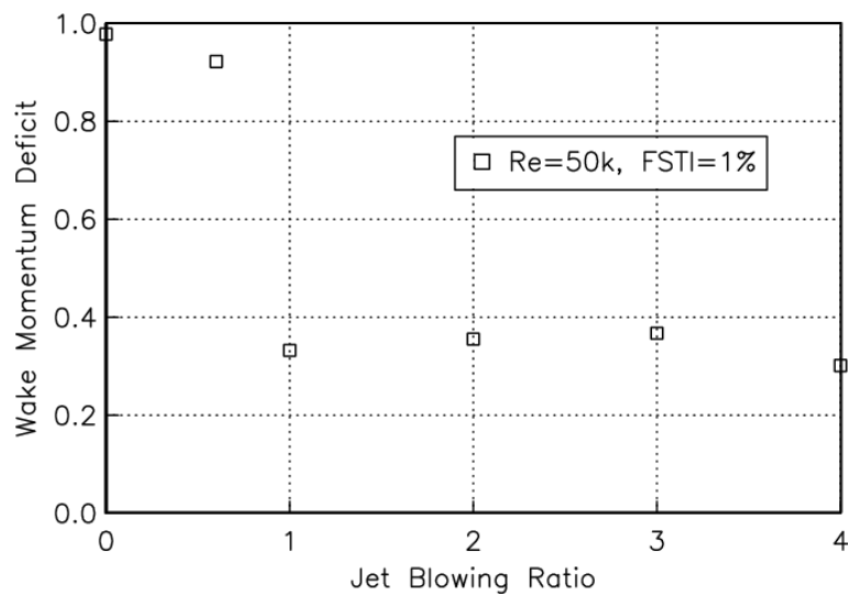
Figure 1.8. Wake momentum deficit vs. blowing ratio (from Bons [3] ).
