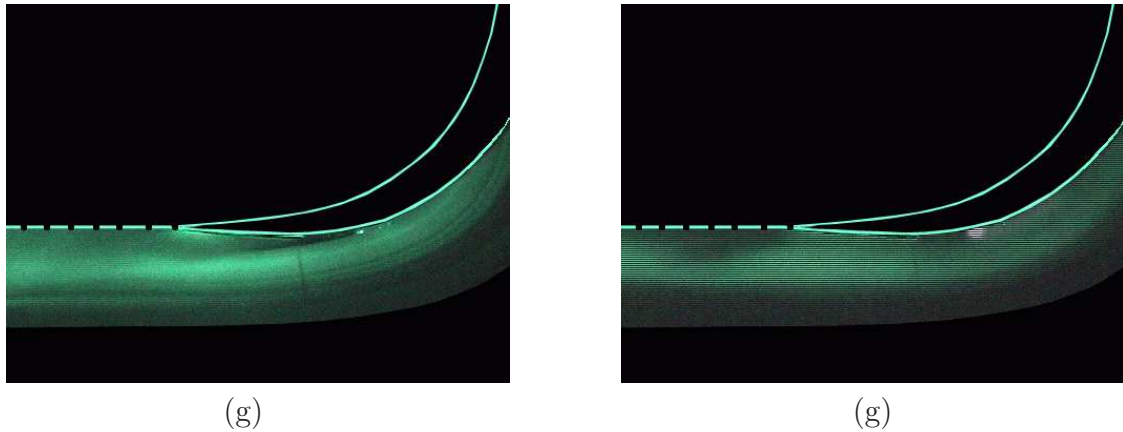
Figure 7.2 (continued). Seven consecutive frames taken from the flow videos for Re_c = 25,000 . The frames in the left column represent the flow field for the uncontrolled case. The frames in the right column represent the flow field when an unsteady plasma actuator was operated. The unsteady plasma actuator was located at x/C_x = 67.5\% and operated at 20 Hz. The actuator amplitude was 8 kV and the plasma duty cycle was 10%.
