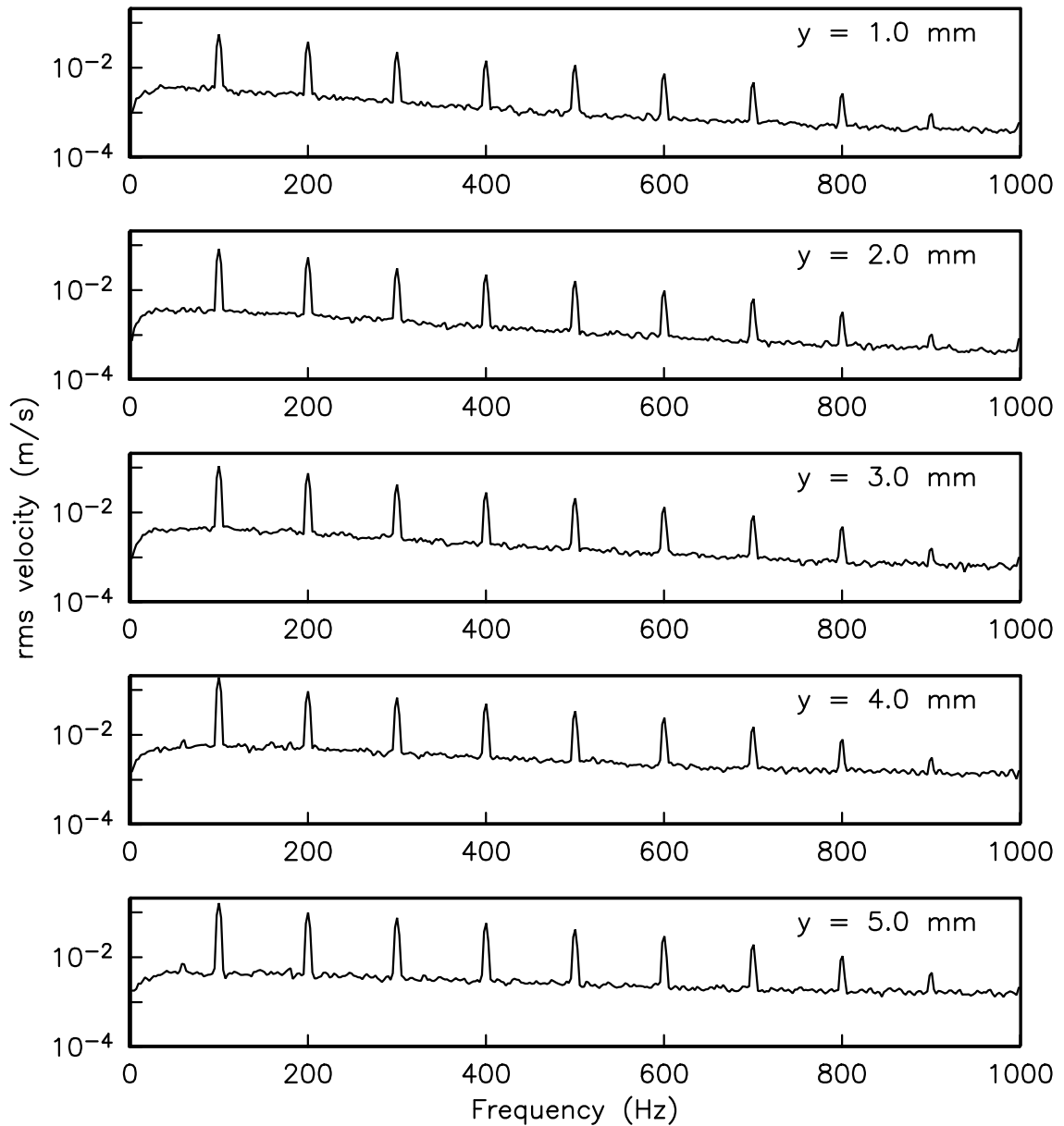
Figure 7.18. Power spectra for five wall normal distances at x/C_x = 90\% for the controlled flow field at Re_c = 50,000 using an unsteady plasma actuator. The plasma actuator was a macor-based actuator and located at x/C_x = 67.5\% . The actuator amplitude was 24 kV. The excitation frequency was 100 Hz and the plasma duty cycle was 10%.
