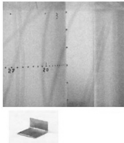
Figure 4.1. Photograph of vortex generator “tabs” on the center blade in cascade, and an individual vortex generator.
