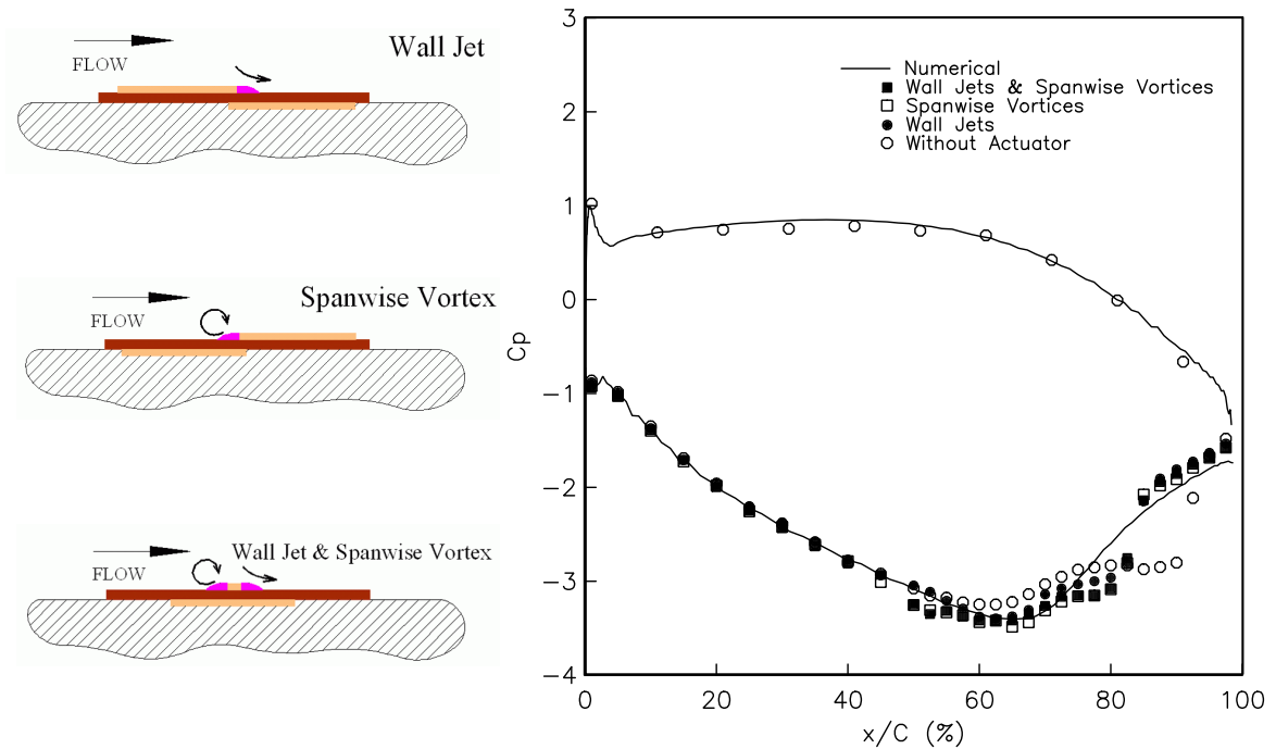
Figure 5.5. Pressure distributions on the “PakB” blade for single steady plasma actuator located at x/C_x = 67.5\% with different electrode orientations ( Re_c = 50,000 ). The actuator amplitude was 8 kV for all the cases.
