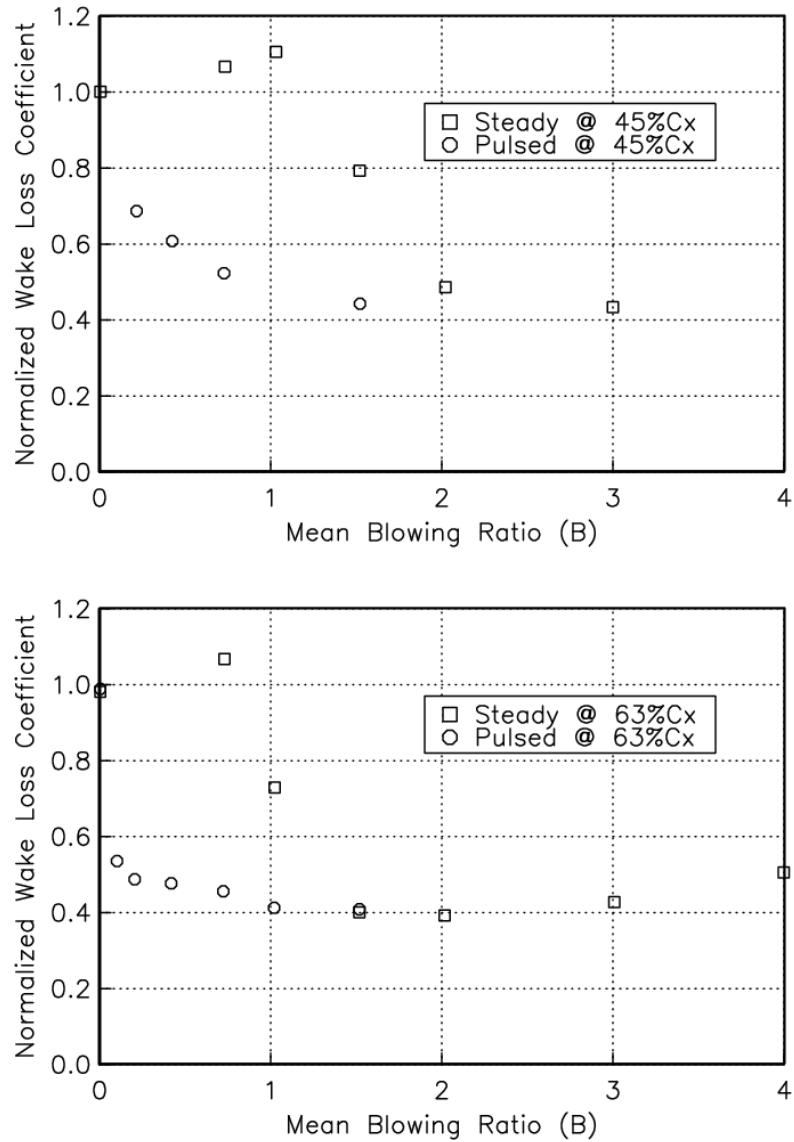
Figure 1.9. The wake loss coefficient normalized by the loss coefficient for B=0 versus the blowing ratio (from Bons [4] ). Data for pulsed blowing at 10 Hz and 50% duty cycle versus steady blowing at Re_c=25,000 .
