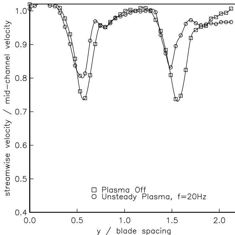
Figure 6.7. The wake profiles of “PakB” cascade for both uncontrolled and controlled cases for Re_c = 25,000 measured 50\%C_x downstream the center blade. For the controlled case, an unsteady plasma actuator was located at x/C_x = 67.5\% and operated at 20 Hz. The actuator amplitude was 8 kV and the plasma duty cycle was 10%.
