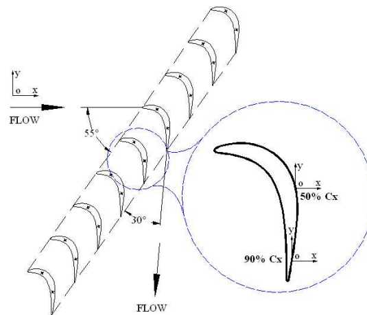
Figure B.1. The coordinate system used in LDV measurements.
