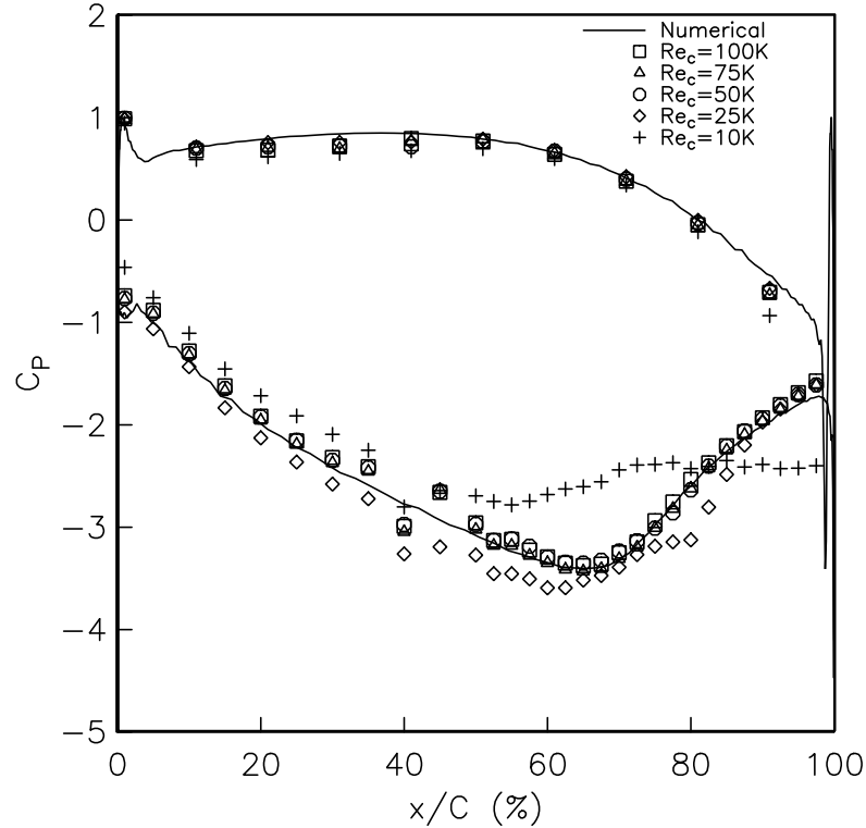
Figure 4.2. Blade pressure distributions with 0.5 in (1.27 cm) spacing of vortex generators for different Reynolds numbers at the lowest freestream turbulence intensity (0.08%).
