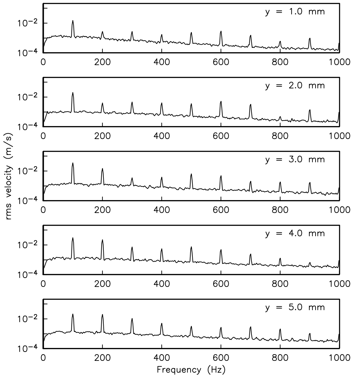
Figure 7.17. Power spectra for five wall normal distances at x/C_x = 85\% for the controlled flow field at Re_c = 50,000 using an unsteady plasma actuator. The plasma actuator was a macor-based actuator and located at x/C_x = 67.5\% . The actuator amplitude was 24 kV. The excitation frequency was 100 Hz and the plasma duty cycle was 10%.
