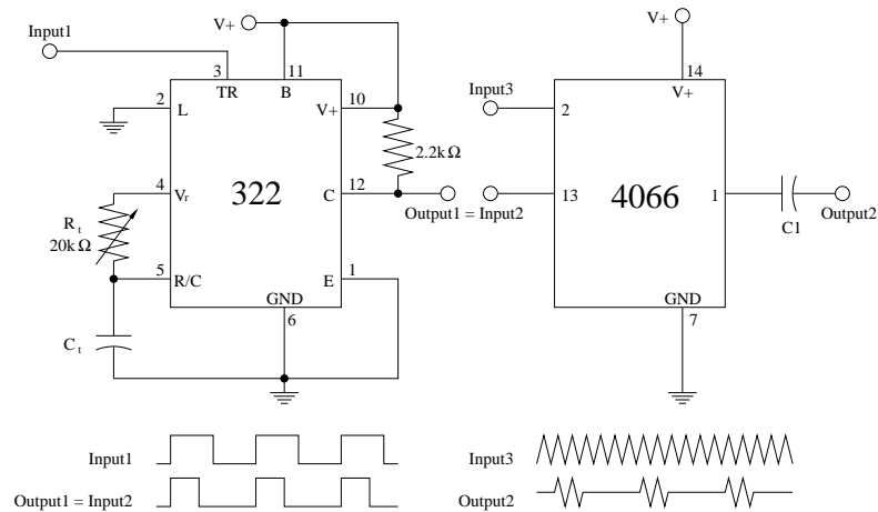
Figure 2.21. This circuit is based on LM322N and CD4066. It was used to control the duty cycle and the frequency of unsteady pulsing.
