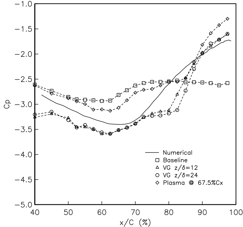
Figure 5.13. Comparison of pressure coefficient distributions in the separation region for vortex generator tabs at two spacings, and a single steady plasma actuator at x/C_x = 67.5\% ( Re_c = 25,000 ). The actuator amplitude was 8 kV for the steady plasma actuator.
