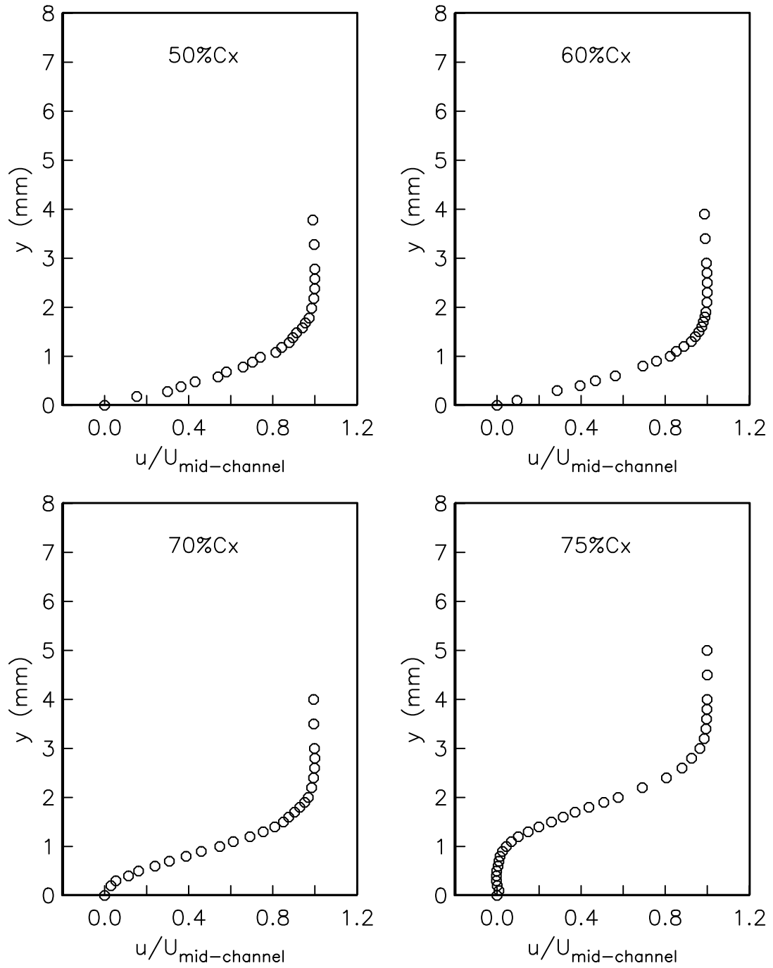
Figure 3.6. Boundary layer profiles for Re=50,000 and FSTI=0.08\% .
