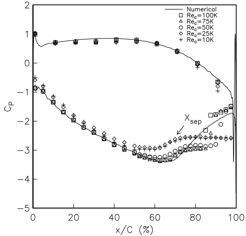
Figure 3.1. Blade pressure coefficient distributions for different Reynolds numbers, for the lowest freestream turbulence intensity (FSTI=0.08%), and comparison to Euler simulation (Romeo [45] ).
