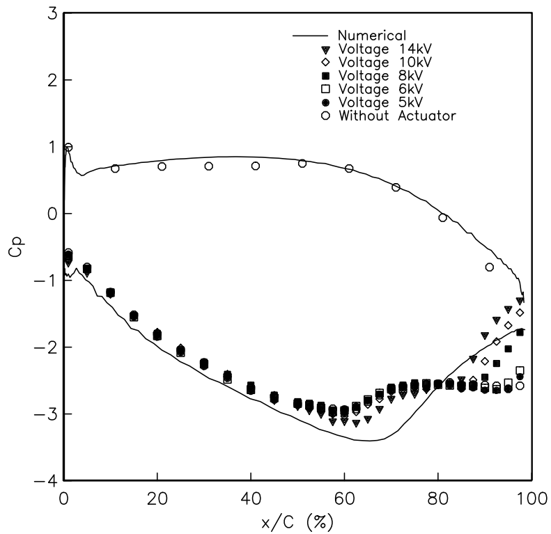
Figure 5.9. Blade pressure coefficient distributions with a single steady plasma actuator at x/C_x = 67.5\% , for different actuation levels at Re_c = 25,000 .
