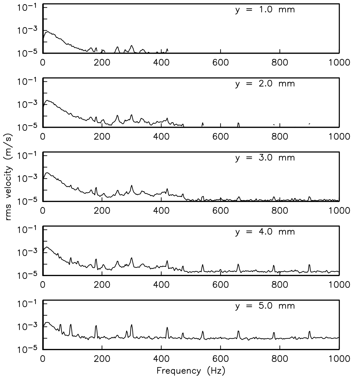
Figure 7.10. Power spectra for five wall normal distances at x/C_x = 80\% for the uncontrolled flow field at Re_c = 50,000 .
