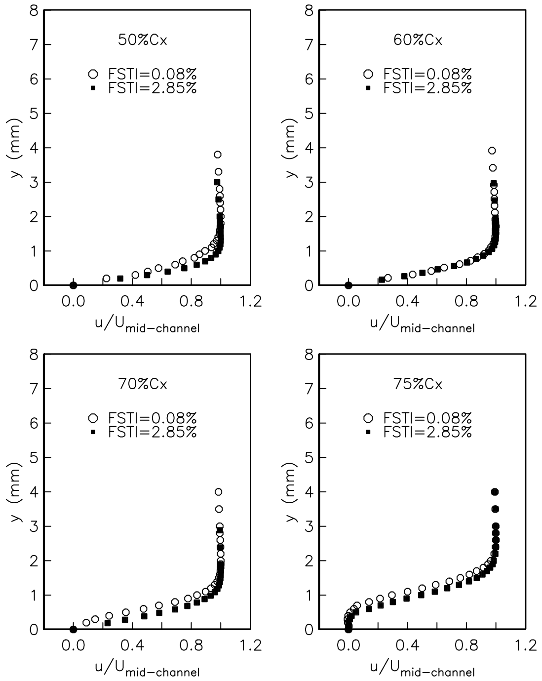
Figure 3.12. The comparison of the boundary layer profiles for two different freestream turbulence intensities at Re_c = 50,000 .
