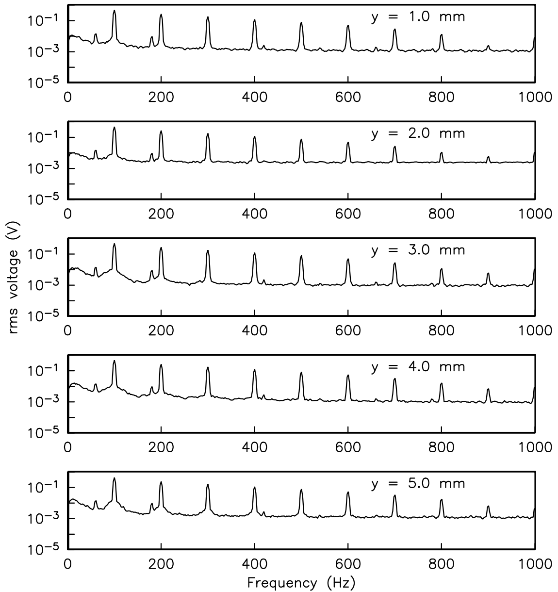
Figure 7.5. Power spectra for five wall normal distances at x/C_x = 85\% for Case 1 in Table 7.1. The unsteady plasma actuator was located at x/C_x = 67.5\% and operated at 100 Hz. The actuator amplitude was 24 kV and the plasma duty cycle was 10%.
