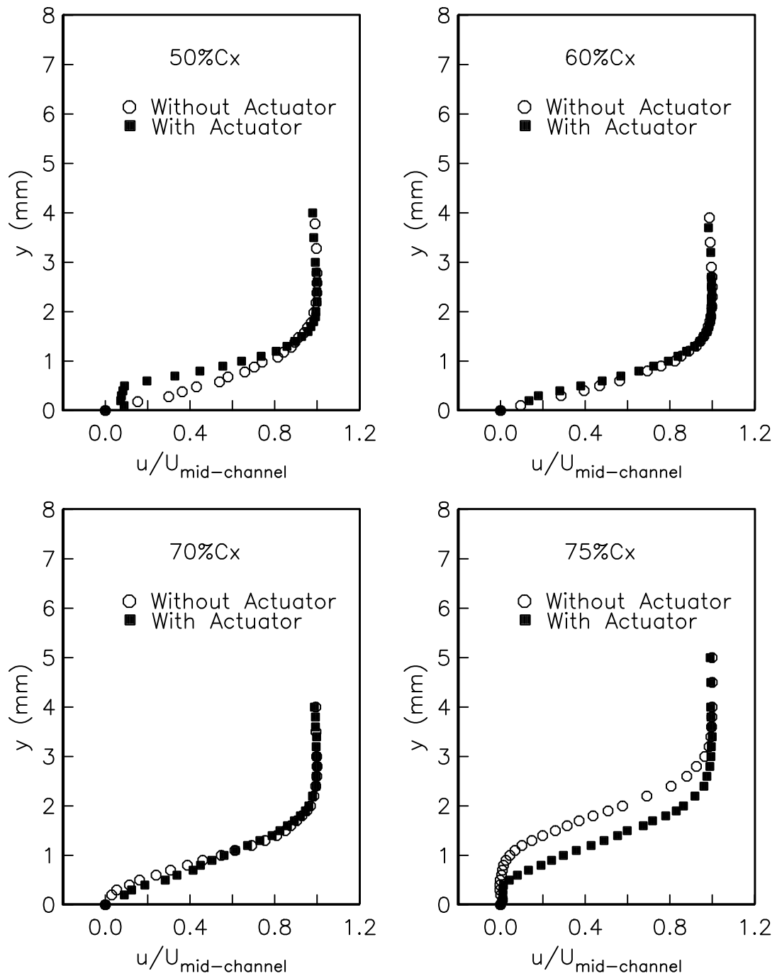
Figure 5.10. The comparison of the boundary layer profiles for uncontrolled and controlled case at Re_c = 50,000 . For the controlled case, a single steady plasma actuator was located at x/C_x = 67.5\% and operated at 8 kV.
