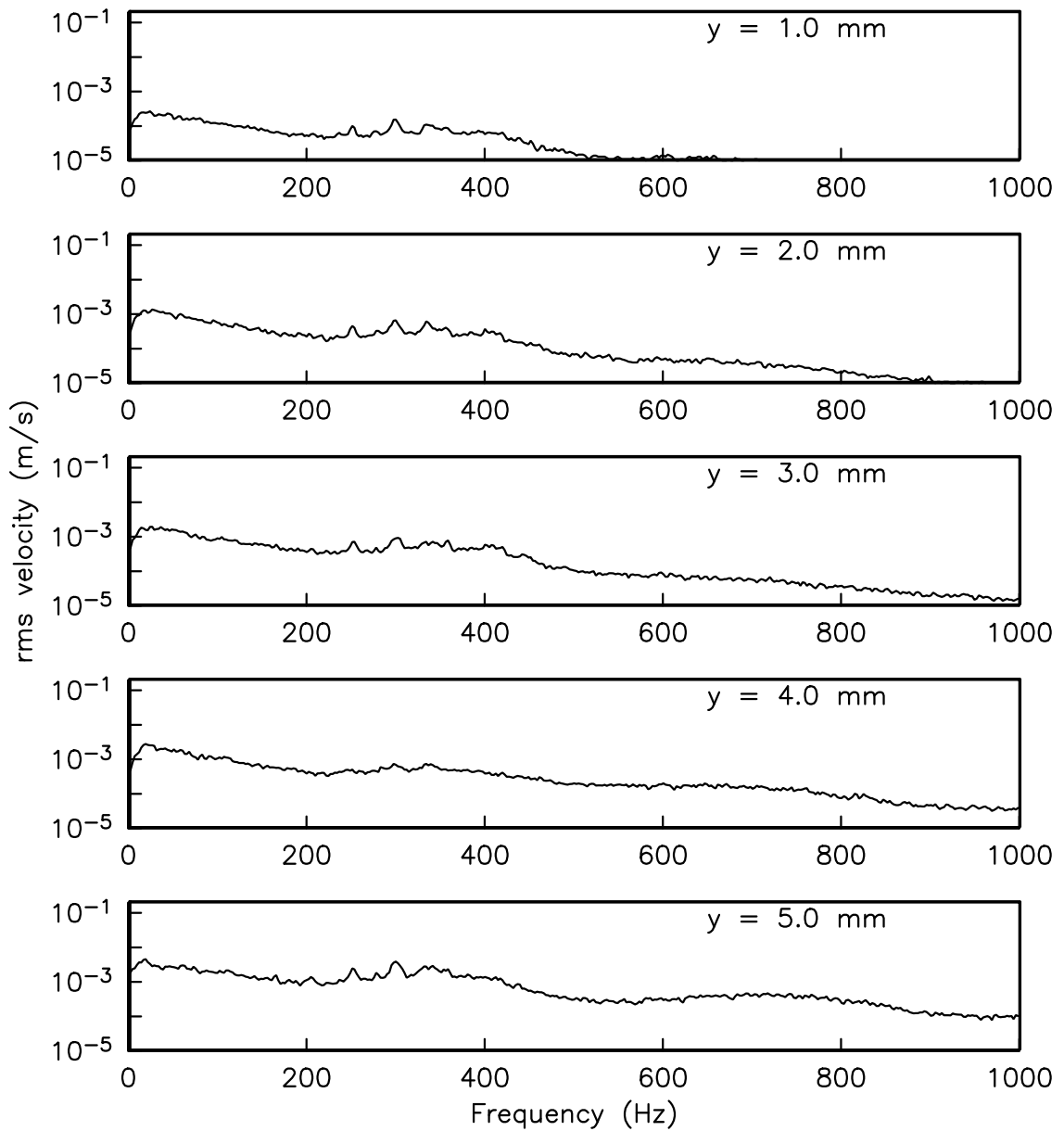
Figure 7.11. Power spectra for five wall normal distances at x/C_x = 85\% for the uncontrolled flow field at Re_c = 50,000 .
