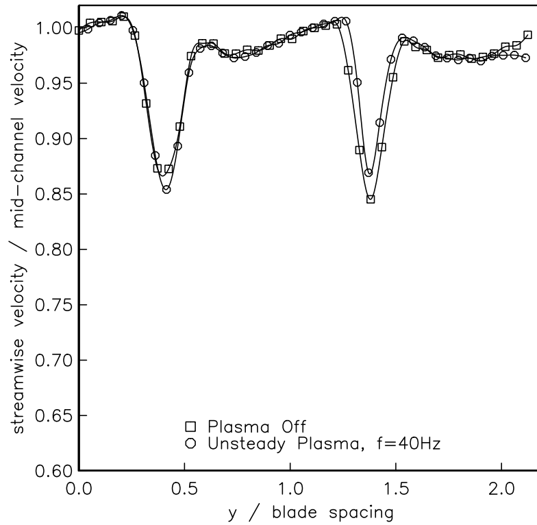
Figure 6.6. The wake profiles of “PakB” cascade for both uncontrolled and controlled cases for Re_c = 50,000 measured 50\%C_x downstream the center blade. For the controlled case, an unsteady plasma actuator was located at x/C_x = 67.5\% and operated at 40 Hz. The actuator amplitude was 8 kV and the plasma duty cycle was 10%.
