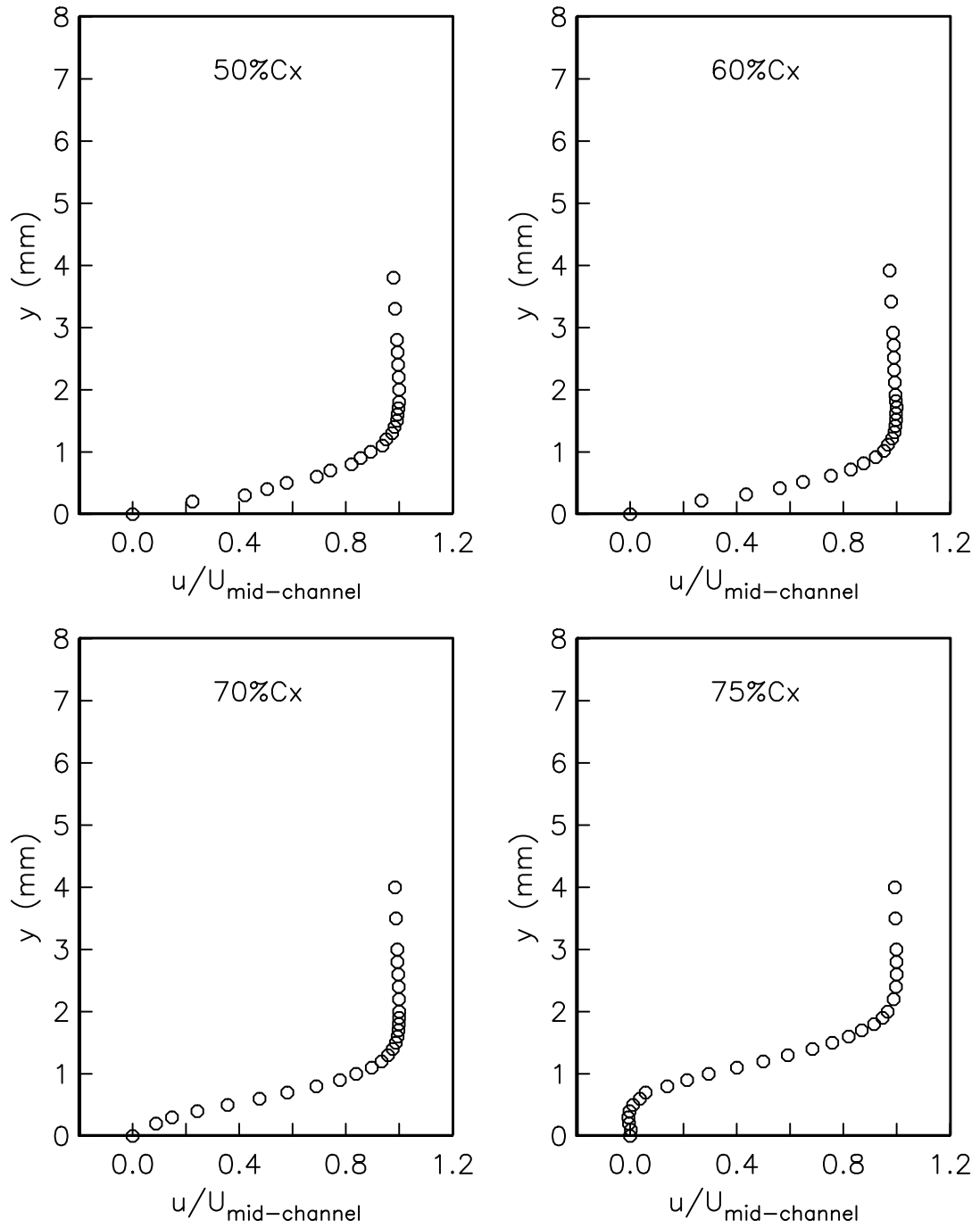
Figure 3.4. Boundary layer profiles for Re=100,000 and FSTI=0.08\% .
