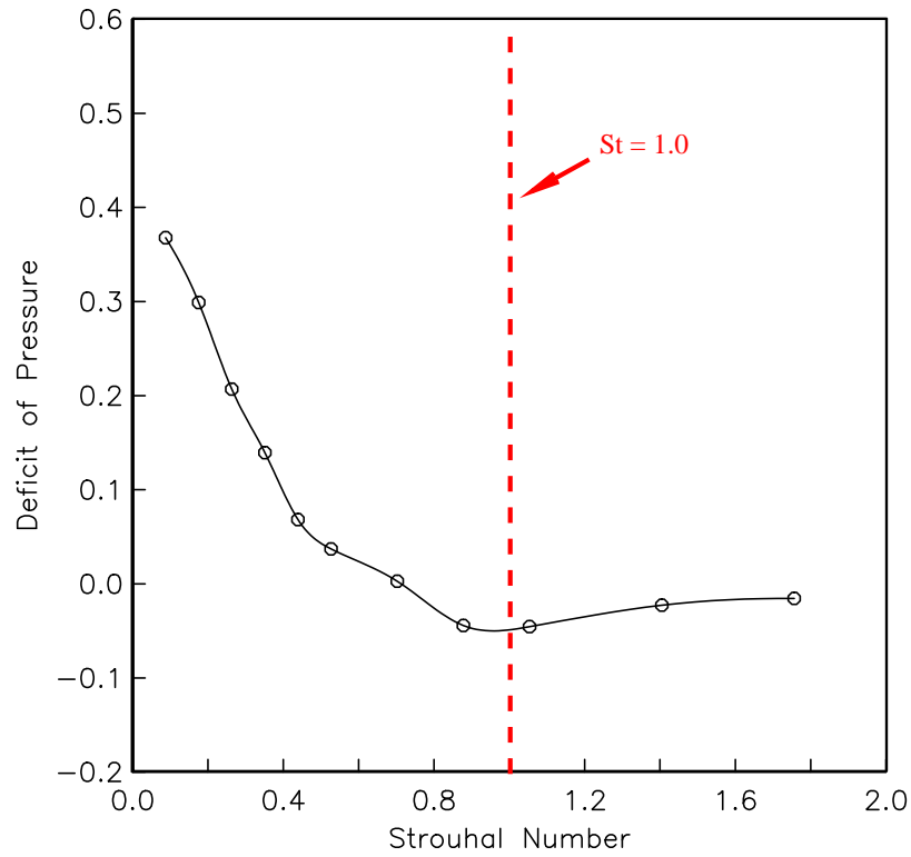
Figure 6.3. Pressure deficit between the experimental results and the numerical result for different excitation frequencies at x/C_x = 85\% for Re_c = 50,000 . The unsteady plasma actuator was a macor-based actuator. It was located at x/C_x = 67.5\% . The actuator amplitude was 24 kV and the plasma duty cycle was 10% for all the cases.
