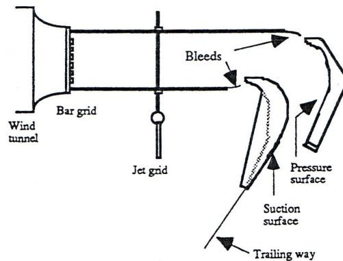
Figure 1.5. The cascade simulator from Qiu [43]’s experiment.
