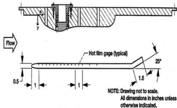
Figure 1.2. The experimental setup of Sohn [54]’s experiment.
