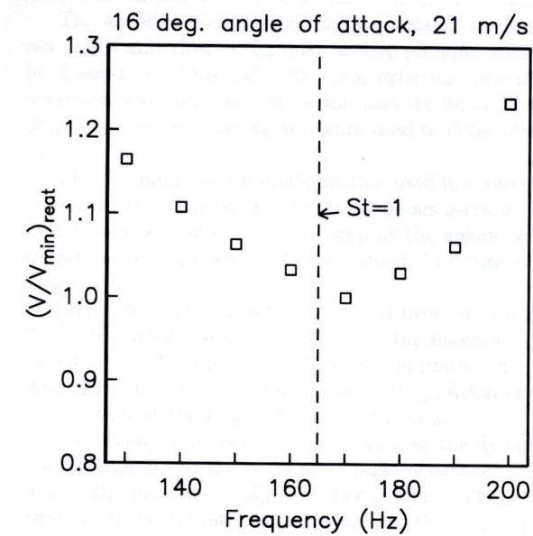
Figure 1.13. Minimum voltage required to reattach the flow as a function of the actuator frequency for unsteady operation (from Corke [10] ).
