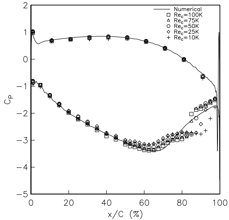
Figure 3.10. Blade pressure coefficient distributions for different Reynolds numbers, for the highest freestream turbulence level (FSTI=2.85%), and comparison to Euler simulation (Romeo [45] ).
