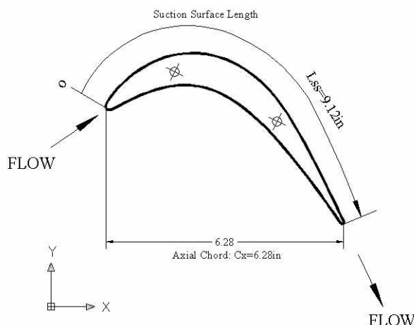
Figure 2.25. The axial chord length and the suction surface length.
