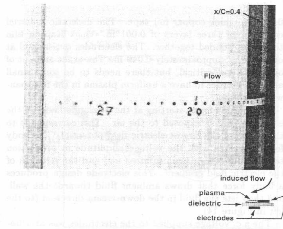
Figure 5.1. Photograph of a plasma actuator located at x/C_x = 40\% on the “PakB” blade with pressure taps.
