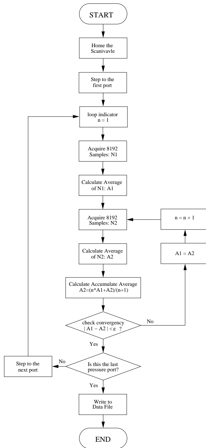
Figure 2.10. The flow chart of pressure measurements.
