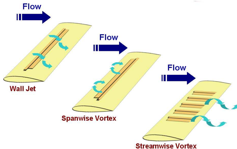
Figure 2.26. Plasma actuators can generate wall jets, spanwise vortices, and streamwise vortices, depending on the orientation of the electrodes.
