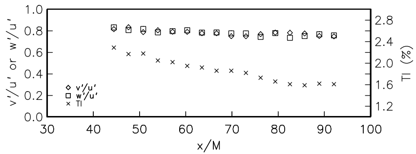
Figure 2.8. Turbulence intensity (TI) and isotropy ( v'/u' and w'/u' ) as a function of streamwise distance for Grid 3.
