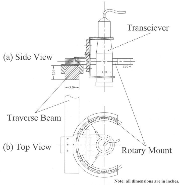
Figure 2.13. Schematic of the rotary mount for LDV measurements.
