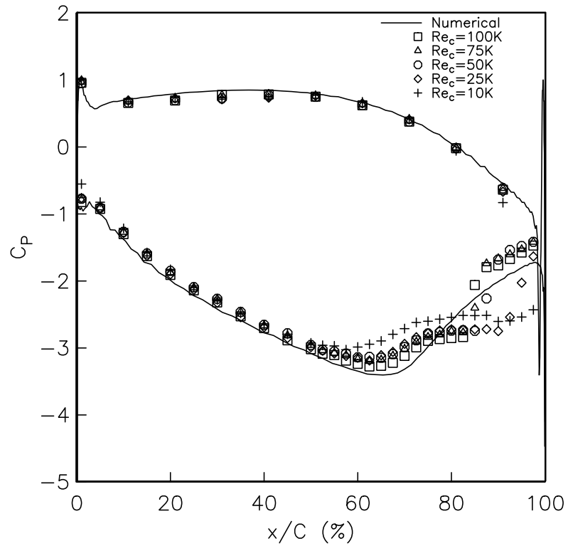
Figure 3.9. Blade pressure coefficient distributions for different Reynolds numbers, for the medium freestream turbulence intensity (FSTI=1.60%), and comparison to Euler simulation (Romeo [45] ).
