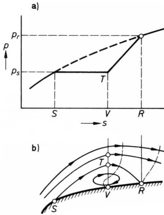
Figure 3.2. “Separation bubble in a laminar boundary layer. a) Pressure distribution in bubble along the wall (schematic). The pressure between S and V in the bubble remains constant at p_s ; further downstream the pressure increases to p_r . b) Shape of bubble (schematic): S =point of separation; R =point of reattachment; V - T =height of bubble.” (from Schlichting [47] )
