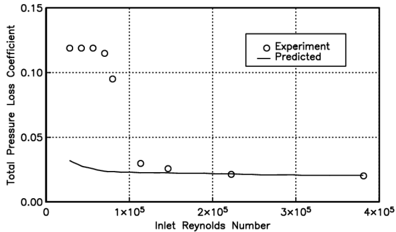
Figure 1.1. Pressure loss of LPT vs. Reynolds number (from Sharma [52] ).
