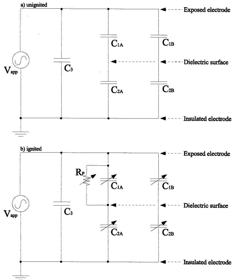
Figure 1.10. Lumped element circuit model of a single dielectric aerodynamic plasma actuator (from Orlov and Corke [37] ).
