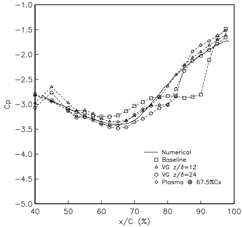
Figure 5.14. Comparison of pressure coefficient distributions in the separation region for vortex generator tabs at two spacings, and a single steady plasma actuator at x/C_x = 67.5\% ( Re_c = 50,000 ). The actuator amplitude was 8 kV for the steady plasma actuator.
