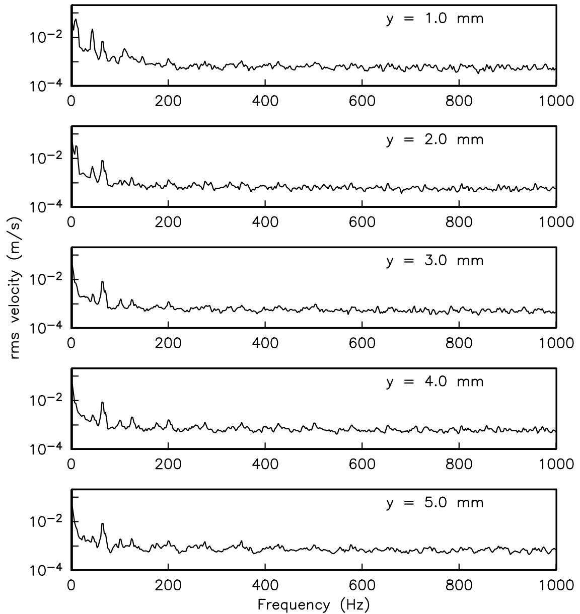
Figure 7.7. Power spectra for five wall normal distances at x/C_x = 60\% for the uncontrolled flow field at Re_c = 50,000 .
