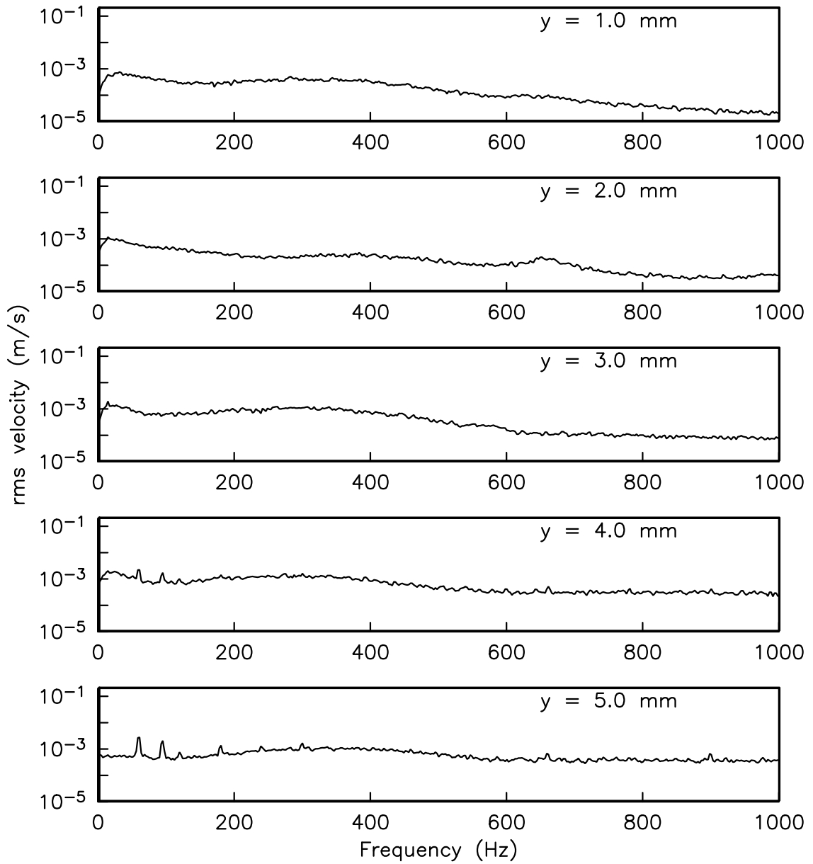
Figure 7.13. Power spectra for five wall normal distances at x/C_x = 80\% for the controlled flow field at Re_c = 50,000 using a steady plasma actuator. The actuator was a kapton-based actuator and located at x/C_x = 67.5\% . The amplitude of the actuator was 8 kV.
