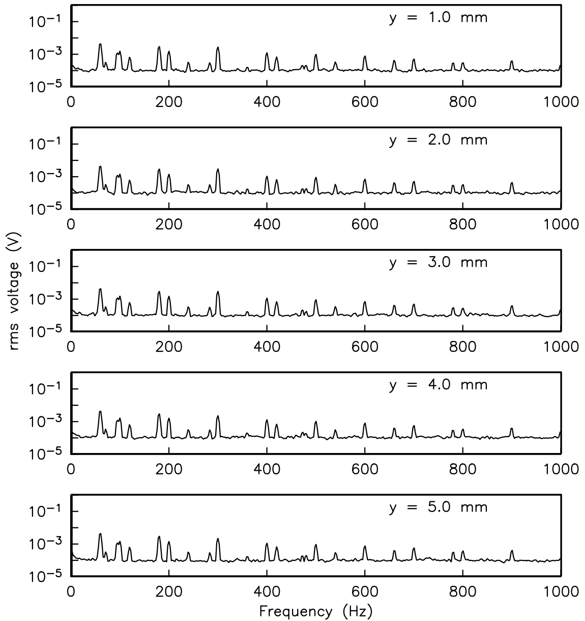
Figure 7.6. Power spectrum for five wall normal distances at x/C_x = 85\% for Case 2 in Table 7.1. The unsteady plasma actuator was located at x/C_x = 67.5\% and operated at 100 Hz. The actuator amplitude was 24 kV and the plasma duty cycle was 10%.
