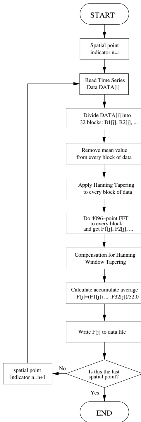
Figure 7.3. The flow chart to calculate the power spectrum.
