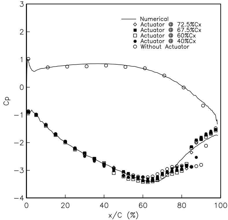
Figure 5.2. Pressure distributions on the “PakB” blade for single steady plasma actuator located at different streamwise locations at Re_c = 50,000 . The actuator voltage amplitude was 8 kV for all the cases.
