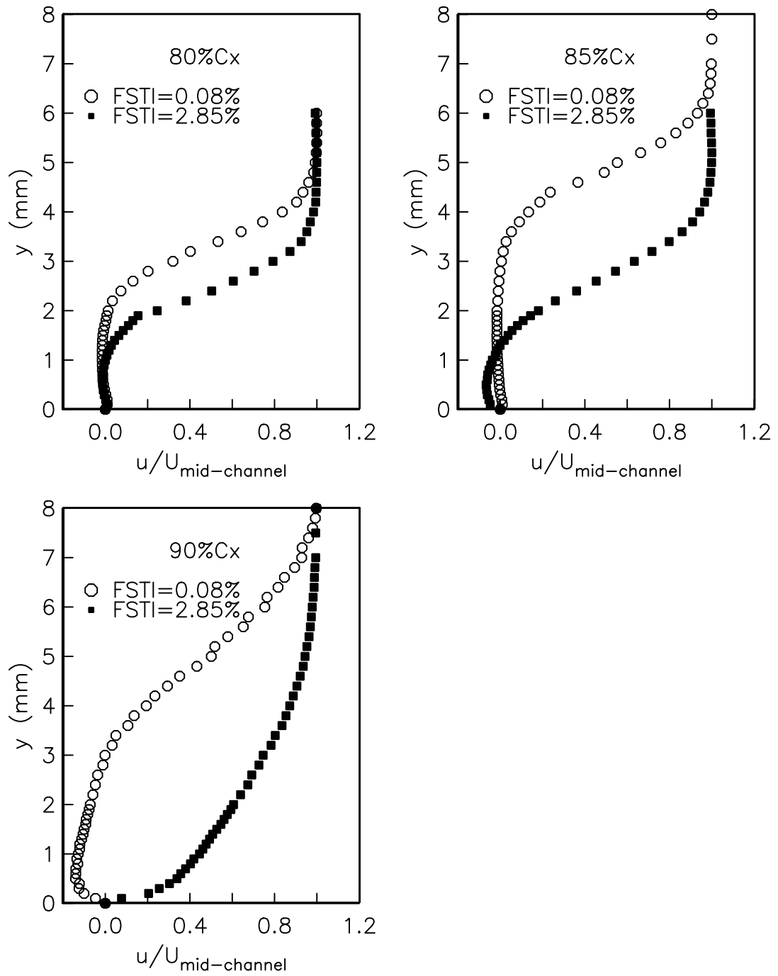
Figure 3.11 (continued). The comparison of the boundary layer profiles for two different freestream turbulence intensities at Re_c = 50,000 .
