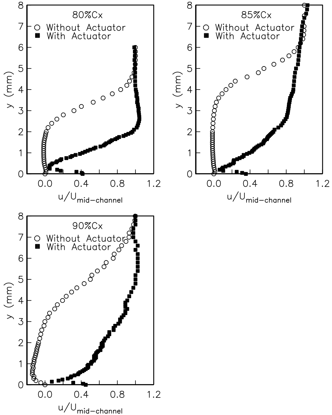
Figure 6.5. The comparison of the boundary layer profiles for uncontrolled and controlled case at Re_c = 50,000 . For the controlled case, an unsteady plasma actuator was located at x/C_x = 67.5\% and operated at 100 Hz. The actuator amplitude was 24 kV and the plasma duty cycle was 10%.
