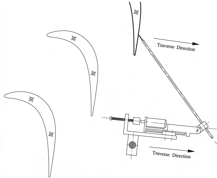
Figure 2.15. The schematics of the mini-traverse system for hot-wire measurements.
