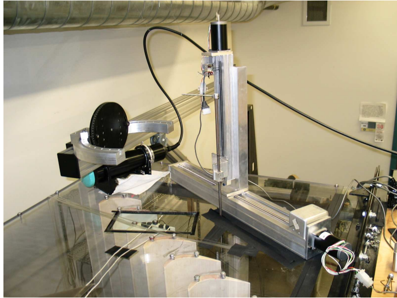
Figure 2.22. A traverse slot was cut into the top of the test section so that the traverse system can move the five-hole probe along the trailing edge of the cascade.
