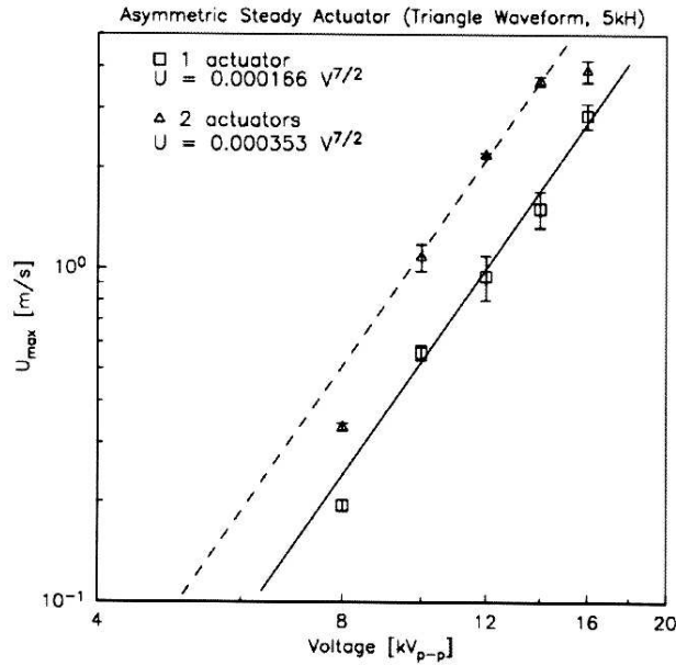
Figure 1.11. Relationship between actuator voltage and velocity output for one and two steady actuators (from Post [41] ).
