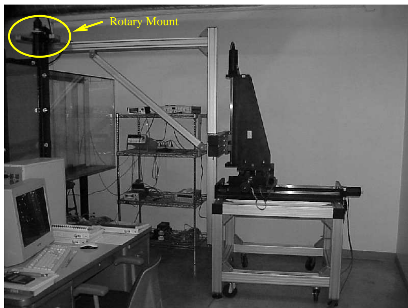
Figure 2.11. The transceiver of the LDV system is mounted on a computer controlled traverse table using a specially designed rotary mount shown at the top of the boom arm in the upper left of the photograph.
