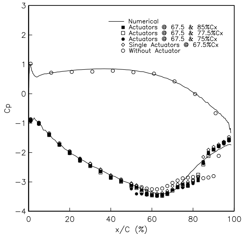
Figure 5.4. Pressure distributions on the “PakB” blade for dual steady plasma actuators ( Re_c = 50,000 ). The first actuator was kept at x/C_x = 67.5\% and the location of the second actuator was varied from x/C_x = 75\% to 85\% . The actuator amplitude was 8 kV for both actuators.
