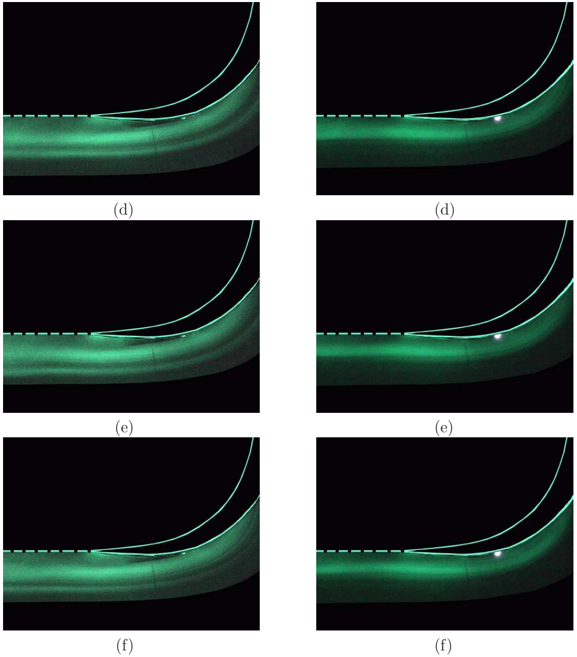
Figure 7.1 (continued). Seven consecutive frames taken from the flow videos for Re_c = 25,000 . The frames in the left column represent the flow field for the uncontrolled case. The frames in the right column represent the flow field when a steady plasma actuator was operated. The steady plasma actuator was located at x/C_x = 67.5\% . The actuator amplitude was 8 kV.
