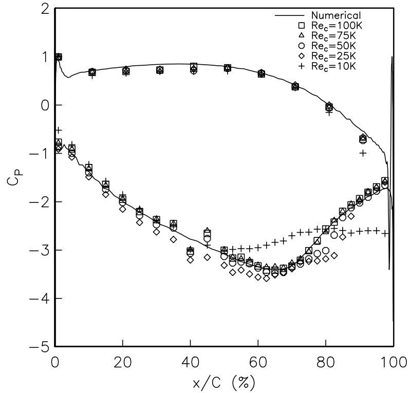
Figure 4.3. Blade pressure distributions with 1.0 in (2.54 cm) spacing of vortex generators for different Reynolds numbers at the lowest freestream turbulence intensity (0.08%).
