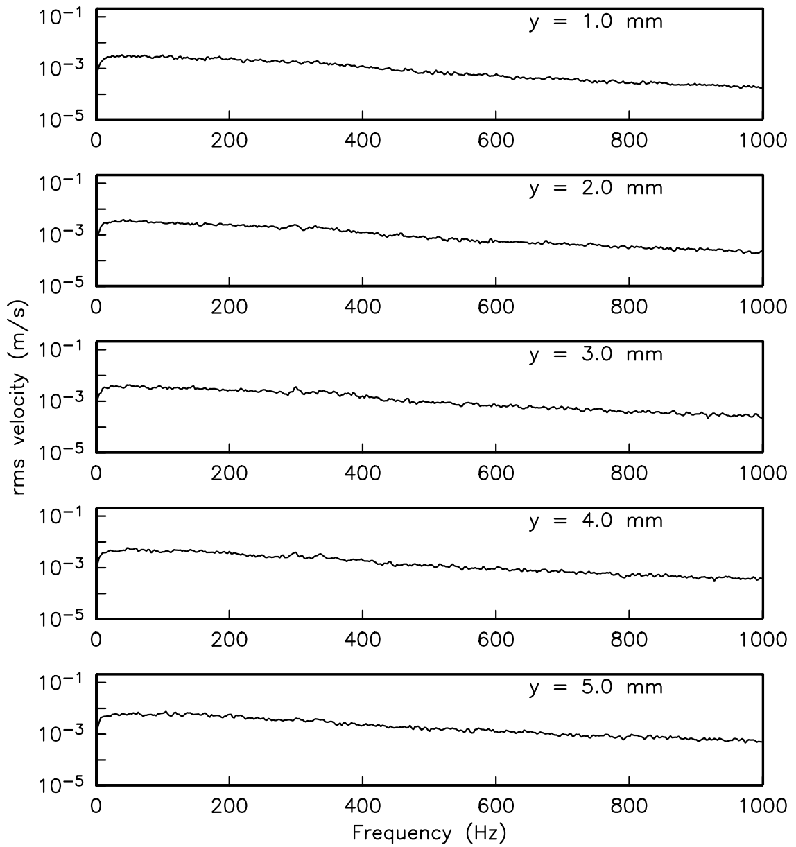
Figure 7.12. Power spectra for five wall normal distances at x/C_x = 90\% for the uncontrolled flow field at Re_c = 50,000 .
