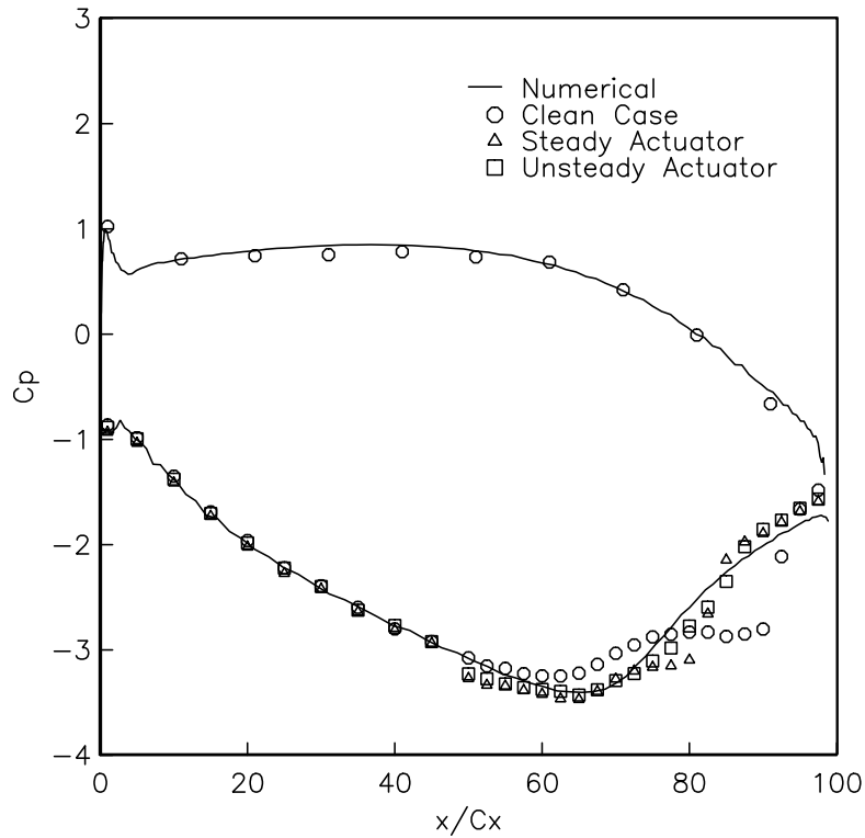
Figure 6.12. Comparison of the blade pressure distributions between the most effective steady actuator and unsteady actuators for Re_c = 50,000 . The steady actuator was a kapton-based actuator and located at x/C_x = 67.5\% . The amplitude for the steady actuator was 8 kV. The unsteady actuator was a macor-based actuator and located at x/C_x = 67.5\% . The excitation frequency was 100 Hz, which corresponded to S_t = 0.9 . The actuator amplitude was 24 kV and the plasma duty cycle was 10%.
