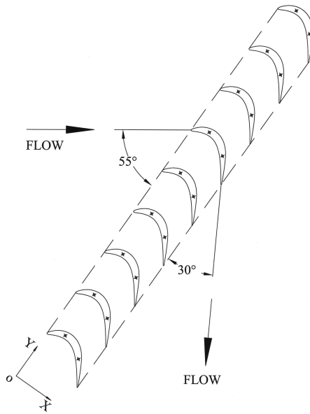
Figure 2.5. The linear cascade consists of nine “PakB” blades.
