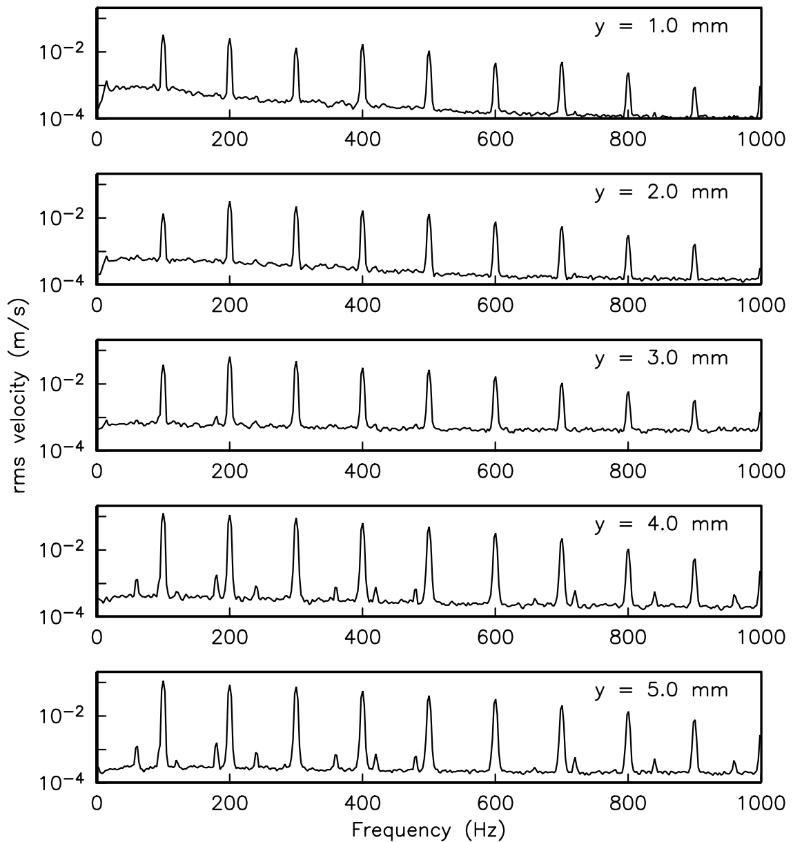
Figure 7.16. Power spectra for five wall normal distances at x/C_x = 80\% for the controlled flow field at Re_c = 50,000 using an unsteady plasma actuator. The plasma actuator was a macor-based actuator and located at x/C_x = 67.5\% . The actuator amplitude was 24 kV. The excitation frequency was 100 Hz and the plasma duty cycle was 10%.
