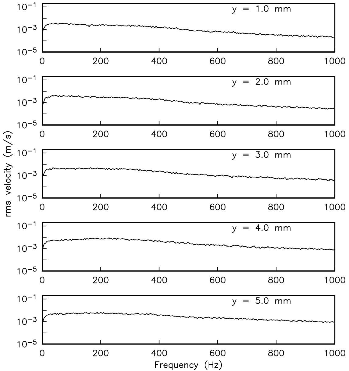
Figure 7.14. Power spectra for five wall normal distances at x/C_x = 85\% for the controlled flow field at Re_c = 50,000 using a steady plasma actuator. The actuator was a kapton-based actuator and located at x/C_x = 67.5\% . The amplitude of the actuator was 8 kV.
