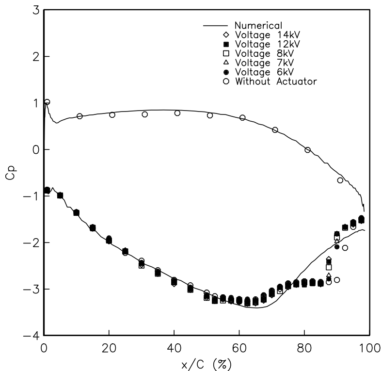
Figure 5.7. Blade pressure coefficient distribution with a single steady plasma actuator at 40\%C_x , for different actuation levels at Re_c = 50,000 .
