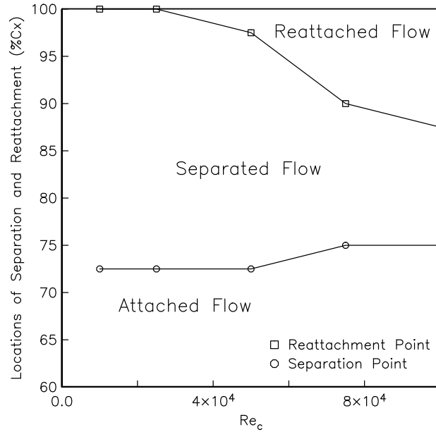
Figure 3.3. Separation and reattachment locations as a function of Reynolds number for the lowest turbulence intensity (FSTI=0.08%).
