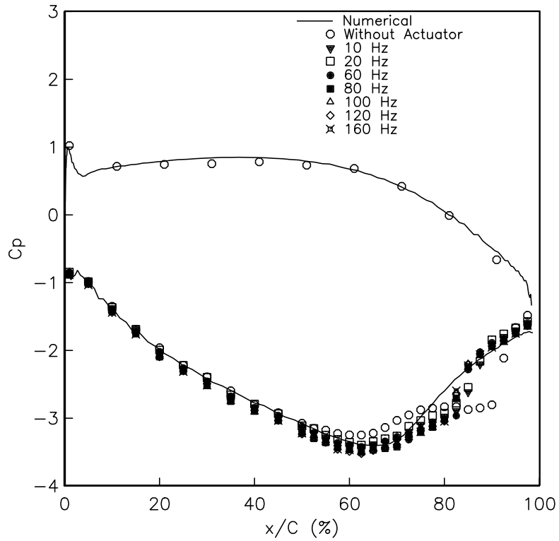
Figure 6.2. Blade pressure distributions at Re_c = 50,000 for different excitation frequencies of unsteady plasma actuator. The unsteady plasma actuator was a macor-based actuator. It was located at x/C_x = 67.5\% . The actuator amplitude was 24 kV and the plasma duty cycle was 10% for all the cases.
