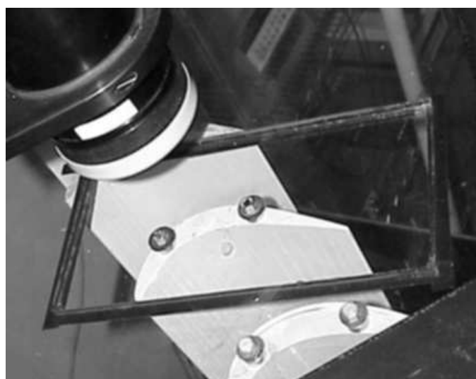
Figure 2.12. A rectangular window was cut into Lexan ceiling and replaced with a piece of \frac{1}{8} " thick regular glass to give better optical access for LDV system.
