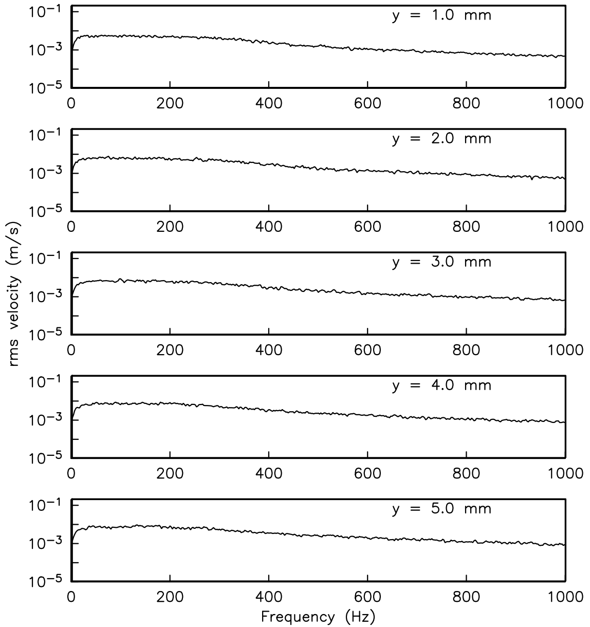
Figure 7.15. Power spectra for five wall normal distances at x/C_x = 90\% for the controlled flow field at Re_c = 50,000 using a steady plasma actuator. The actuator was a kapton-based actuator and located at x/C_x = 67.5\% . The amplitude of the actuator was 8 kV.
