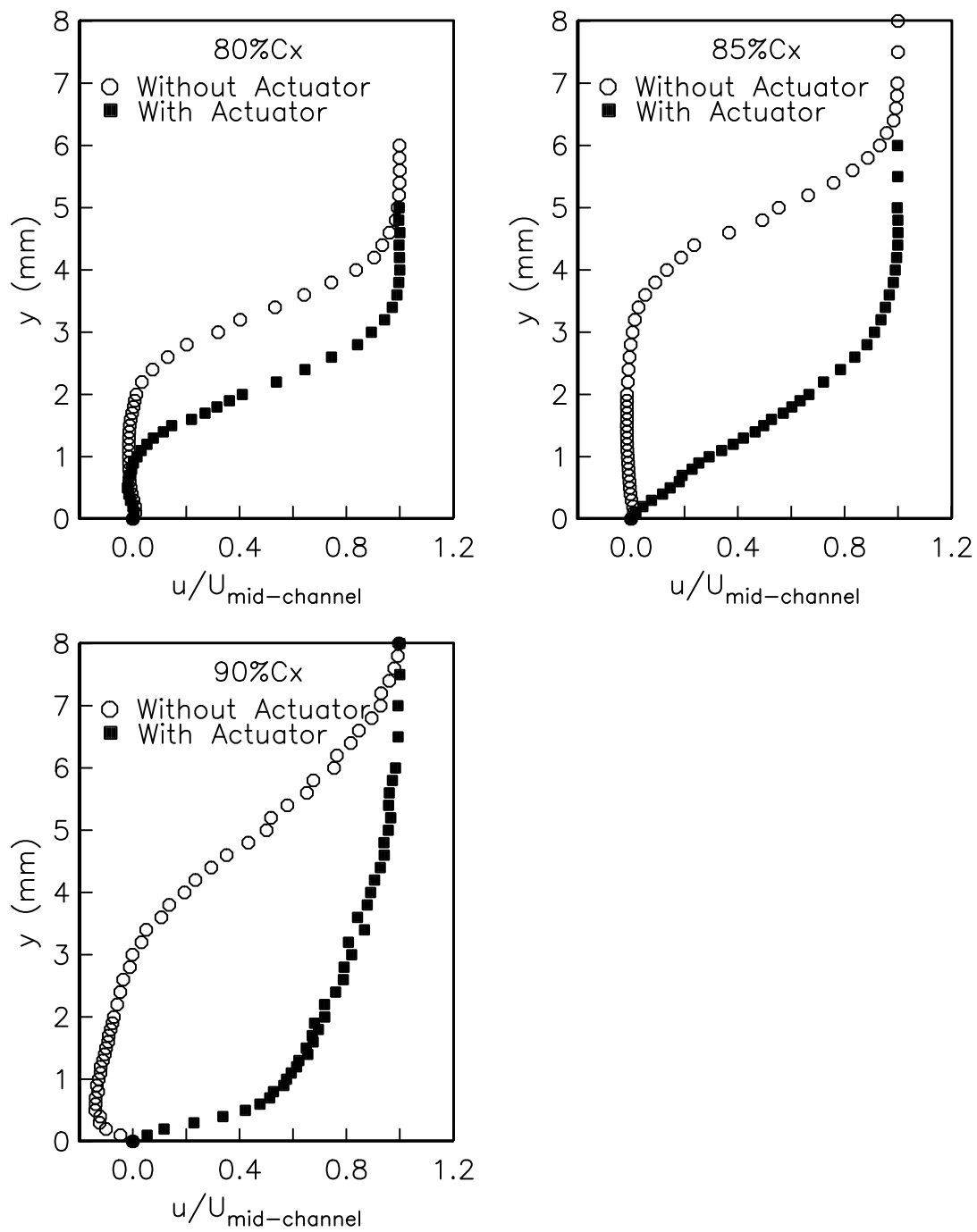
Figure 5.10 (continued). The comparison of the boundary layer profiles for uncontrolled and controlled case at Re_c = 50,000 . For the controlled case, a single steady plasma actuator was located at x/C_x = 67.5\% and operated at 8 kV.
