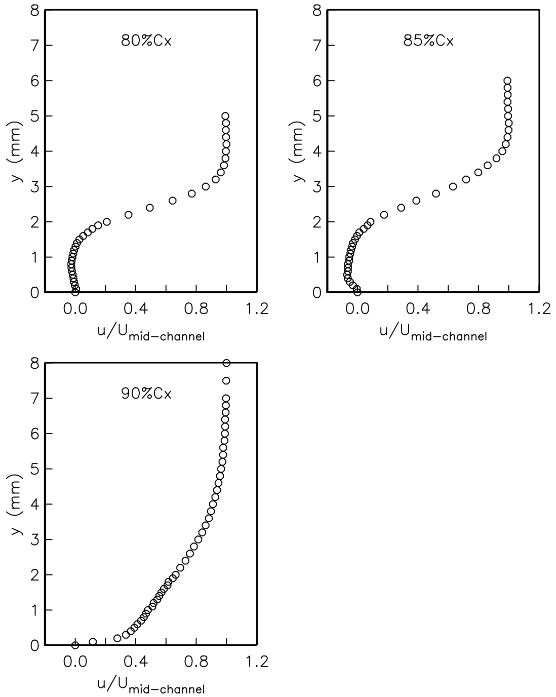
Figure 3.5 (continued). Boundary layer profiles for Re=75,000 and FSTI=0.08\% .
