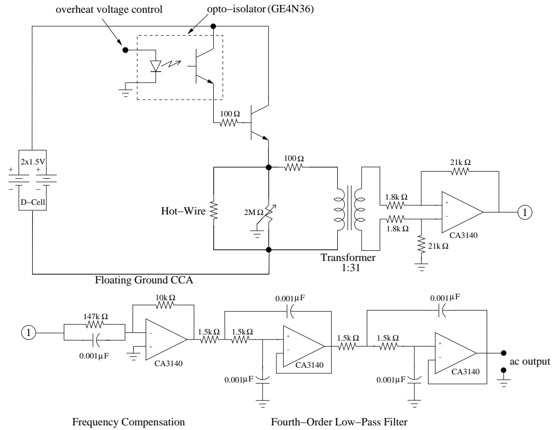
Figure 2.17. A constant-current anemometer was specially designed to analyze the hot-wire signal when plasma actuators were operated.
