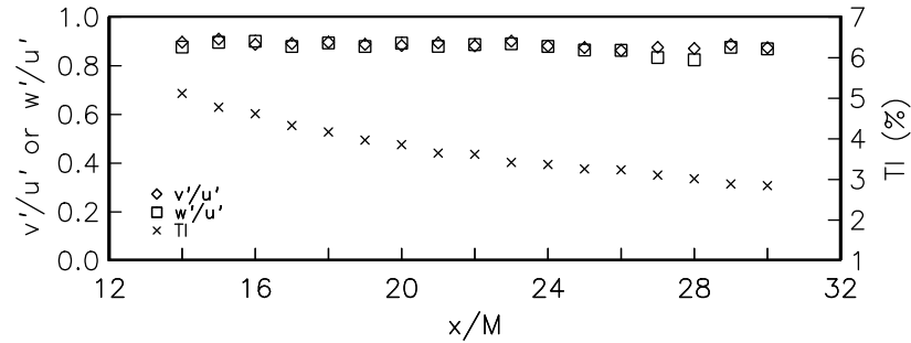
Figure 2.9. Turbulence intensity (TI) and isotropy ( v'/u' and w'/u' ) as a function of streamwise distance for Grid 0.
