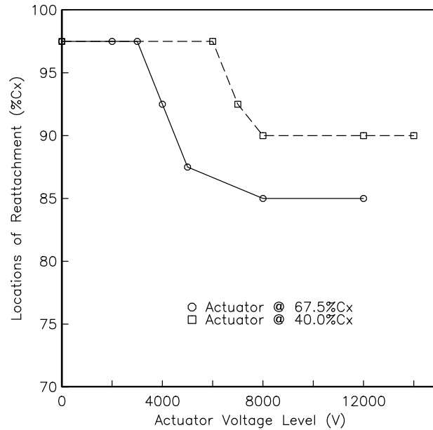
Figure 5.8. Effect of steady plasma actuator amplitude on reattachment location for two actuator positions ( Re_c = 50,000 ).
