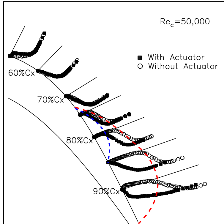
Figure 5.11. The boundary layer profiles on “PakB” blade for uncontrolled and controlled case at Re_c = 50,000 . For the controlled case, a single steady plasma actuator was located at x/C_x = 67.5\% and operated at 8 kV. The separation bubbles are sketched using dashed lines. The larger separation bubble for the uncontrolled case is reduced to the smaller one when the plasma actuator is operated.
