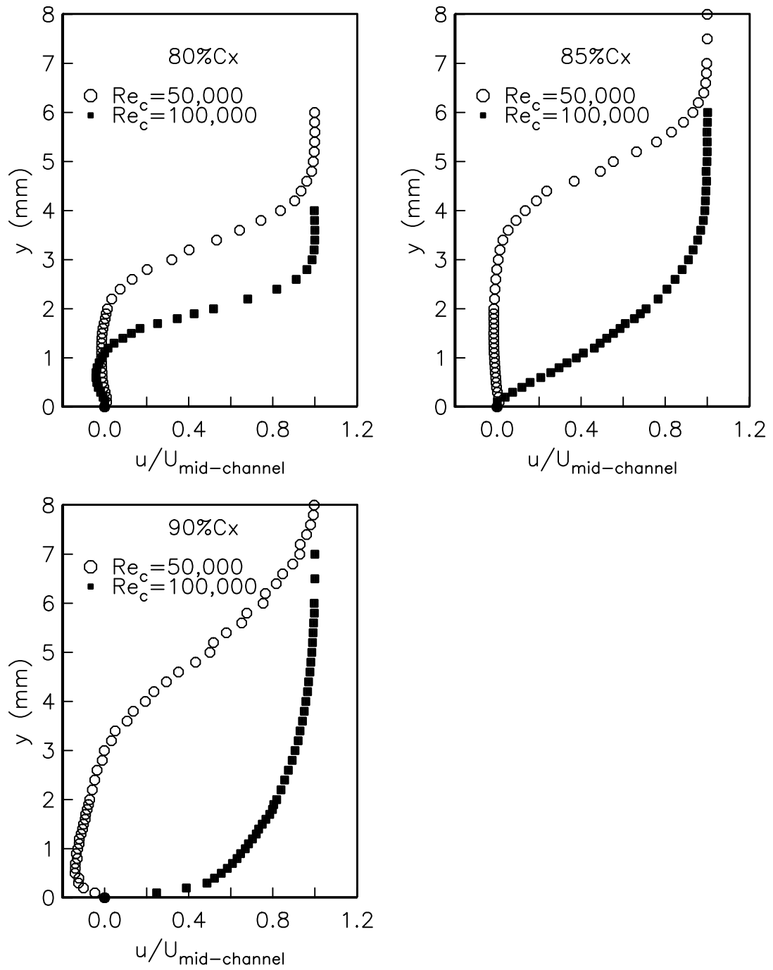
Figure 3.7 (continued). Boundary layer profiles for Re_c = 50,000 and Re_c = 100,000 for FSTI=0.08\% .
