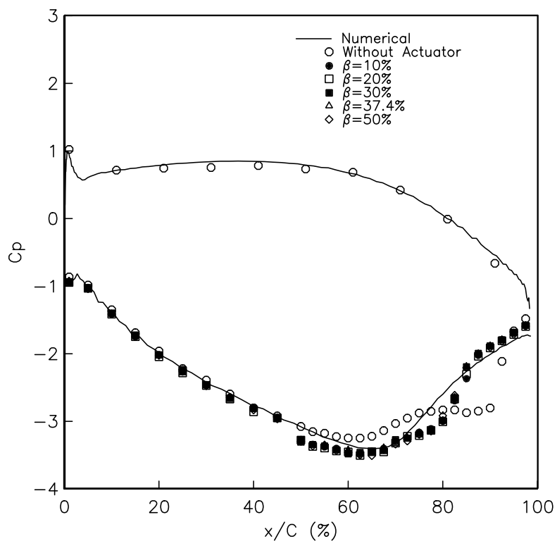
Figure 6.4. Blade pressure distributions at Re_c = 50,000 for different plasma duty cycles of unsteady plasma actuator. The unsteady plasma actuator was a kapton-based actuator. It was located at x/C_x = 67.5\% . The excitation frequency was 40 Hz and the actuator amplitude was 8 kV for all the cases.
