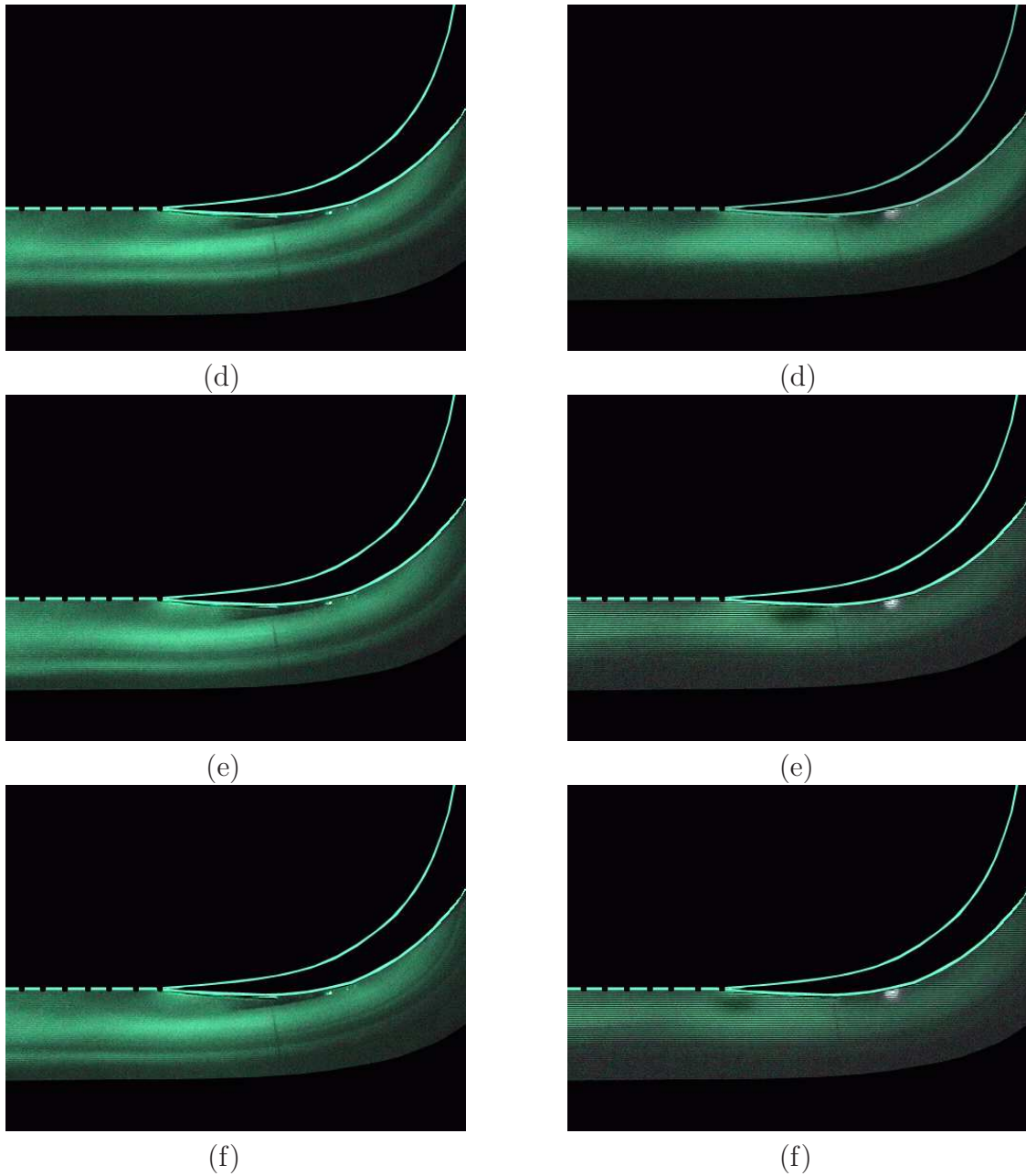
Figure 7.2 (continued). Seven consecutive frames taken from the flow videos for Re_c = 25,000 . The frames in the left column represent the flow field for the uncontrolled case. The frames in the right column represent the flow field when an unsteady plasma actuator was operated. The unsteady plasma actuator was located at x/C_x = 67.5\% and operated at 20 Hz. The actuator amplitude was 8 kV and the plasma duty cycle was 10%.
