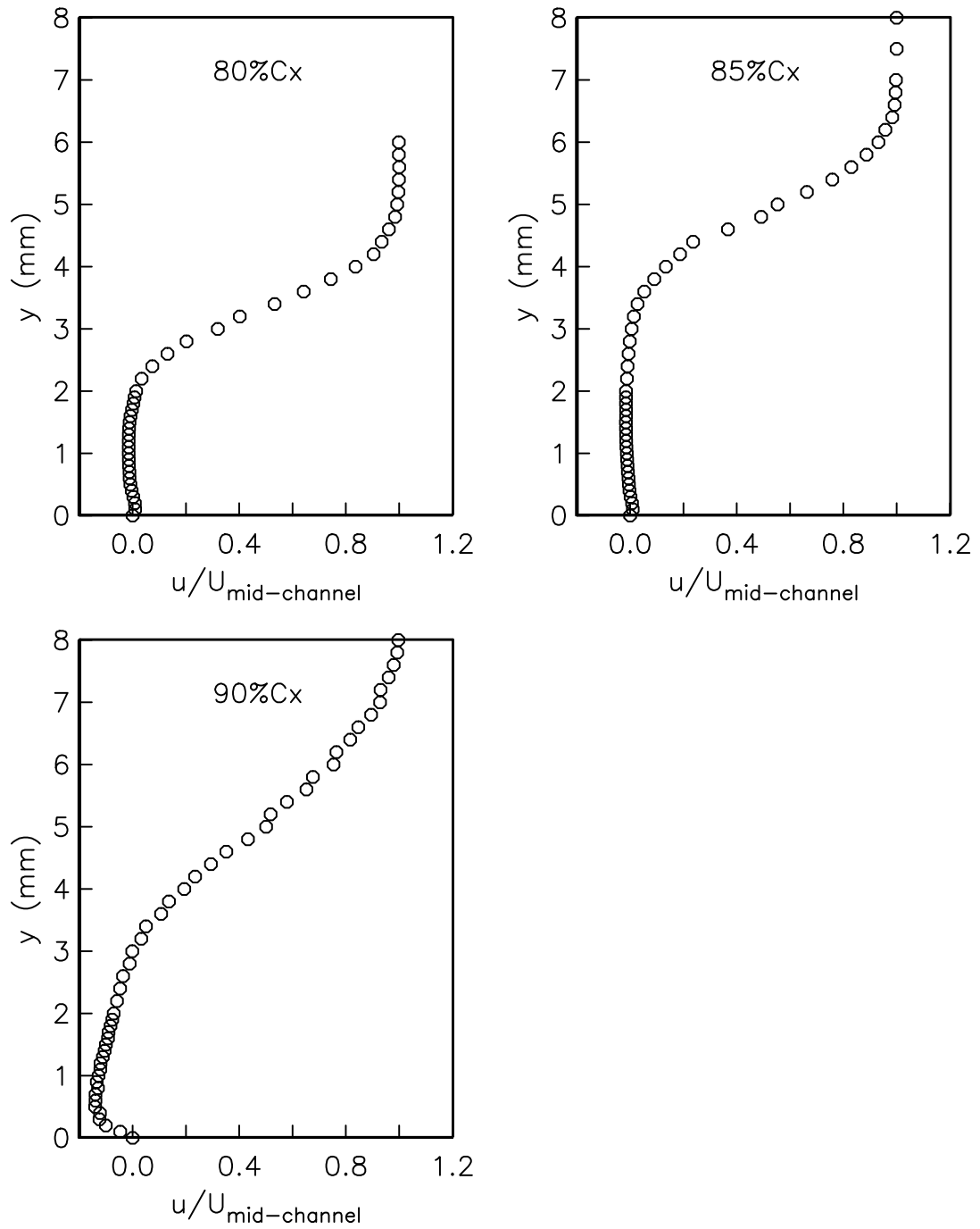
Figure 3.6 (continued). Boundary layer profiles for Re=50,000 and FSTI=0.08\% .
