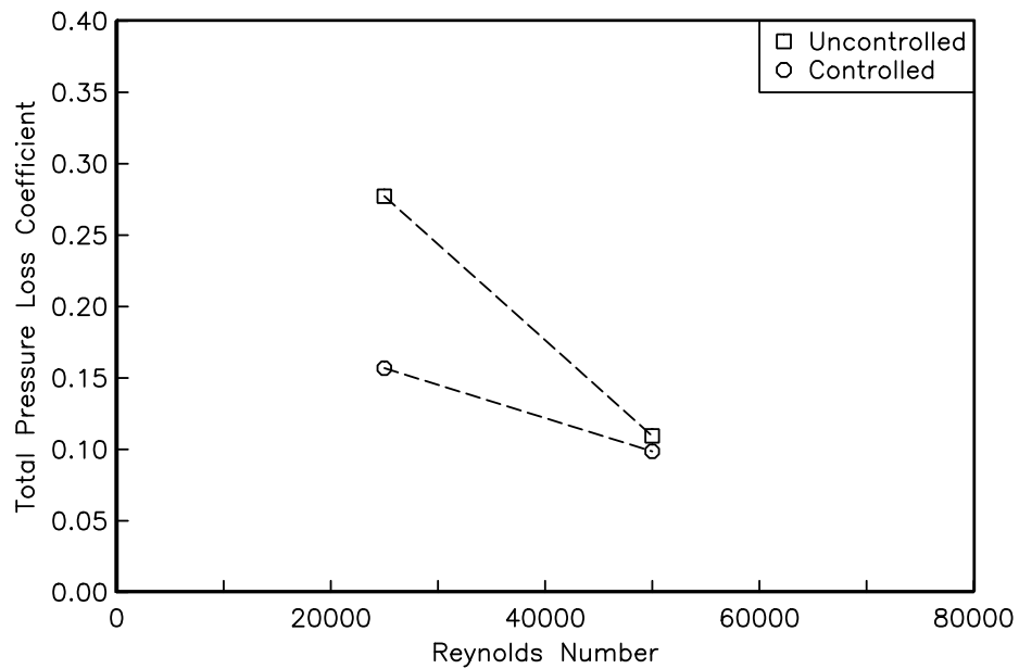
Figure 6.8. Total pressure loss coefficient calculated from the measured wake profiles for both uncontrolled and controlled cases. For controlled cases, an unsteady plasma actuator was located at x/C_x = 67.5\% . The excitation frequency was 40 Hz for Re_c = 50,000 and 20 Hz for Re_c = 25,000 . The actuator amplitude was 8 kV and the plasma duty cycle was 10% for both Reynolds numbers.
