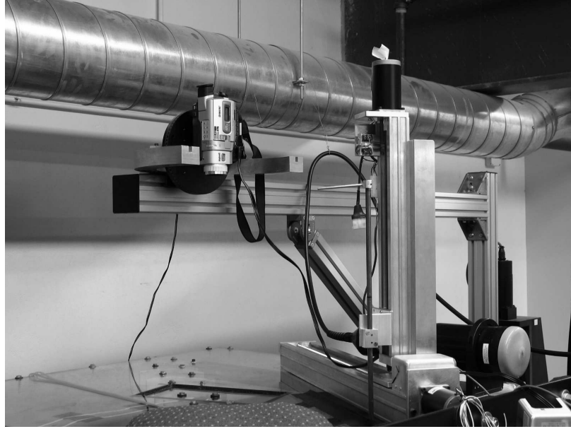
Figure 2.24. A Sony DCR-TRV740 digital camcorder was mounted on the LDV traverse beam and used to record the flow video.
