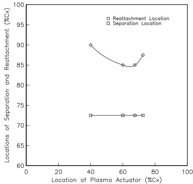
Figure 5.3. The locations of separation and reattachment as a function of the location of single steady plasma actuator. The Reynolds number was 50,000 and the amplitude of the actuator voltage level was 8 kV.
