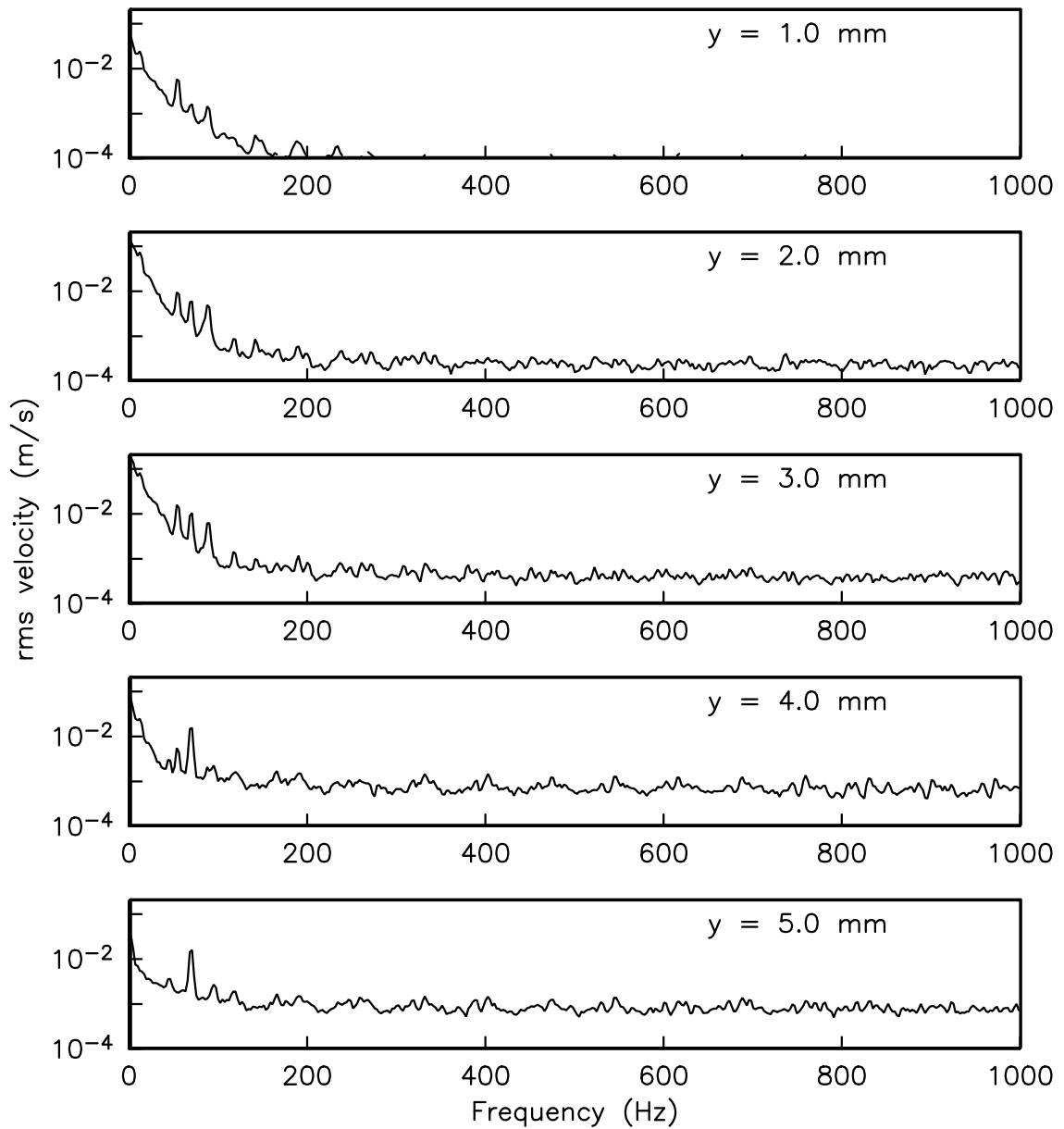
Figure 7.9. Power spectra for five wall normal distances at x/C_x = 75\% for the uncontrolled flow field at Re_c = 50,000 .
