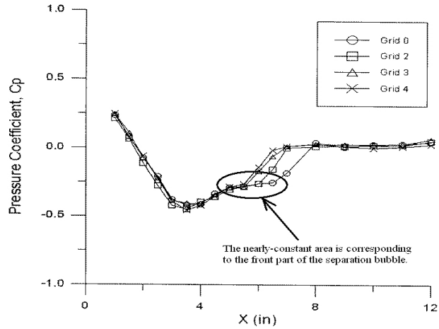
Figure 1.4. The pressure distribution over the flat plate (simulated suction surface) for Re_{ss}=70k (from Sohn [54]).
