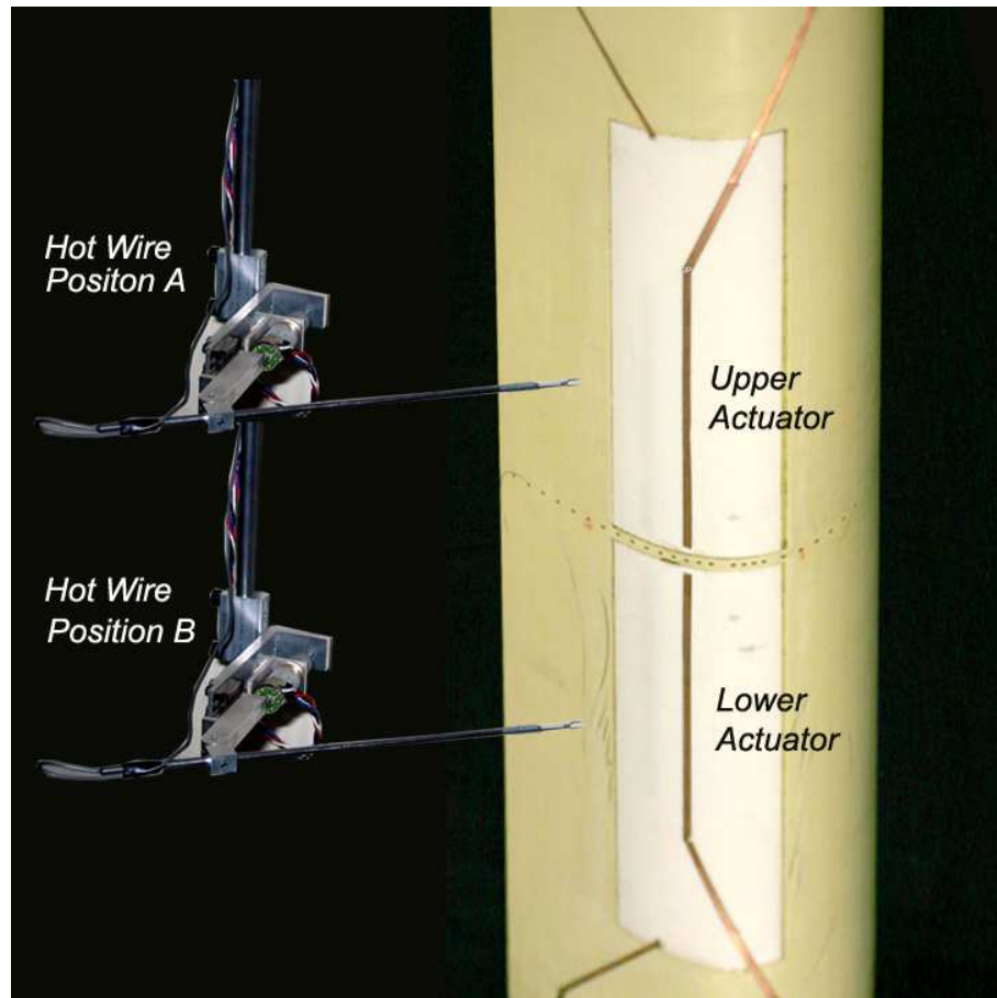
Figure 7.4. The experimental setup to check the electronic noise from plasma actuators for hot-wire measurements.
