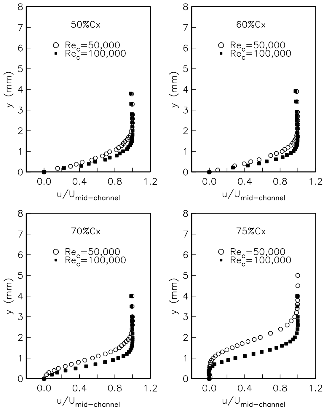
Figure 3.7. Boundary layer profiles for Re_c = 50,000 and Re_c = 100,000 for FSTI=0.08\% .
