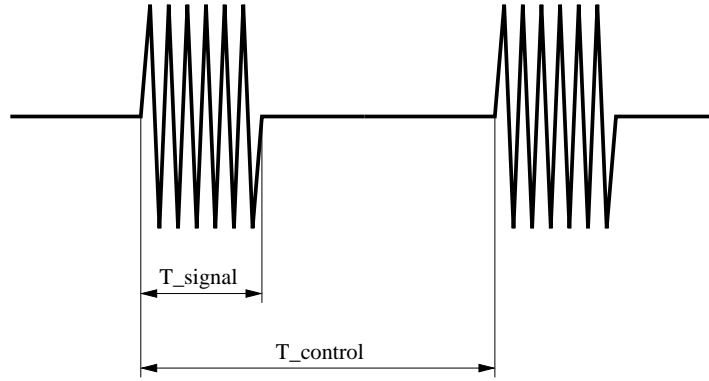
Figure 6.1. The control signal sent to the plasma actuator during unsteady excitation. T\_control is the time duration of one cycle of the control signal. T\_signal is the time duration of the high frequency, high amplitude triangular wave.
