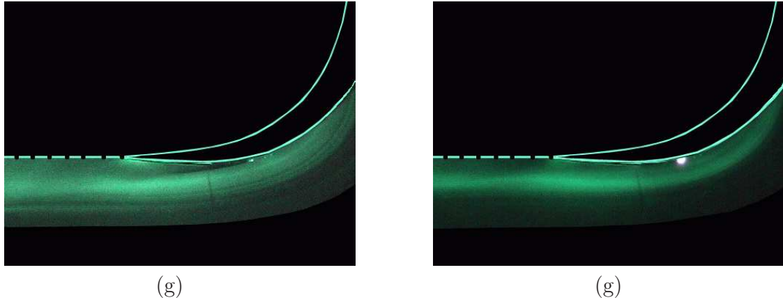
Figure 7.1 (continued). Seven consecutive frames taken from the flow videos for Re_c = 25,000 . The frames in the left column represent the flow field for the uncontrolled case. The frames in the right column represent the flow field when a steady plasma actuator was operated. The steady plasma actuator was located at x/C_x = 67.5\% . The actuator amplitude was 8 kV.
