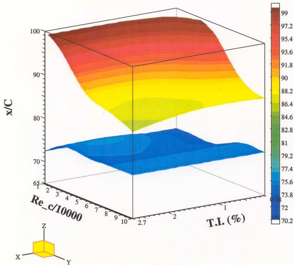
Figure 3.14. Combined effect of chord Reynolds number and freestream turbulence level on the separation (bottom surface) and reattachment (top surface) locations on the suction side of the “PakB” blade.
