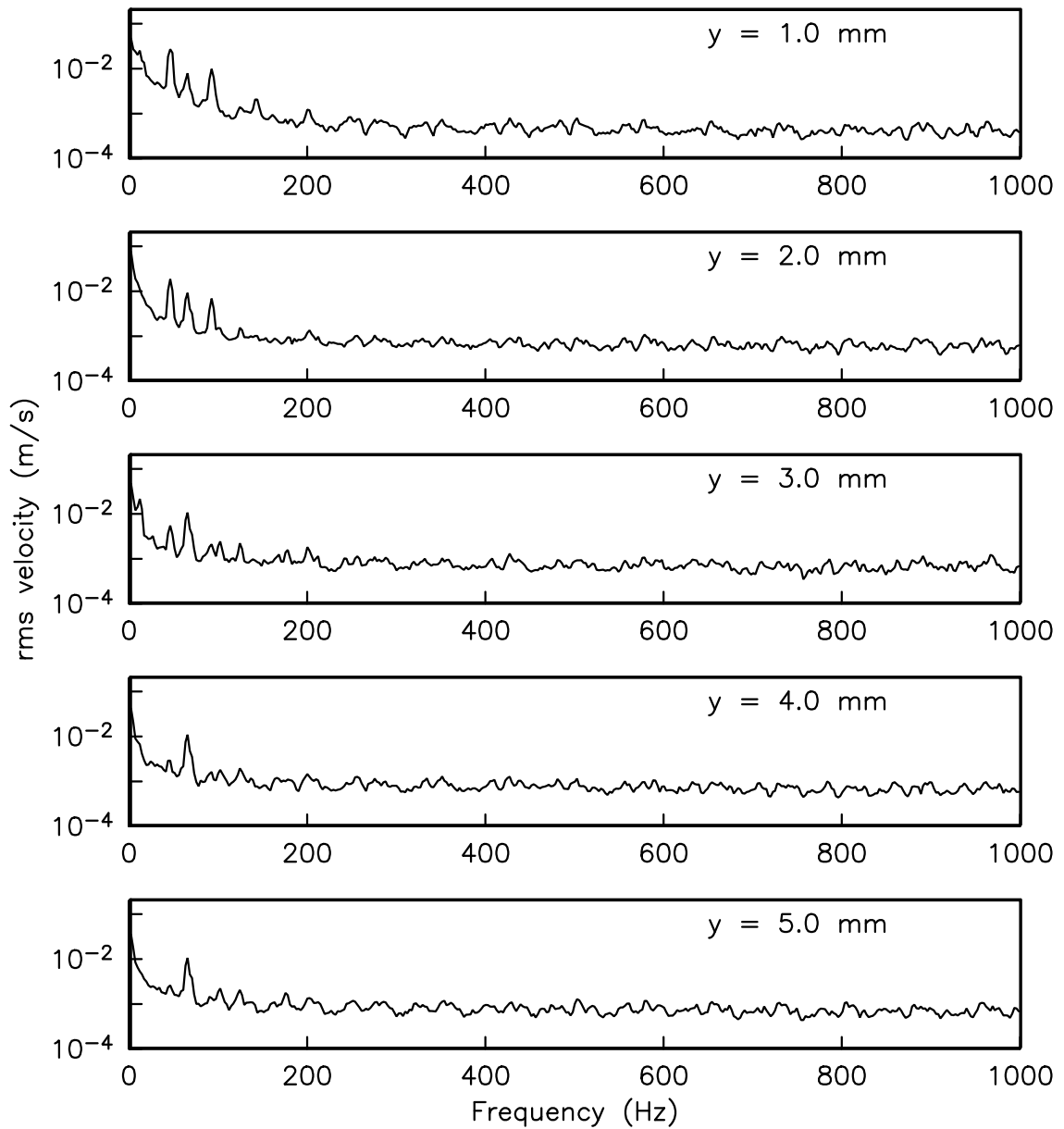
Figure 7.8. Power spectra for five wall normal distances at x/C_x = 70\% for the uncontrolled flow field at Re_c = 50,000 .
