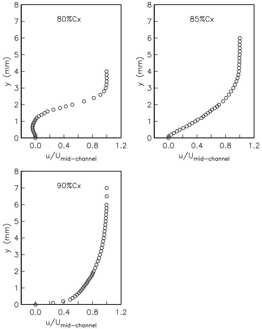
Figure 3.4 (continued). Boundary layer profiles for Re=100,000 and FSTI=0.08%.
