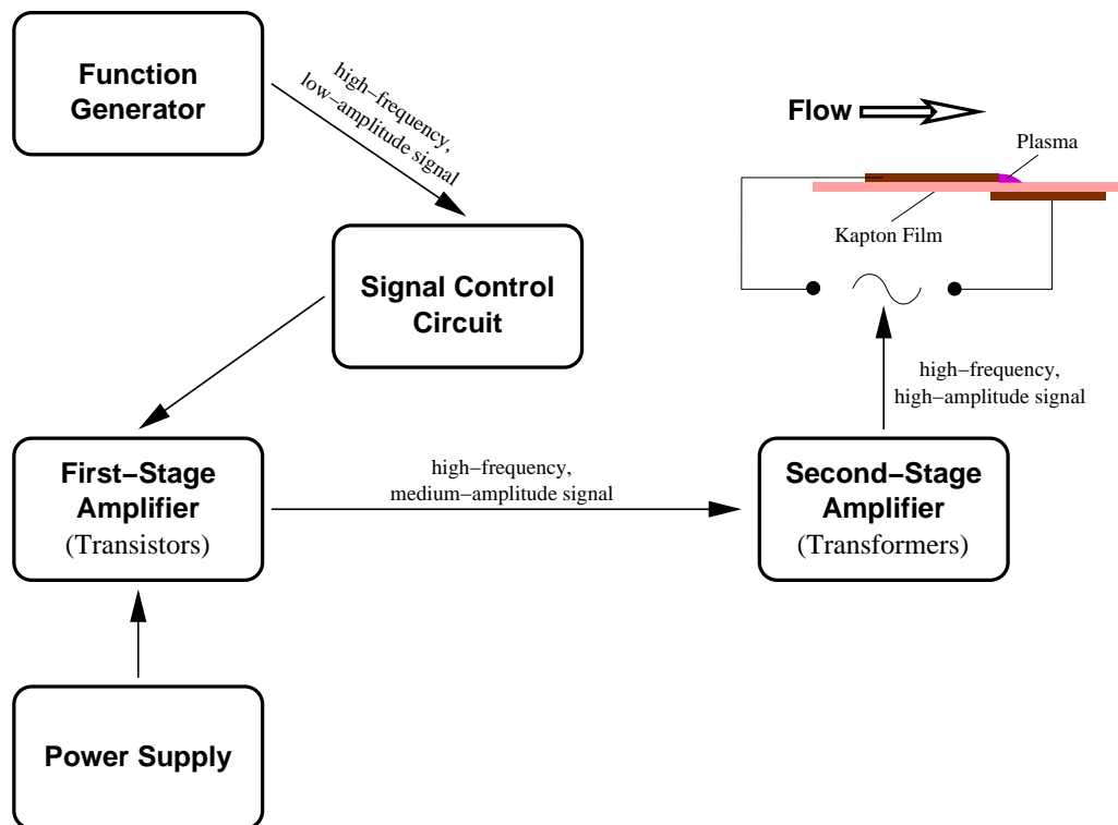
Figure 2.20. A specially-designed circuit was used to generate high a.c. voltage.
