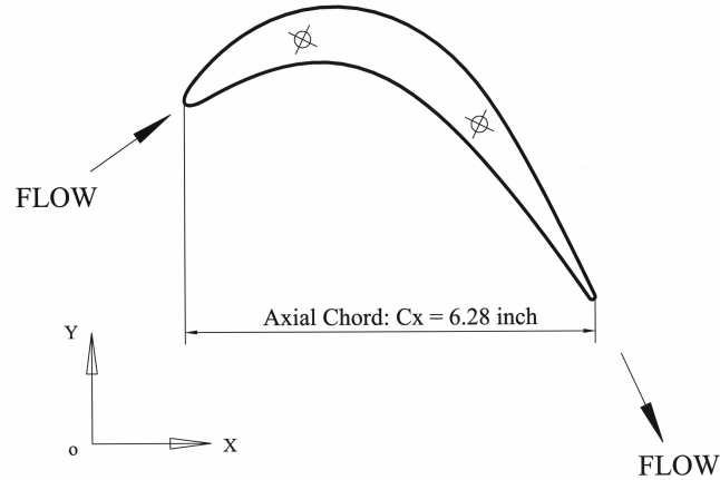
Figure 2.3. The “PakB” blade has an axial chord length of 6.28 in (15.95 cm).
