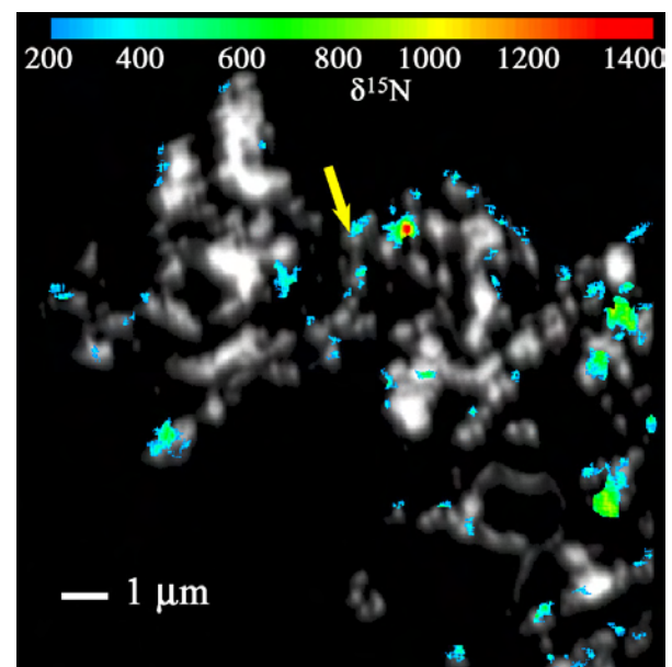
Fig. 2: This image shows regions of IDP L2036 AA7 with \delta^{15}\text{N} values larger than +200 ‰ overlain on the ^{16}\text{O} image of the sample. The location of the presolar silicate candidate grain is indicated by the arrow.
