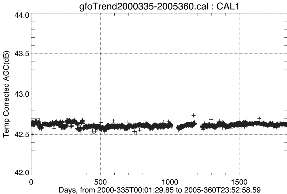
Figure 2-2 CAL-1 AGC for the First 109 Cycles
