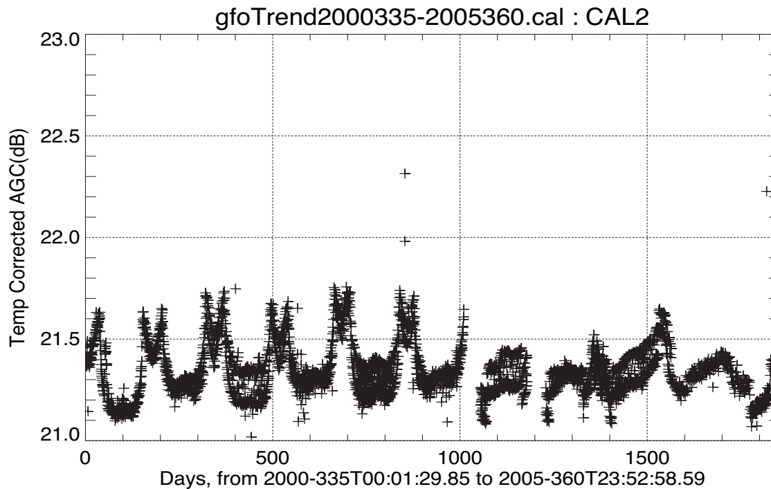
Figure 2-3 CAL-1 AGC for the First 109 Cycles
