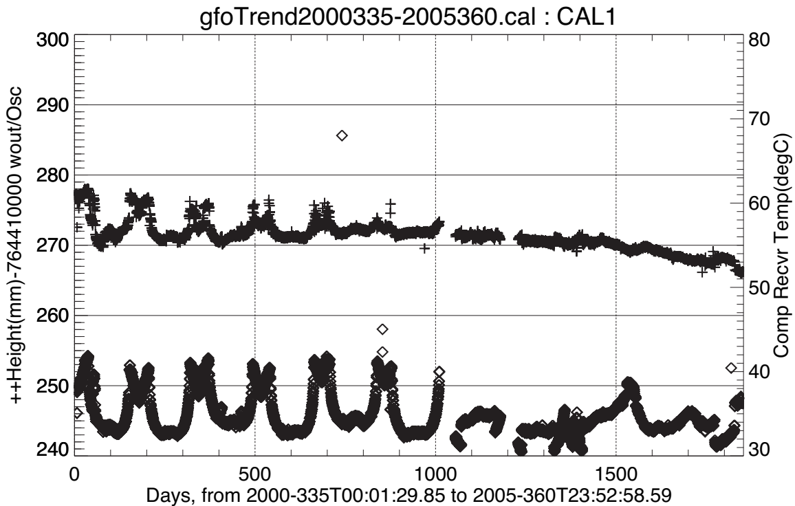
Figure 2-1 CAL-1 Range/Temperatures for the First 109 Cycles
