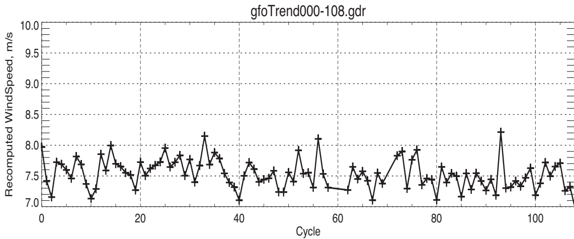
Figure 2-14 Cycle-Averages Recomputed Windspeed in Meters Per Second
