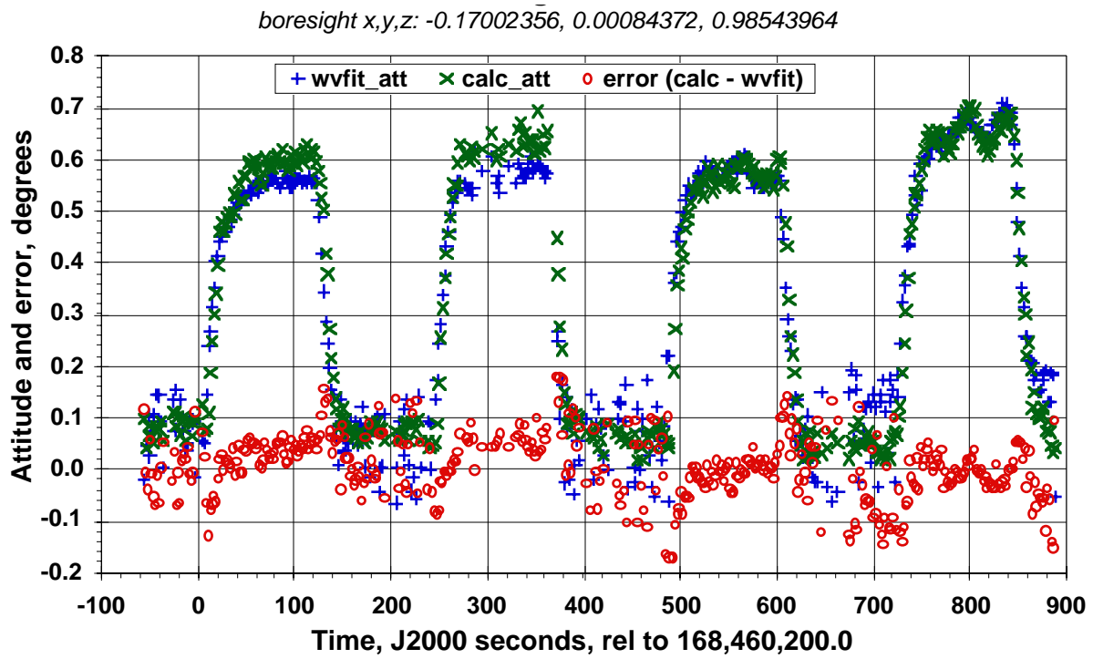
Figure 4-5 Waveform Fit and Calculated Attitudes in 2005/05/04 ABCAL from WFF Boresight Vector Solution
