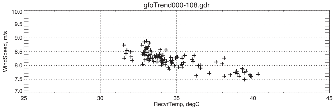
Figure 2-11 Cycle-Averages Windspeed vs. Temperature
