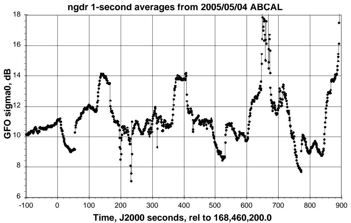
Figure 4-4 GFO NGDR Sigma0 Estimates
