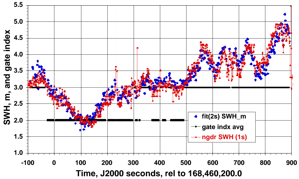
Figure 4-3 GFO SWH Estimates and Gate Index Values in 2005/05/04 ABCAL
