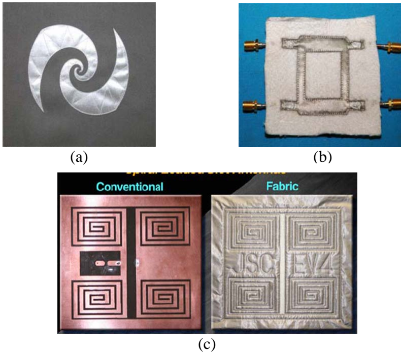
Figure 1(a) E-textile equiangular spiral. (b) Quadrature hybrid. (c) Miniaturized spiral-loaded slot antenna.
