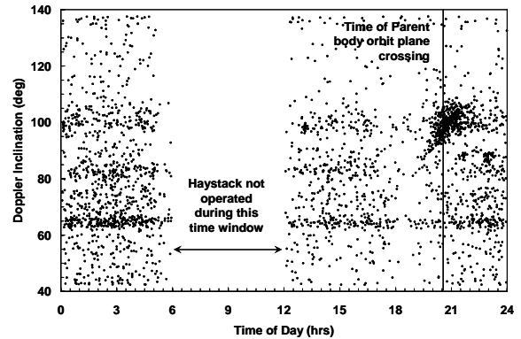
Fig. 7. Haystack staring data collected from January to May, 2007. Many of the detections near 100^\circ inclination and 2100 hrs are Fengyun-1C debris.
