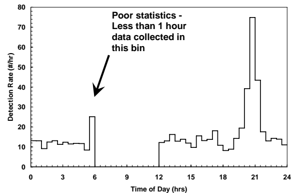
Fig. 8. Diurnal detection rate for the Haystack 75^\circ East staring data shown in Figure 7. The peak detection rate corresponding to passage of the Fengyun-1C cloud through the radar beam is 6 times higher than the background rate of 12.4 detections per hour.
