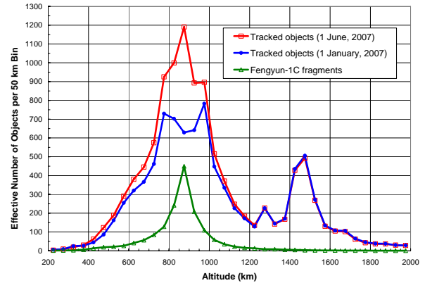
Fig. 9. Distribution of Fengyun-1C debris and effect on the LEO population.
