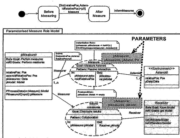
Figure 5. Parameterized role model of Measure
