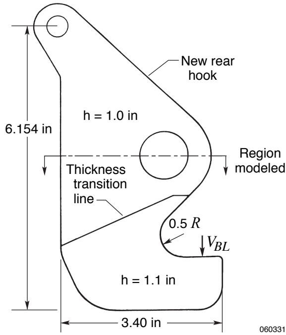
Figure 7. Geometry of the B-52B pylon rear hook.
