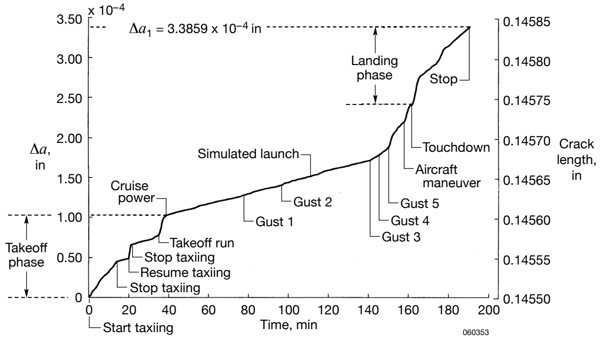
Figure 29. Crack growth curve for the Pegasus pylon front right hook (VPFR); B-52B carrying the Hyper-X launching vehicle; captive flight.
