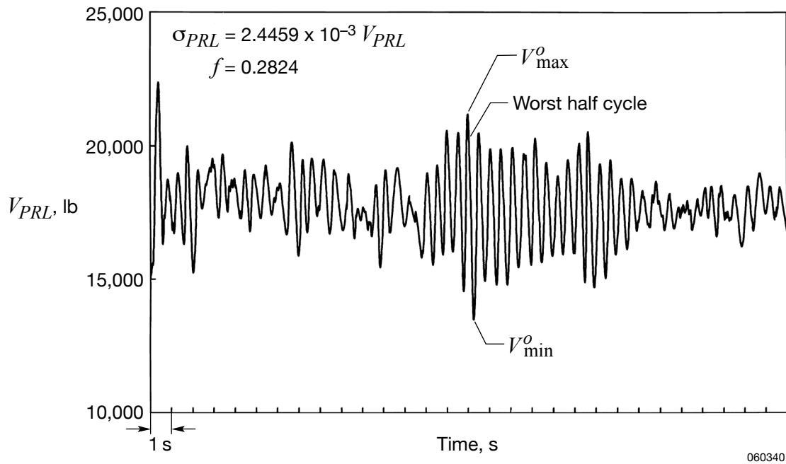
Figure 16. Loading spectrum of the Pegasus pylon rear left hook (VPRL) carrying Hyper-X launching vehicle during takeoff.
