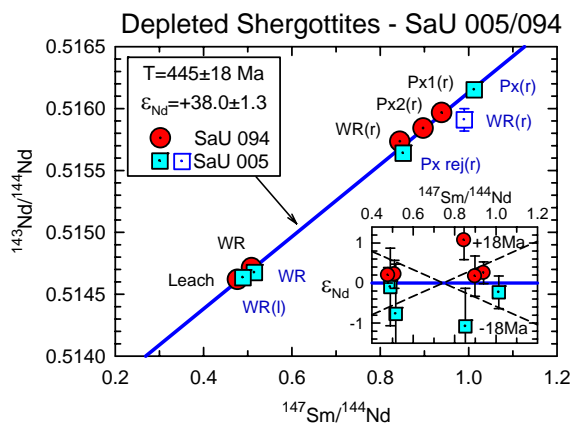
Figure 2. Sm-Nd data of SaU 005/094.
