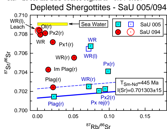
Figure 1. Rb-Sr data of SaU 005/094.
