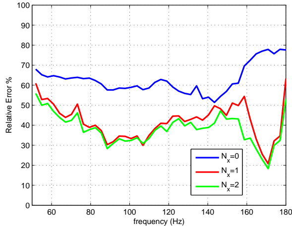
Figure 4: Patch ESM with \delta = 0.08m reconstruction for different frequencies using extension points N_x .
