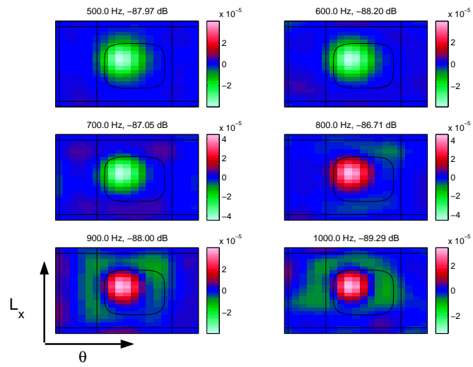
Figure 7: Normal Velocity reconstruction using patch ESM with extension points N_x = 2 and \delta = 0.0254m for some selected frequencies.
