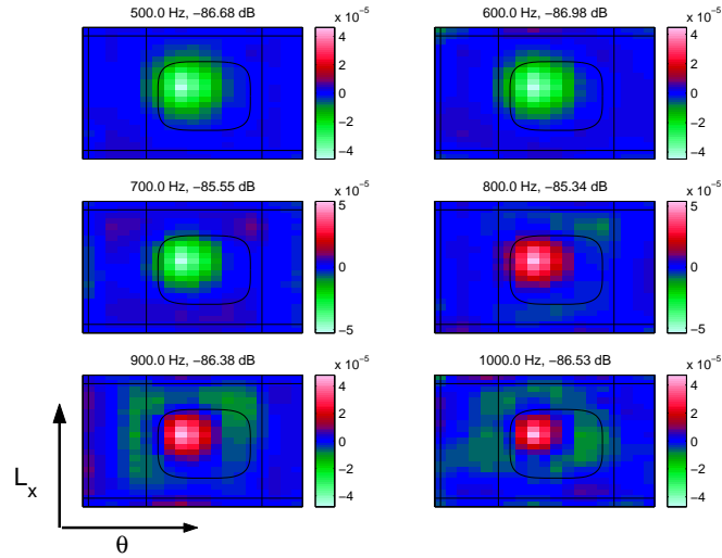
Figure 6: Normal Velocity reconstruction using patch IBEM with extension points N_x = 2 for some selected frequencies.
