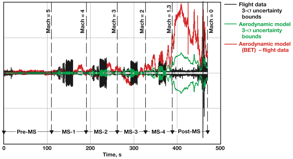
Figure E-09. Yawing moment differential relative to 3-σ uncertainties.
