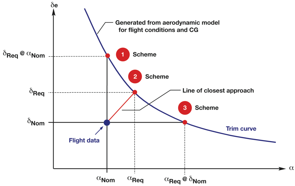
Figure 6. Pitching moment matching schemes.
