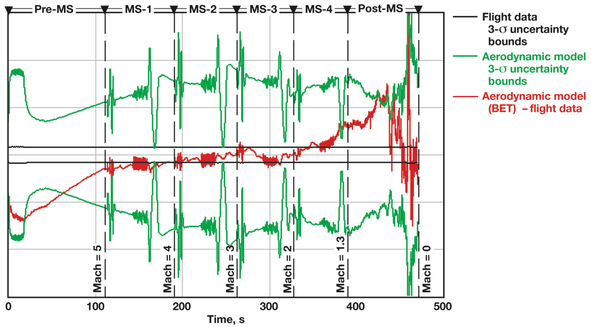
Figure B-08. Normal force differential relative to 3\text{-}\sigma uncertainties.
