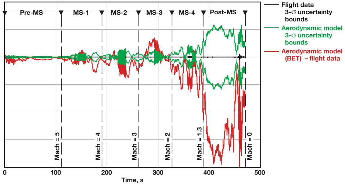
Figure E-06. Rolling moment differential relative to 3- \sigma uncertainties.
