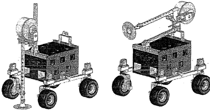
Figure 13. MUM deployed on K10 rover (left), MUM stowed for driving (right). (Image credit: Khoa Nguyen)
