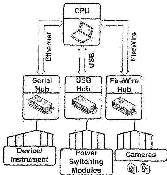
Figure 5. Communications System Block Diagram.
