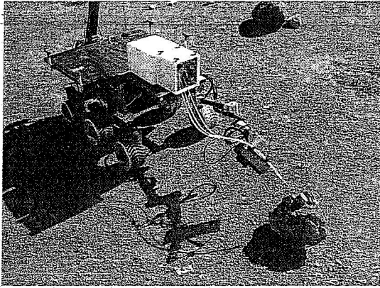
Figure 10. K9 extends the CMAD remote sensor.
