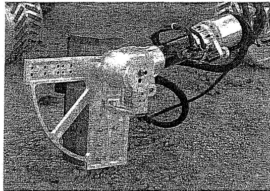
Figure 7. Instrument Palette.
