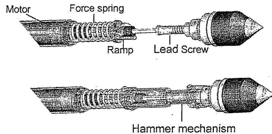
Figure 11. Internal view of MUM showing hammering mechanism. (Image credit: Khoa Nguyen)
