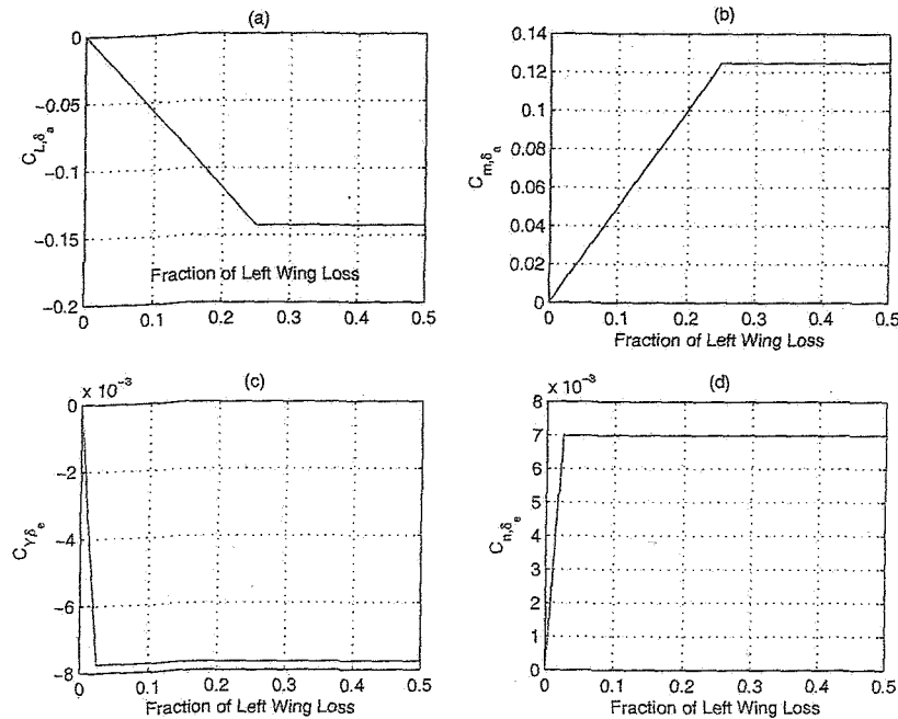
Fig. 3 - Control Derivatives Due to Wing Loss at \alpha = 12^\circ and \beta = 0^\circ
