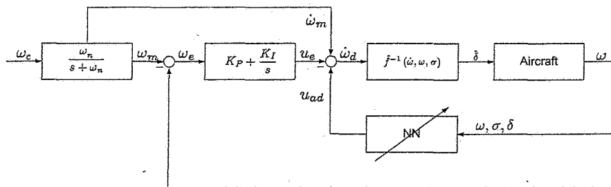
Fig. 6 - Direct Neural Network Adaptive Flight Control Architecture
