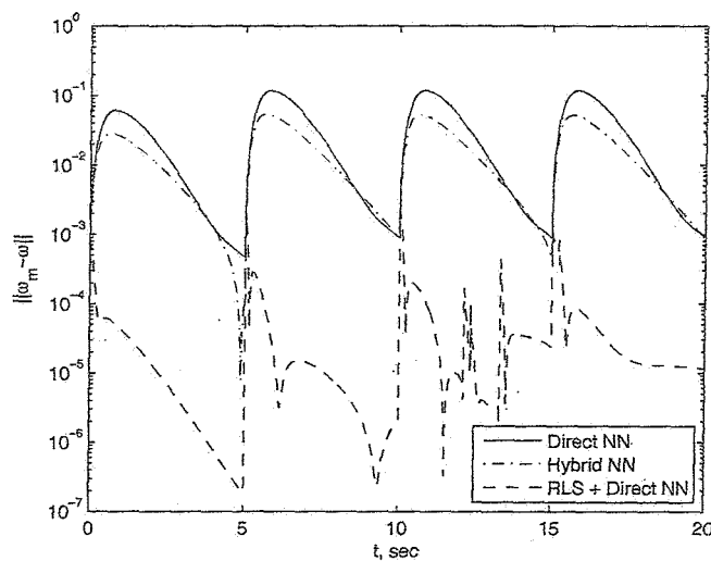
Fig. 12 - Tracking Error Norm
