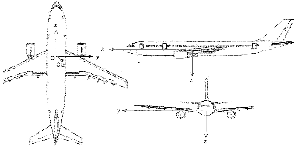
Fig. 4 - C.G. Shift Relative to Reference Point O
