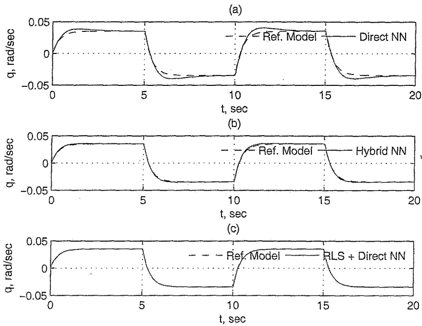
Fig. 11 - Pitch Doublet Tracking Performance
