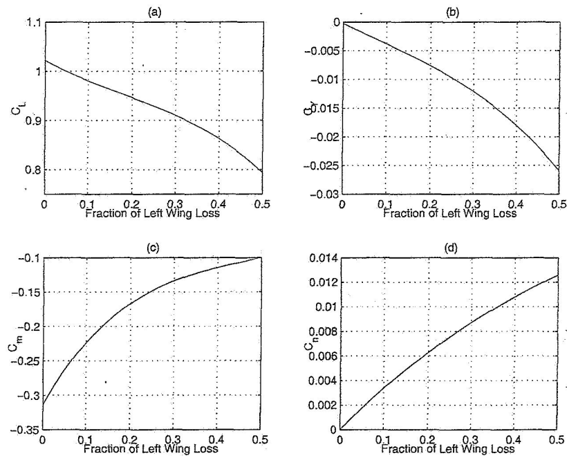
Fig. 2 - Aerodynamic Coefficients Due to Wing Loss at \alpha = 12^\circ and \beta = 0^\circ
