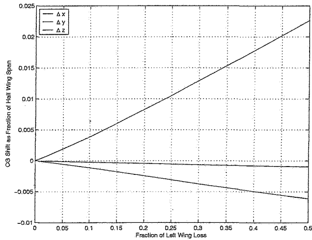
Fig. 5 - C.G. Shift due to Wing Loss
