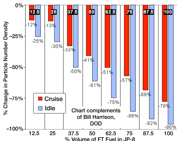
Figure 15.—Reduction of exhaust emission particulates has been found when using FT fuel blended in JP-8 9 (ref. 2).
