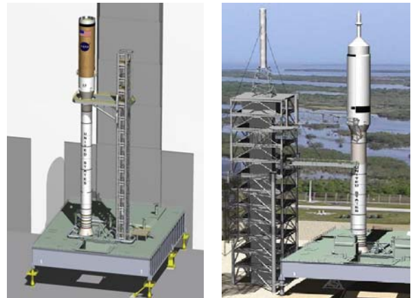
Figure 11. Depiction of vehicle stacking and operations at NASA Kennedy Space Center.
