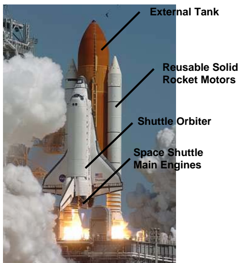
Figure 7. Components of the Space Shuttle System.
