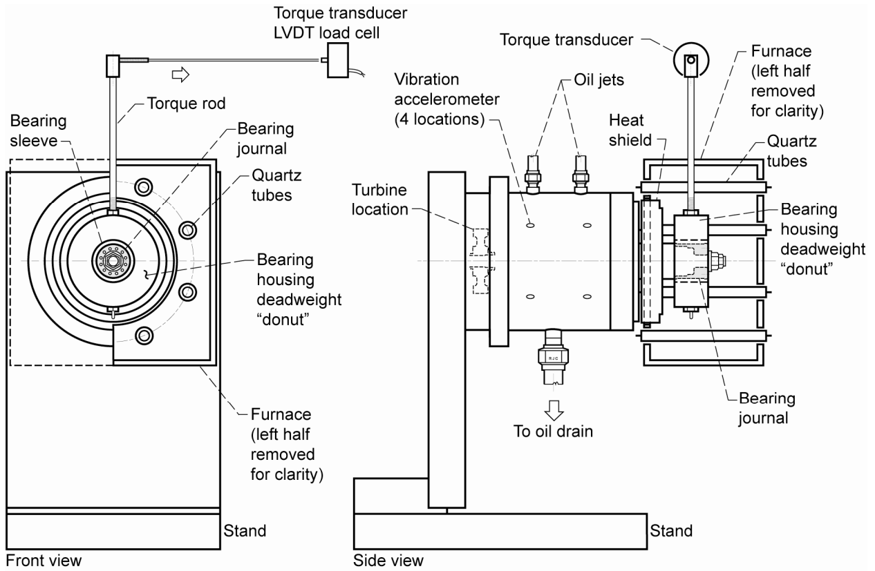
Figure 6. —Schematic view of high-temperature, high-speed foil bearing test rig used to measure bearing power loss.
