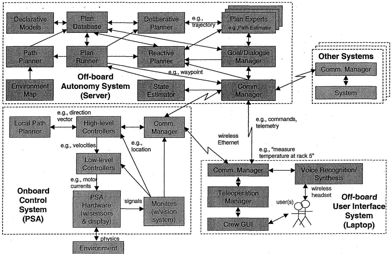
Figure 4 - PSA Autonomy Framework
