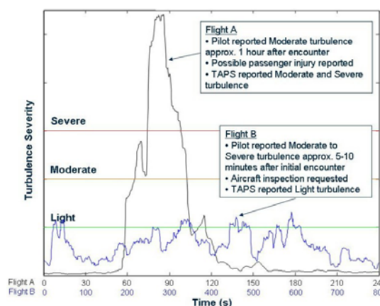
Fig. 8. Two Comparisons of PIREPs vs. TAPS
