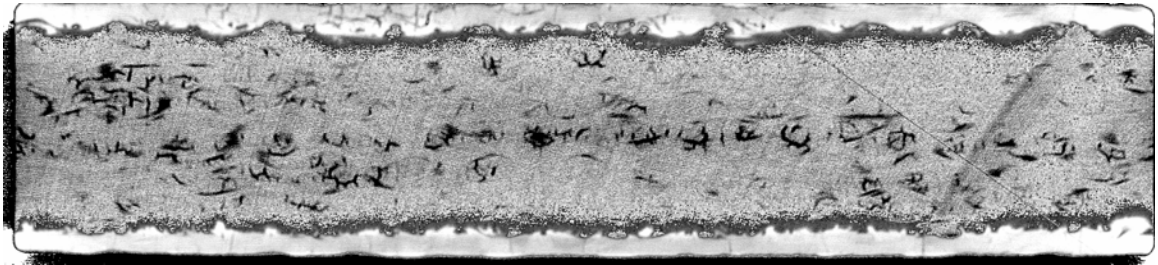
Figure 11. Next sequential 100 micron slice of flex-5 near center of specimen.
