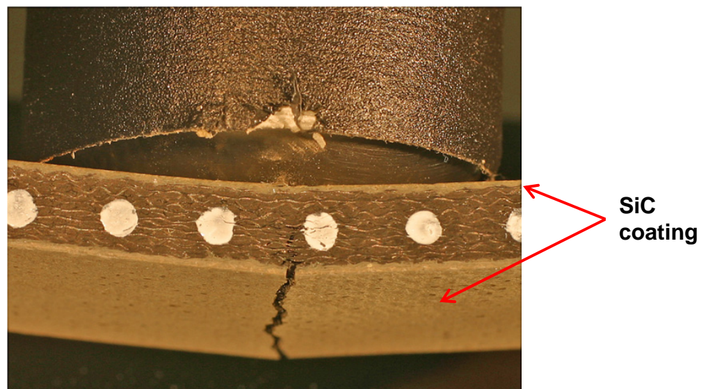
Figure 7. Typical failure of bend specimen. Dots were used for photogrammetry.
