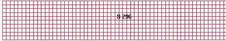
Figure 15. Simple 3-point specimen discretization
