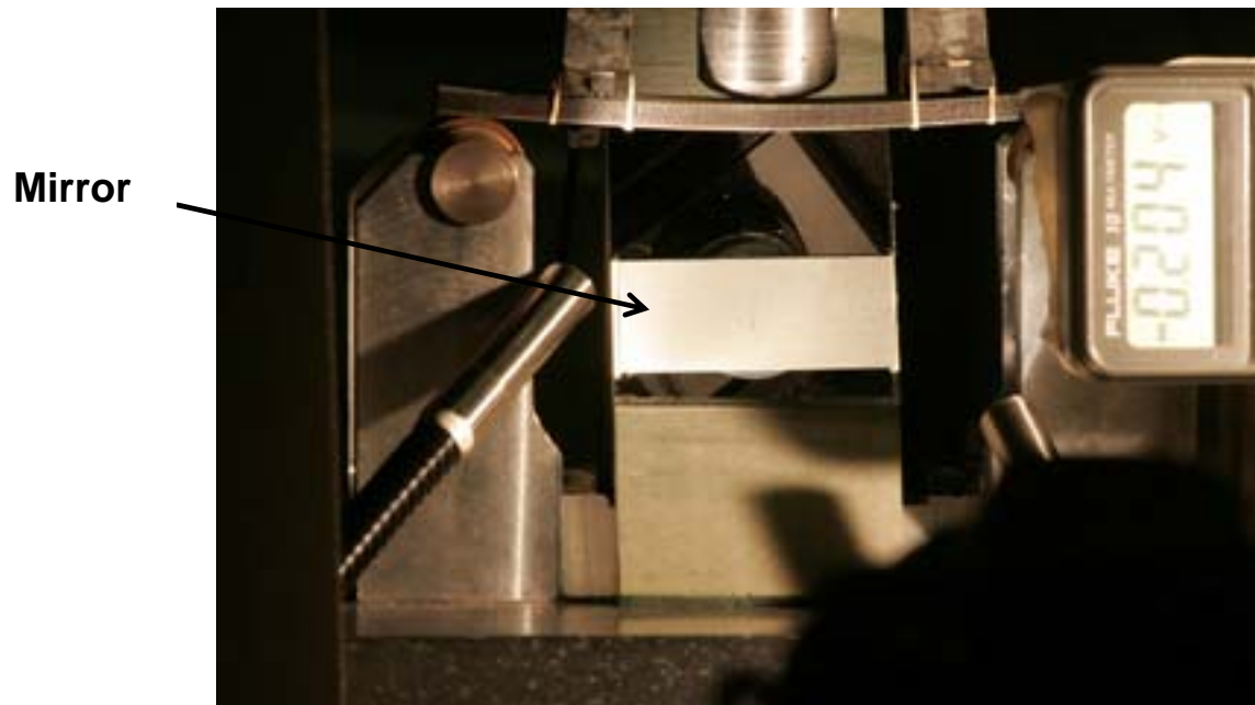
Figure 6. 3-Point bend test with mirror to view the crack growth in the lower layer of SiC with a digital camera.
