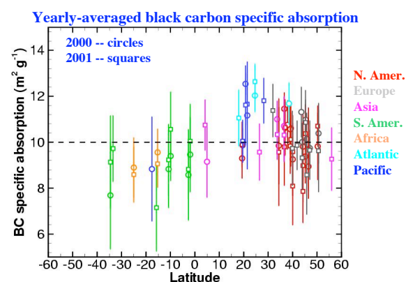
Figure 2: Yearly averaged black carbon specific absorption ( \lambda = 0.55 \mu\text{m} ) corresponding to 46 AERONET sites. Circles represent the year 2000, squares the year 2001, and whiskers indicate the standard deviations.
