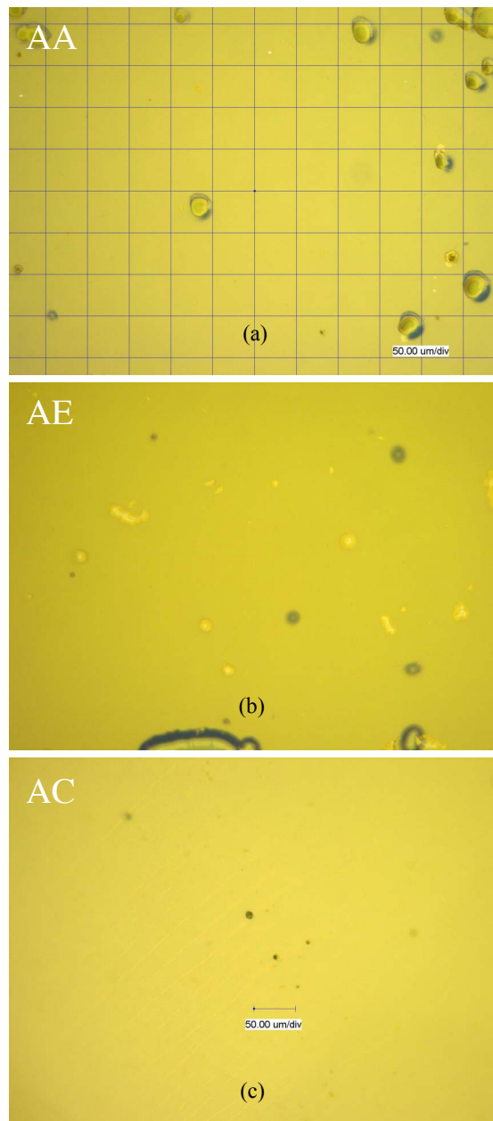
Figure 6.—Typical undercutting densities for various AO exposures: (a) asher followed by in-space, (b) asher, and (c) in-space.
