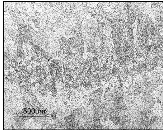
Figure 7. Small equiaxed grains at interlayer boundaries in as-deposited Al 2219.
