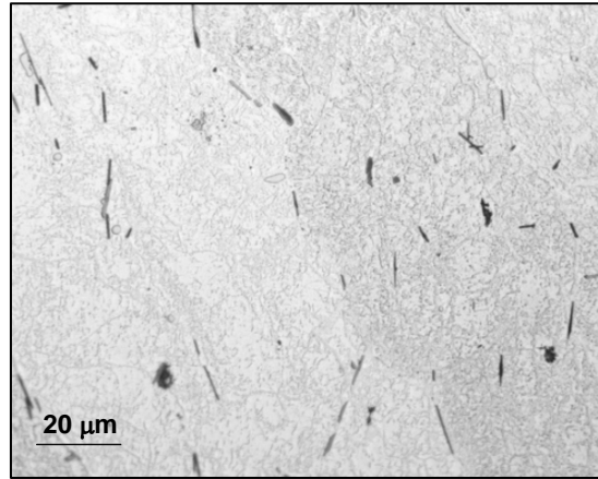
Figure 11. Transformed internal dendritic structure following T6 heat treatment.
