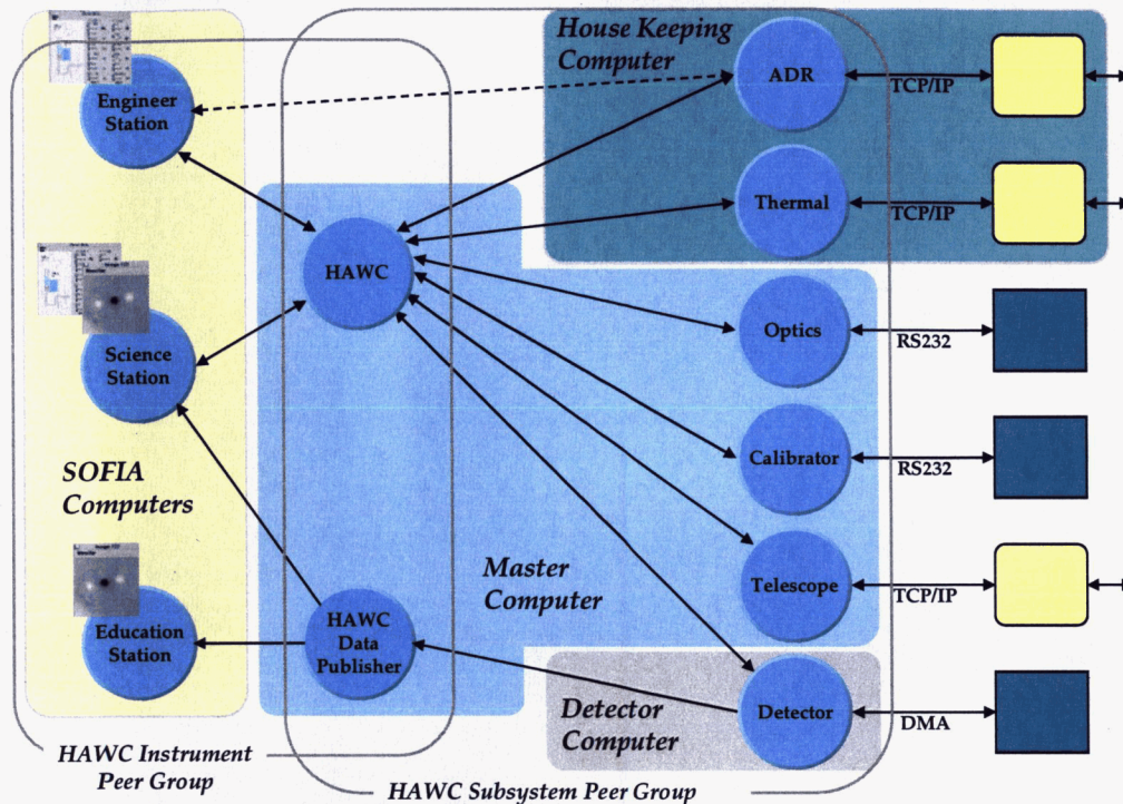
Figure 9. HAWC IRC Device Architecture.
