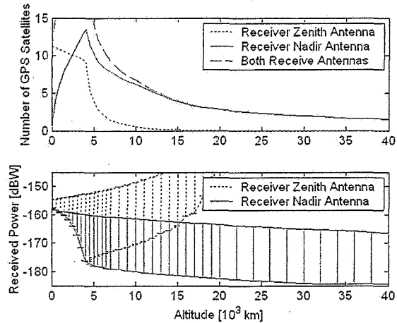
Figure B: (Top) Number of GPS satellites visible and (Bottom) received power broken out between zenith and nadir receiving antennas as a function of altitude. Assumes L1 C/A signals from a Block IIA GPS earth coverage antenna with a 23.5° beamwidth (side lobe signals excluded).
