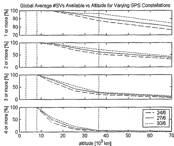
Figure J: Global average of GPS availability as a function of altitude for the 24/6, 27/6, and 30/6 satellite constellations.
