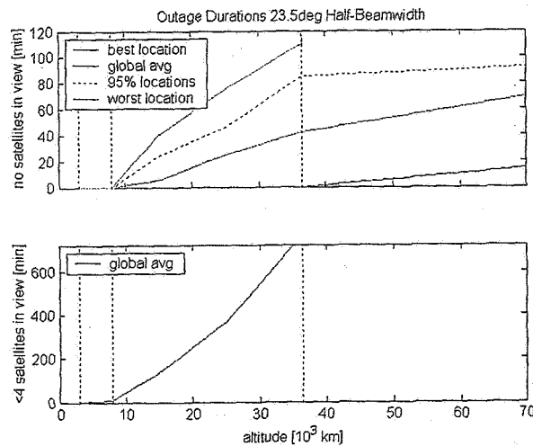
Figure H: Outage durations for 23.5° half-beamwidth.
