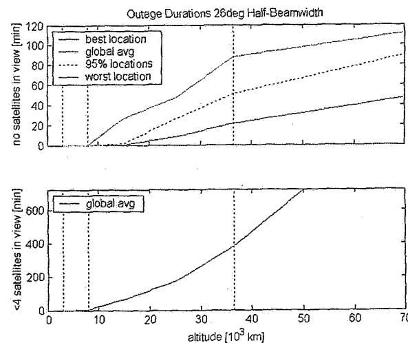
Figure I: Outage durations for 26.0° half-beamwidth.
