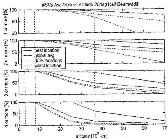
Figure G: GPS availability as a function of altitude for 26.0° half-beamwidth.
