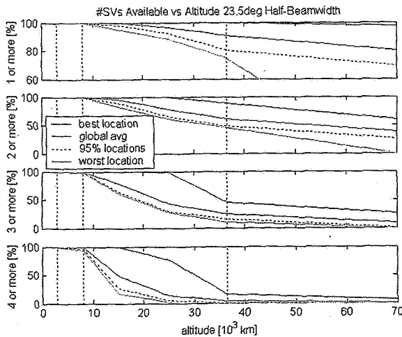
Figure F: GPS availability as a function of altitude for 23.5° half-beamwidth.
