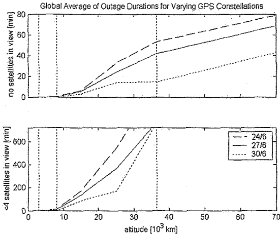
Figure K: The global average of the longest outages as a function of altitude for the 24/6, 27/6, and 30/6 satellite constellations (in six orbital planes). Simply adding three satellites to the six-plane GPS constellation significantly decreases the longest outage duration for users above the GPS constellation.
