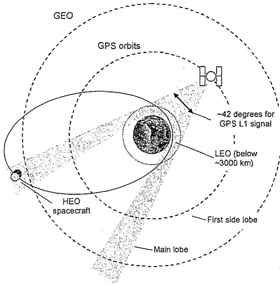
Figure A: Geometry for reception of GPS signals by a HEO spacecraft.
