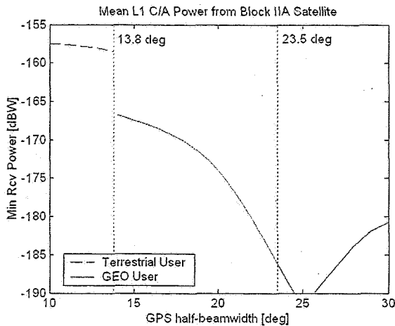
Figure D: Illustration of minimum received power levels as a function of transmitter half-beamwidth angle assuming Block IIA gain pattern [14]
